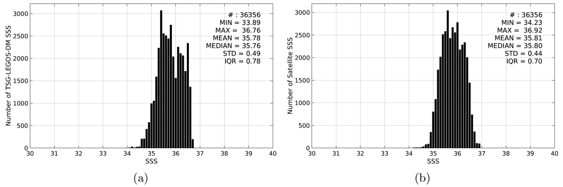
Figure 2: Histograms of SSS from TSG-LEGOS-DM (a) and SMOS-L3-CATDS-IFREMER-CECOS-V2-MONTHLY-0.25DEG (b) considering all match-up pairs per bins of 0.1 over the OTT zone Pi-MEP region and for the full satellite product period.
