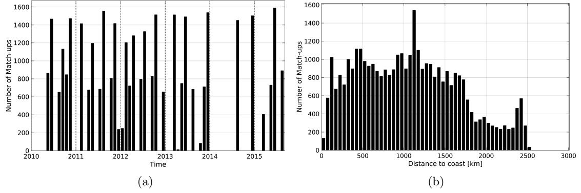
Figure 1: Number of match-ups between TSG-LEGOS-DM and SMOS-L3-CATDS-IFREMER-CECOS-V2-MONTHLY-0.25DEG SSS as a function of time (a) and as function of the distance to coast (b) over the OTT zone Pi-MEP region and for the full satellite product period.
