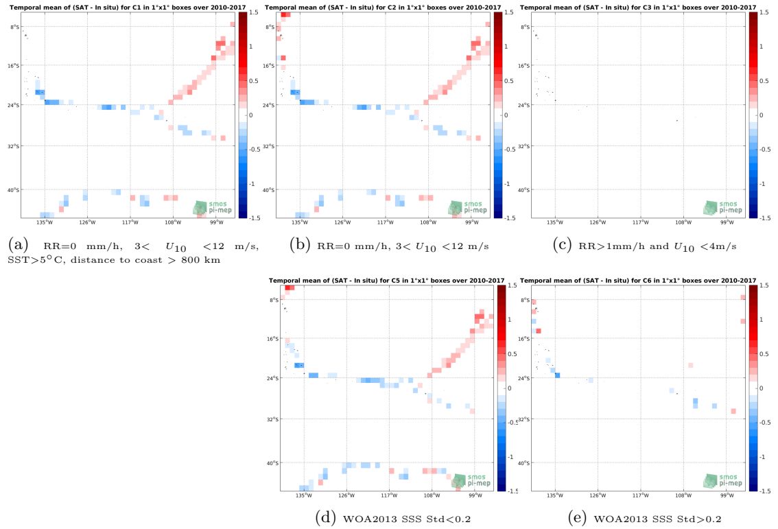
Figure 12: Temporal mean gridded over spatial boxes of size 1^\circ \times 1^\circ of \Delta SSS (SMOS-L3-CATDS-IFREMER-CECOS-V2-MONTHLY-0.25DEG - TSG-GOSUD-Sailing-ship) for 5 different sub-datasets corresponding to: RR=0 mm/h, 3 < U_{10} < 12 m/s, SST > 5^\circ C , distance to coast > 800 km (a), RR=0 mm/h, 3 < U_{10} < 12 m/s (b), RR > 1 mm/h and U_{10} < 4 m/s (c), WOA2013 SSS Std < 0.2 (d), WOA2013 SSS Std > 0.2 (e).
