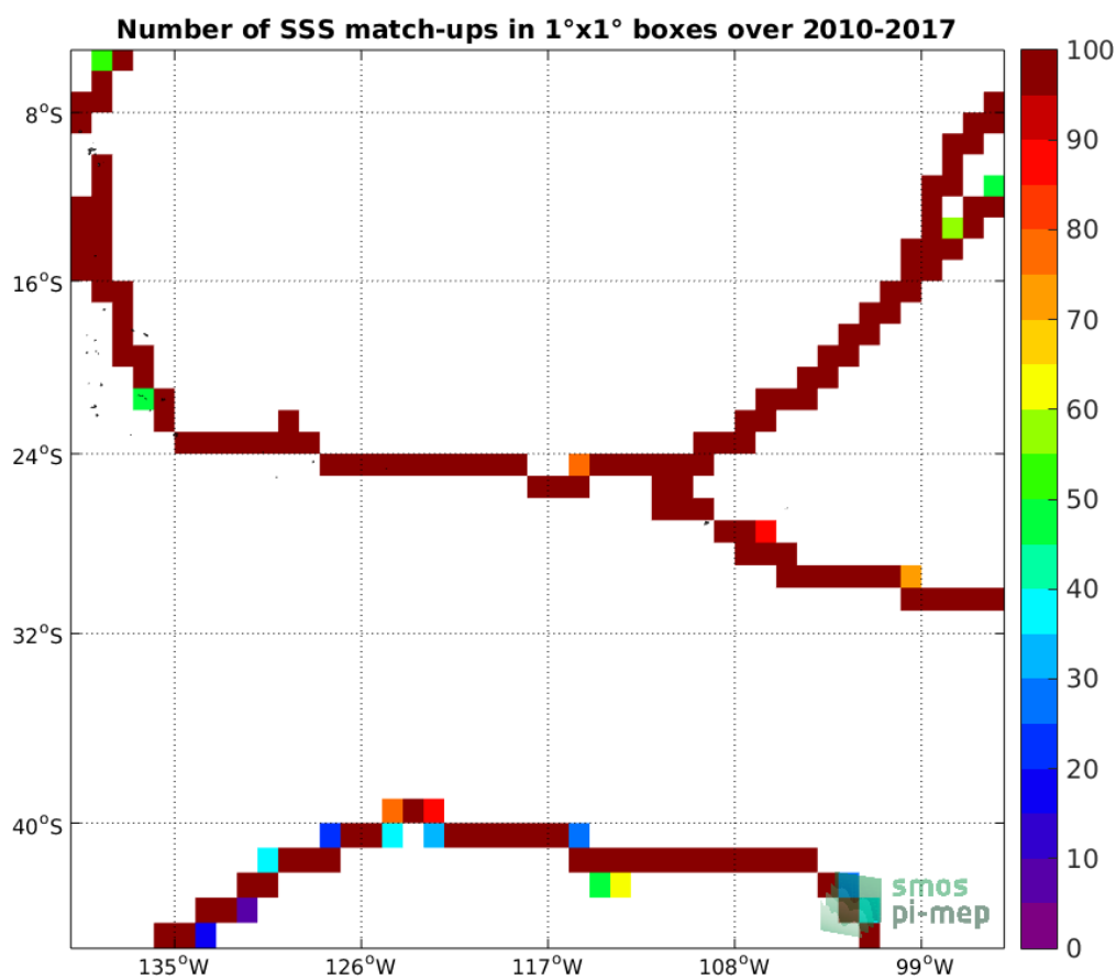
Figure 4: Number of SSS match-ups between TSG-GOSUD-Sailing-ship SSS and the SMOS-L3-CATDS-IFREMER-CECOS-V2-MONTHLY-0.25DEG SSS product for the OTT zone Pi-MEP region over 1°x1° boxes and for the full satellite product period.
