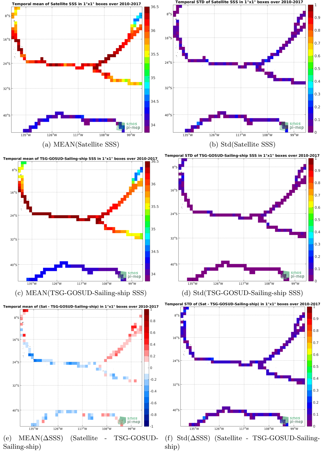
Figure 6: Temporal mean (left) and Std (right) of SSS from SMOS-L3-CATDS-IFREMER-CECOS-V2-MONTHLY-0.25DEG (top), TSG-GOSUD-Sailing-ship (middle), and of \Delta SSS (Satellite - TSG-GOSUD-Sailing-ship). Only match-up pairs are used to generate these maps.
