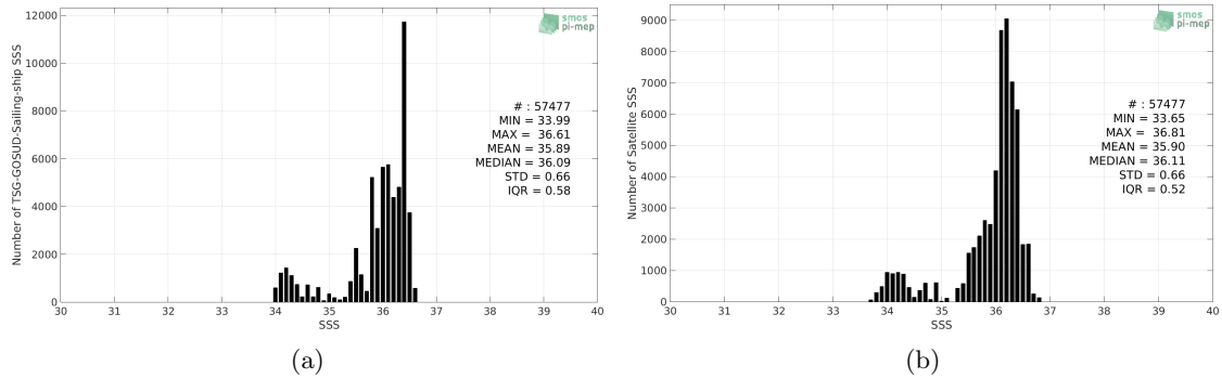
Figure 2: Histograms of SSS from TSG-GOSUD-Sailing-ship (a) and SMOS-L3-CATDS-IFREMER-CECOS-V2-MONTHLY-0.25DEG (b) considering all match-up pairs per bins of 0.1 over the OTT zone Pi-MEP region and for the full satellite product period.
