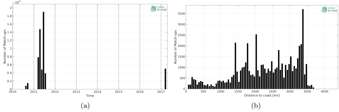
Figure 1: Number of match-ups between TSG-GOSUD-Sailing-ship and SMOS-L3-CATDS-IFREMER-CECOS-V2-MONTHLY-0.25DEG SSS as a function of time (a) and as function of the distance to coast (b) over the OTT zone Pi-MEP region and for the full satellite product period.
