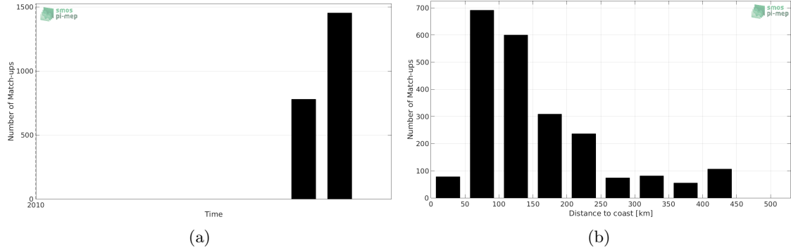
Figure 1: Number of match-ups between TSG-GOSUD-Sailing-ship and SMOS-L3-CATDS-IFREMER-CECOS-V2-MONTHLY-0.25DEG SSS as a function of time (a) and as function of the distance to coast (b) over the OTT zone Pi-MEP region and for the full satellite product period.
