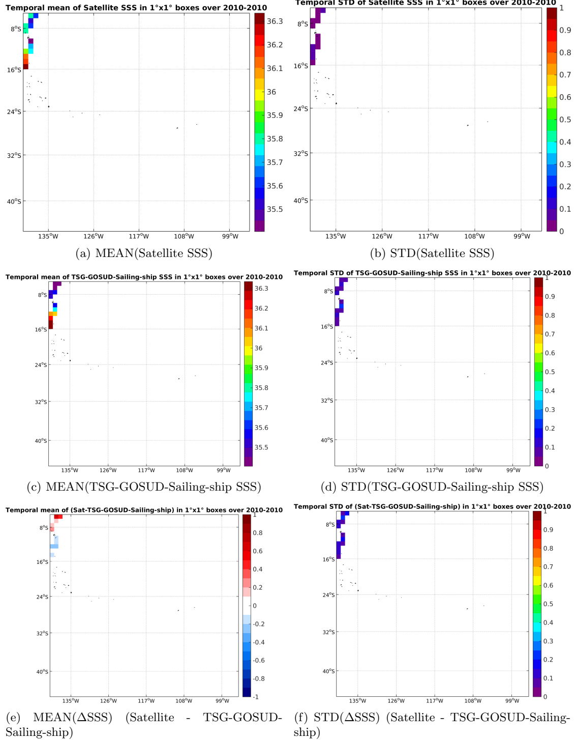
Figure 6: Temporal mean (left) and STD (right) of SSS from SMOS-L3-CATDS-IFREMER-CECOS-V2-MONTHLY-0.25DEG (top), TSG-GOSUD-Sailing-ship (middle), and of \Delta SSS (Satellite - TSG-GOSUD-Sailing-ship). Only match-up pairs are used to generate these maps.
