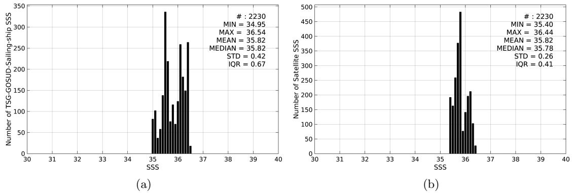
Figure 2: Histograms of SSS from TSG-GOSUD-Sailing-ship (a) and SMOS-L3-CATDS-IFREMER-CECOS-V2-MONTHLY-0.25DEG (b) considering all match-up pairs per bins of 0.1 over the OTT zone Pi-MEP region and for the full satellite product period.
