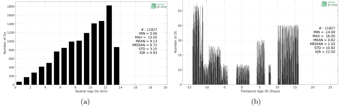
Figure 5: Histograms of the spatial (a) and temporal (b) lags between the location/time of the TSG (GOSUD-Research-vessel) measurement and the date of the corresponding SMOS SSS L3 v2 - Monthly - 0.25 Deg (CATDS-CECOS-IFREMER) SSS pixel.
