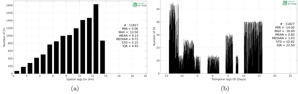
Figure 5: Histograms of the spatial (a) and temporal (b) lags between the time of the TSG (GOSUD-Research-vessel) measurements and the date of the corresponding SMOS SSS L3 v2 - Monthly - 0.25 Deg (CATDS-CECOS-IFREMER) SSS product.
