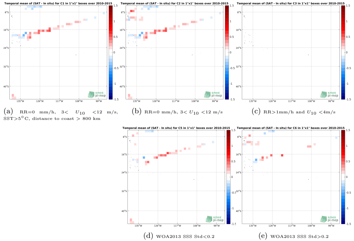
Figure 12: Temporal mean gridded over spatial boxes of size 1^\circ \times 1^\circ of \Delta SSS (SMOS SSS L3 v2 - Monthly - 0.25 Deg (CATDS-CECOS-IFREMER) - TSG (GOSUD-Research-vessel)) for 5 different subdatasets corresponding to: RR=0 mm/h, 3 < U_{10} < 12 m/s, SST > 5^\circ C , distance to coast > 800 km (a), RR=0 mm/h, 3 < U_{10} < 12 m/s (b), RR > 1 mm/h and U_{10} < 4 m/s (c), WOA2013 SSS Std < 0.2 (d), WOA2013 SSS Std > 0.2 (e).
