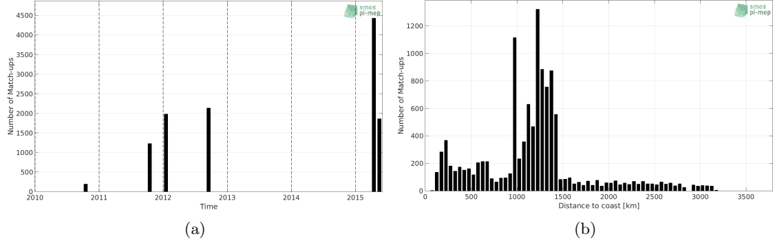
Figure 1: Number of match-ups between TSG (GOSUD-Research-vessel) and SMOS SSS L3 v2 - Monthly - 0.25 Deg (CATDS-CECOS-IFREMER) SSS as a function of time (a) and as function of the distance to coast (b) over the OTT zone Pi-MEP region and for the full satellite product period.
