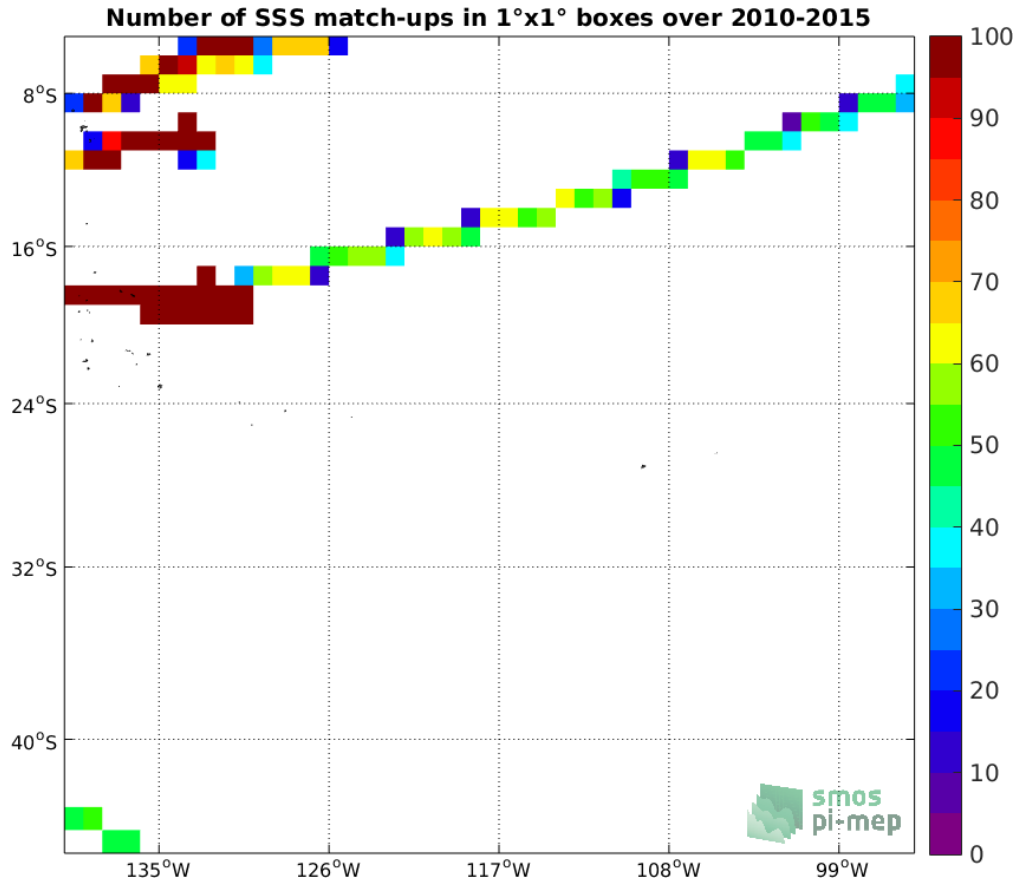
Figure 4: Number of SSS match-ups between TSG (GOSUD-Research-vessel) SSS and the SMOS SSS L3 v2 - Monthly - 0.25 Deg (CATDS-CECOS-IFREMER) SSS product for the OTT zone Pi-MEP region over 1°x1° boxes and for the full satellite product period.
