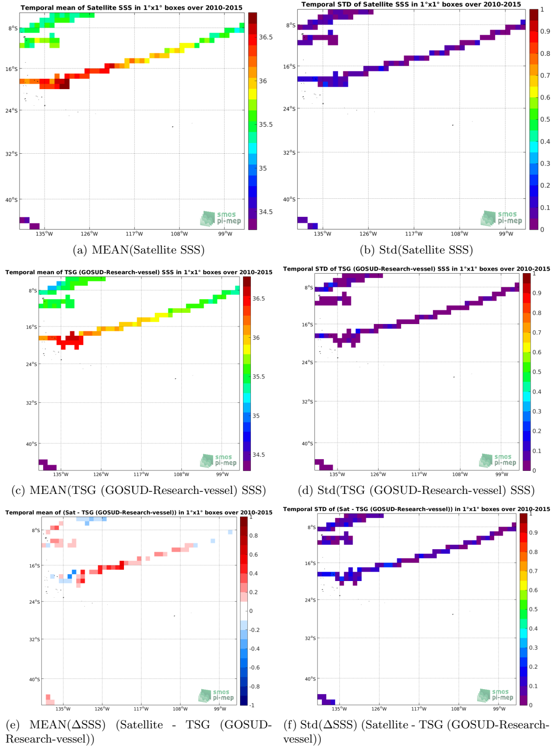
Figure 6: Temporal mean (left) and Std (right) of SSS from SMOS SSS L3 v2 - Monthly - 0.25 Deg (CATDS-CECOS-IFREMER) (top), TSG (GOSUD-Research-vessel) (middle), and of \Delta SSS (Satellite - TSG (GOSUD-Research-vessel)). Only match-up pairs are used to generate these maps.
