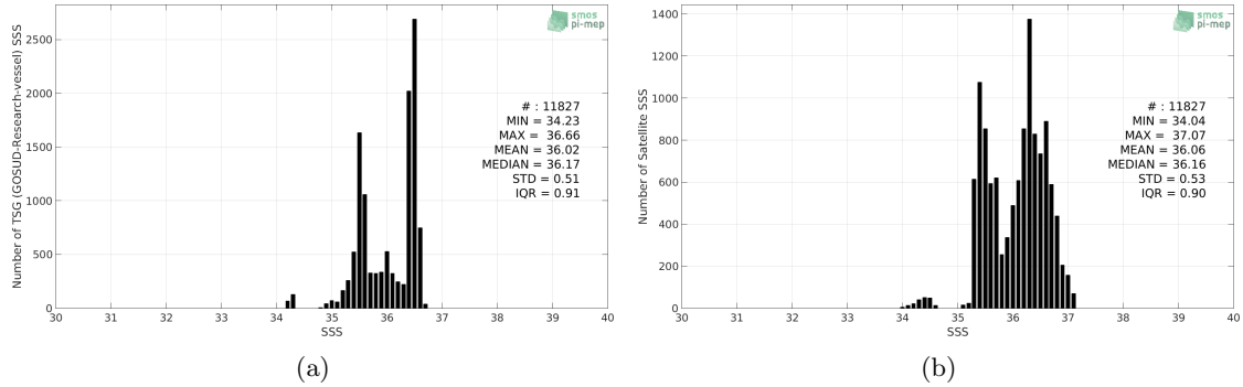
Figure 2: Histograms of SSS from TSG (GOSUD-Research-vessel) (a) and SMOS SSS L3 v2 - Monthly - 0.25 Deg (CATDS-CECOS-IFREMER) (b) considering all match-up pairs per bins of 0.1 over the OTT zone Pi-MEP region and for the full satellite product period.
