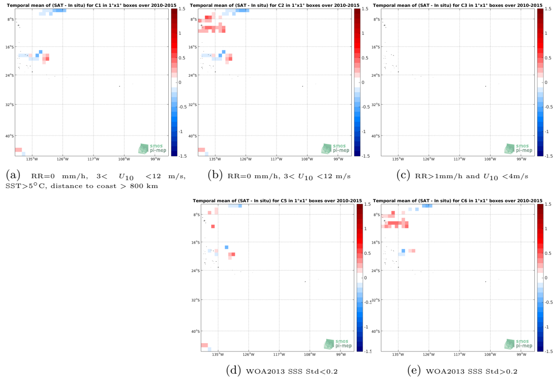
Figure 12: Temporal mean gridded over spatial boxes of size 1^\circ \times 1^\circ of \Delta SSS (SMOS-L3-CATDS-IFREMER-CECOS-V2-MONTHLY-0.25DEG - TSG-GOSUD-Research-vessel) for 5 different subdatasets corresponding to: RR=0 mm/h, 3 < U_{10} < 12 m/s, SST > 5^\circ\text{C} , distance to coast > 800 km (a), RR=0 mm/h, 3 < U_{10} < 12 m/s (b), RR > 1 mm/h and U_{10} < 4 m/s (c), WOA2013 SSS Std < 0.2 (d), WOA2013 SSS Std > 0.2 (e).
