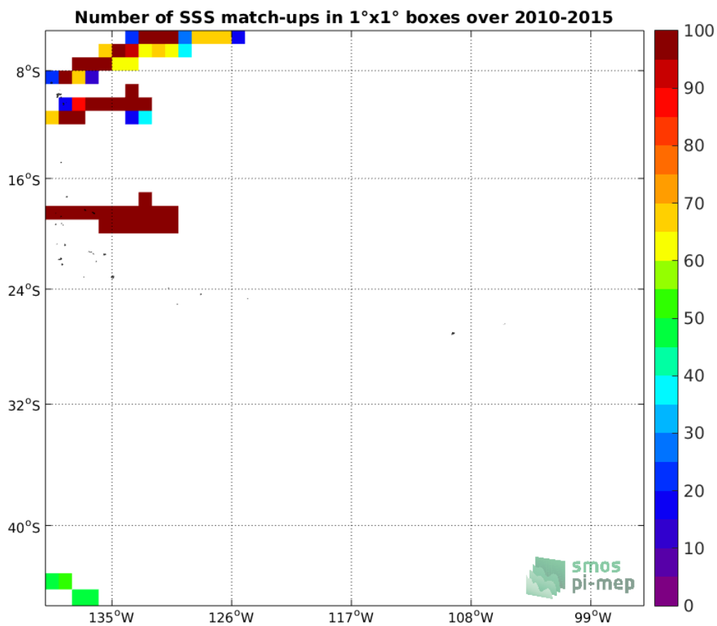
Figure 4: Number of SSS match-ups between TSG-GOSUD-Research-vessel SSS and the SMOS-L3-CATDS-IFREMER-CECOS-V2-MONTHLY-0.25DEG SSS product for the OTT zone Pi-MEP region over 1°x1° boxes and for the full satellite product period.
