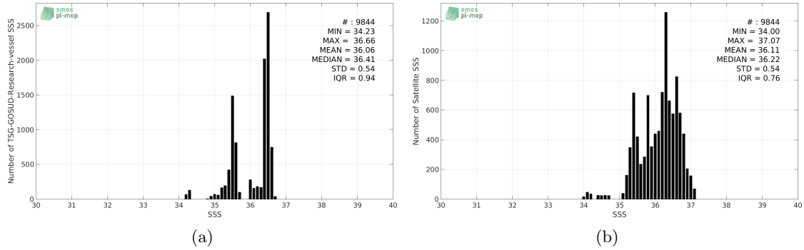
Figure 2: Histograms of SSS from TSG-GOSUD-Research-vessel (a) and SMOS-L3-CATDS-IFREMER-CECOS-V2-MONTHLY-0.25DEG (b) considering all match-up pairs per bins of 0.1 over the OTT zone Pi-MEP region and for the full satellite product period.
