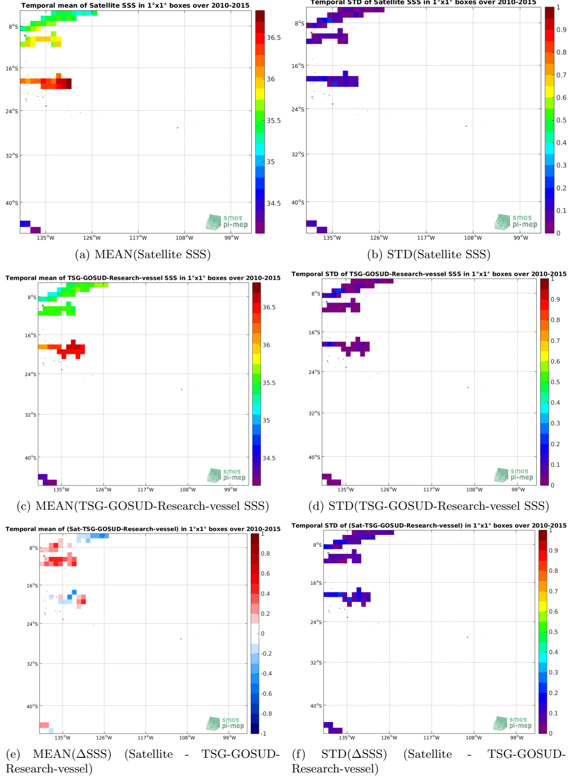
Figure 6: Temporal mean (left) and STD (right) of SSS from SMOS-L3-CATDS-IFREMER-CECOS-V2-MONTHLY-0.25DEG (top), TSG-GOSUD-Research-vessel (middle), and of \Delta SSS (Satellite - TSG-GOSUD-Research-vessel). Only match-up pairs are used to generate these maps.
