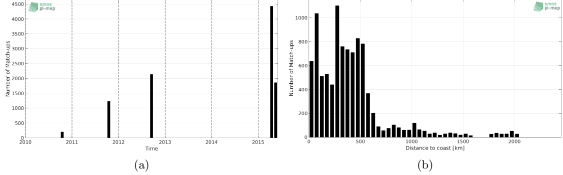
Figure 1: Number of match-ups between TSG-GOSUD-Research-vessel and SMOS-L3-CATDS-IFREMER-CECOS-V2-MONTHLY-0.25DEG SSS as a function of time (a) and as function of the distance to coast (b) over the OTT zone Pi-MEP region and for the full satellite product period.
