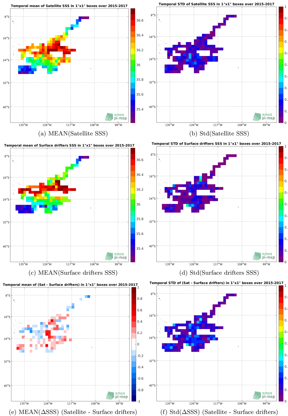
Figure 5: Temporal mean (left) and Std (right) of SSS from SMOS SSS L3 v2 - Monthly - 0.25 Deg (CATDS-CECOS-IFREMER) (top), Surface drifters (middle), and of \Delta SSS (Satellite - Surface drifters). Only match-up pairs are used to generate these maps.
