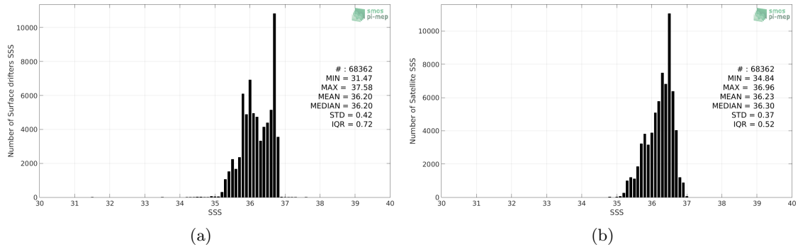
Figure 2: Histograms of SSS from Surface drifters (a) and SMOS SSS L3 v2 - Monthly - 0.25 Deg (CATDS-CECOS-IFREMER) (b) considering all match-up pairs per bins of 0.1 over the OTT zone Pi-MEP region and for the full satellite product period.
