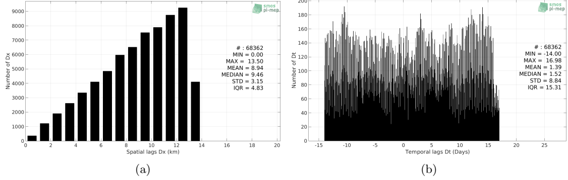
Figure 4: Histograms of the spatial (a) and temporal (b) lags between the time of the Surface drifters measurements and the date of the corresponding SMOS SSS L3 v2 - Monthly - 0.25 Deg (CATDS-CECOS-IFREMER) SSS product.
