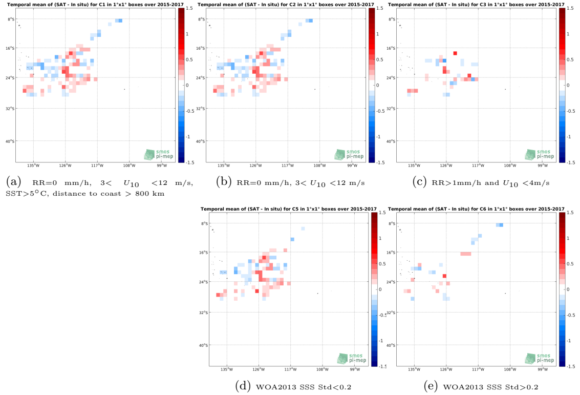
Figure 11: Temporal mean gridded over spatial boxes of size 1^{\circ}\times 1^{\circ} of \Delta\text{SSS} (SMOS SSS L3 v2 - Monthly - 0.25 Deg (CATDS-CECOS-IFREMER) - Surface drifters) for 5 different subdatasets corresponding to: RR=0 mm/h, 3 < U_{10} < 12 m/s, SST >5^{\circ}\text{C} , distance to coast > 800 km (a), RR=0 mm/h, 3 < U_{10} < 12 m/s (b), RR >1 mm/h and U_{10} < 4 m/s (c), WOA2013 SSS Std <0.2 (d), WOA2013 SSS Std >0.2 (e).
