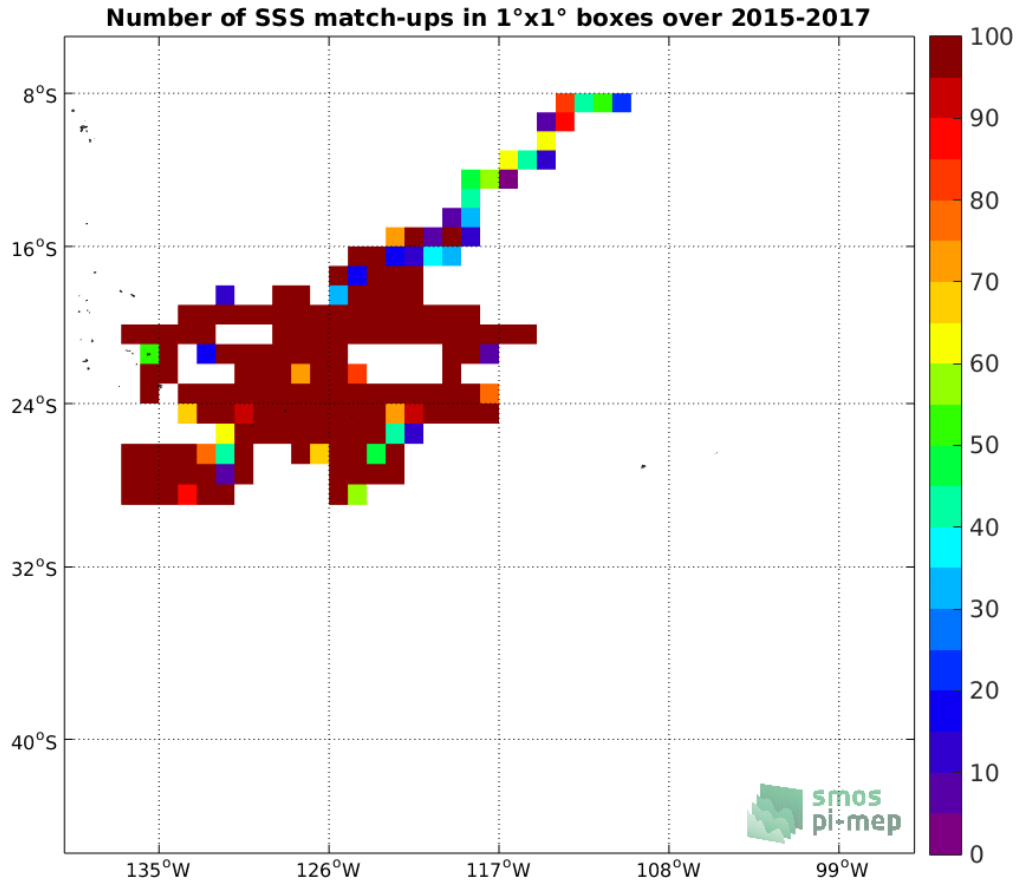
Figure 3: Number of SSS match-ups between Surface drifters SSS and the SMOS SSS L3 v2 - Monthly - 0.25 Deg (CATDS-CECOS-IFREMER) SSS product for the OTT zone Pi-MEP region over 1°x1° boxes and for the full satellite product period.
