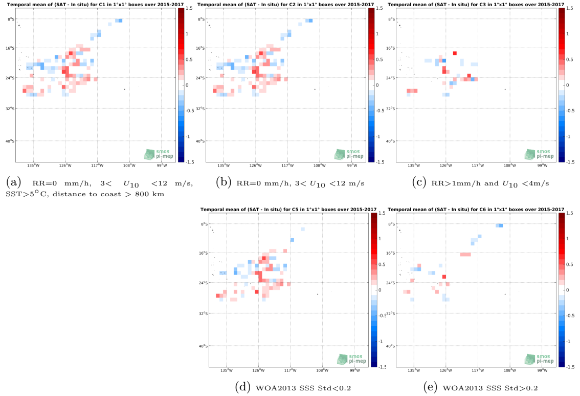
Figure 11: Temporal mean gridded over spatial boxes of size 1^{\circ}\times 1^{\circ} of \Delta\text{SSS} (SMOS L3 v2 - Monthly - 0.25 Deg (CATDS-CECOS-IFREMER) - Surface drifters) for 5 different subdatasets corresponding to:RR=0 mm/h, 3 < U_{10} < 12 m/s, SST >5^{\circ}\text{C} , distance to coast > 800 km (a), RR=0 mm/h, 3 < U_{10} < 12 m/s (b), RR >1\text{mm/h} and U_{10} < 4\text{m/s} (c), WOA2013 SSS Std <0.2 (d), WOA2013 SSS Std >0.2 (e).
