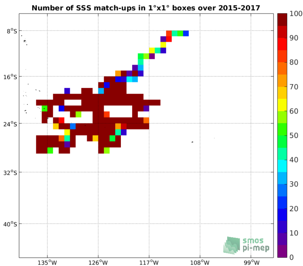
Figure 3: Number of SSS match-ups between Surface drifters SSS and the SMOS L3 v2 - Monthly - 0.25 Deg (CATDS-CECOS-IFREMER) SSS product for the OTT zone Pi-MEP region over 1°x1° boxes and for the full satellite product period.
