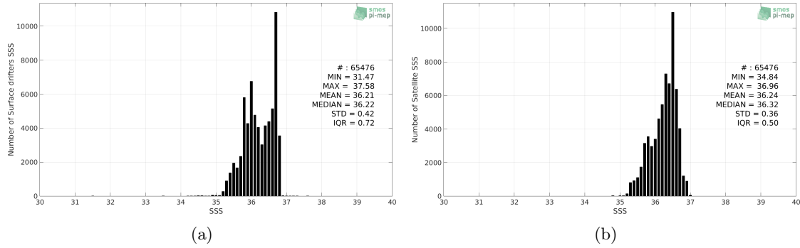
Figure 2: Histograms of SSS from Surface drifters (a) and SMOS L3 v2 - Monthly - 0.25 Deg (CATDS-CECOS-IFREMER) (b) considering all match-up pairs per bins of 0.1 over the OTT zone Pi-MEP region and for the full satellite product period.
