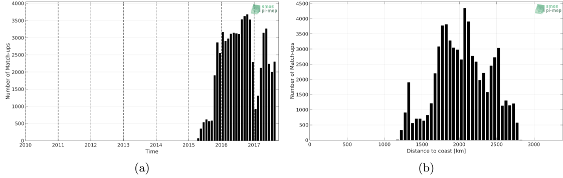
Figure 1: Number of match-ups between Surface drifters and SMOS L3 v2 - Monthly - 0.25 Deg (CATDS-CECOS-IFREMER) SSS as a function of time (a) and as function of the distance to coast (b) over the OTT zone Pi-MEP region and for the full satellite product period.
