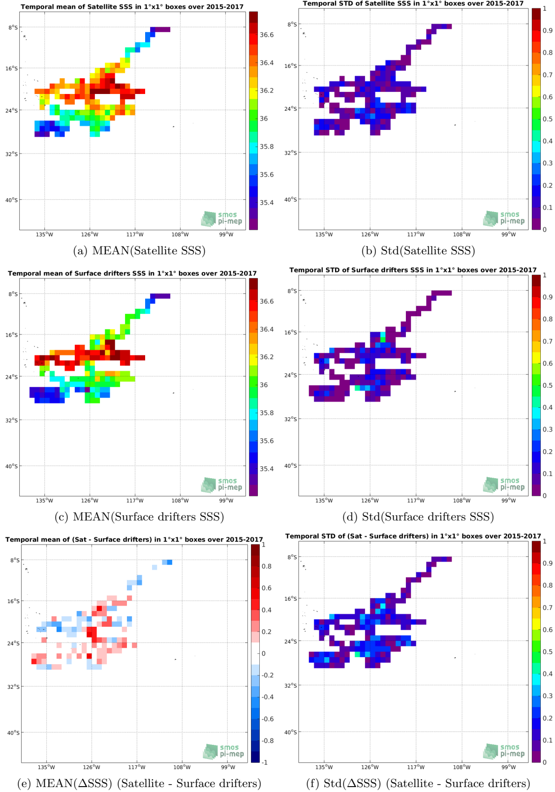
Figure 5: Temporal mean (left) and Std (right), of SSS from SMOS L3 v2 - Monthly - 0.25 Deg (CATDS-CECOS-IFREMER) (top), Surface drifters (middle), and of \Delta SSS (Satellite - Surface drifters). Only match-up pairs are used to generate these maps.
