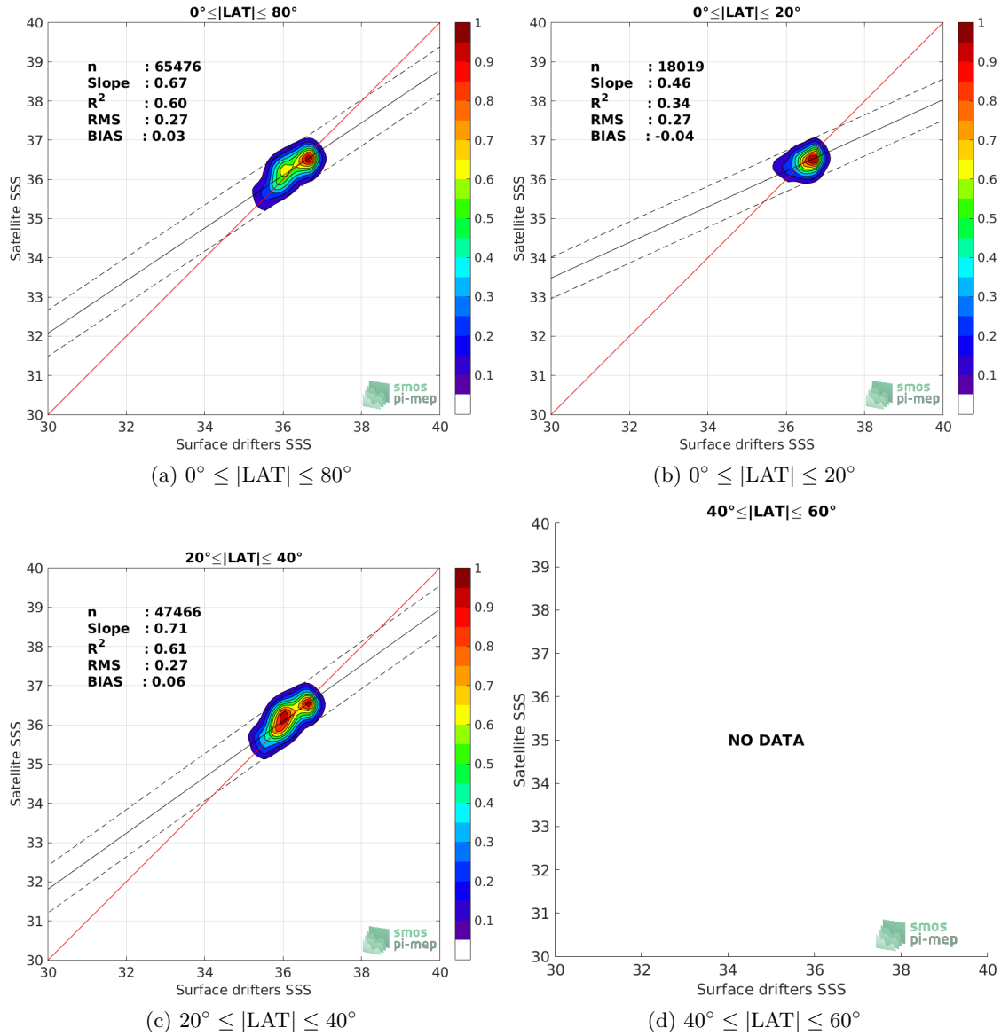
Figure 8: Contour maps of the concentration of SMOS L3 v2 - Monthly - 0.25 Deg (CATDS-CECOS-IFREMER) SSS (y-axis) versus Surface drifters SSS (x-axis) at match-up pairs for different latitude bands. For each plot, the red line shows x=y . The black thin and dashed lines indicate a linear fit through the data cloud and the \pm 95\% confidence levels, respectively. The number match-up pairs n , the slope and R^2 coefficient of the linear fit, the root mean square (RMS) and the mean bias between satellite and in situ data are indicated for each latitude band in each plots.
