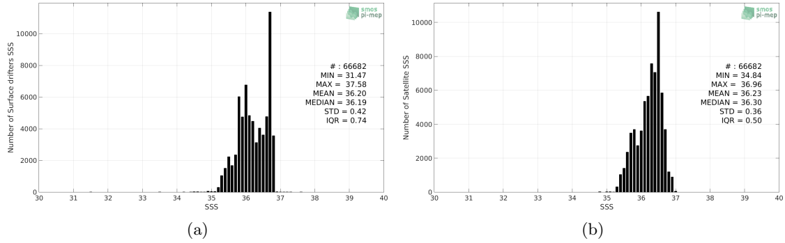
Figure 2: Histograms of SSS from Surface drifters (a) and SMOS-L3-CATDS-IFREMER-CECOS-V2-MONTHLY-0.25DEG (b) considering all match-up pairs per bins of 0.1 over the OTT zone Pi-MEP region and for the full satellite product period.
