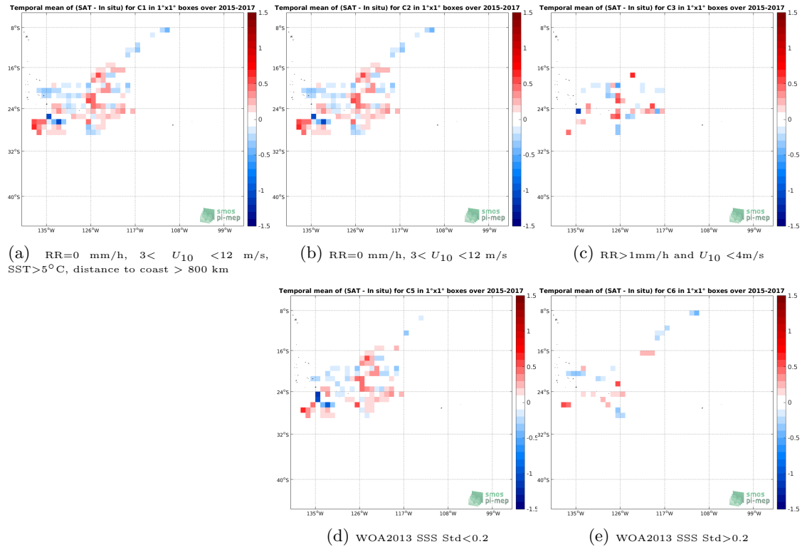
Figure 11: Temporal mean gridded over spatial boxes of size 1^\circ \times 1^\circ of \Delta SSS (SMOS-L3-CATDS-IFREMER-CECOS-V2-MONTHLY-0.25DEG - Surface drifters) for 5 different subdatasets corresponding to:RR=0 mm/h, 3 < U_{10} < 12 m/s, SST >5^\circ C, distance to coast > 800 km (a), RR=0 mm/h, 3 < U_{10} < 12 m/s (b), RR >1 mm/h and U_{10} < 4 m/s (c), WOA2013 SSS Std <0.2 (d), WOA2013 SSS Std >0.2 (e).
