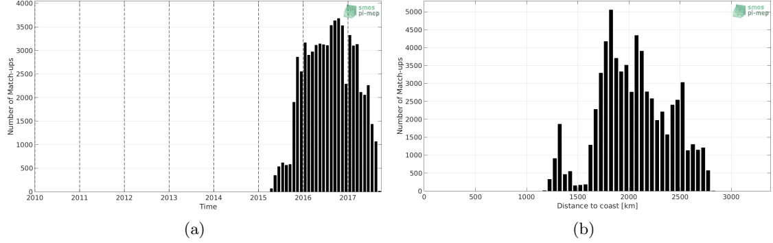
Figure 1: Number of match-ups between Surface drifters and SMOS-L3-CATDS-IFREMER-CECOS-V2-MONTHLY-0.25DEG SSS as a function of time (a) and as function of the distance to coast (b) over the OTT zone Pi-MEP region and for the full satellite product period.
