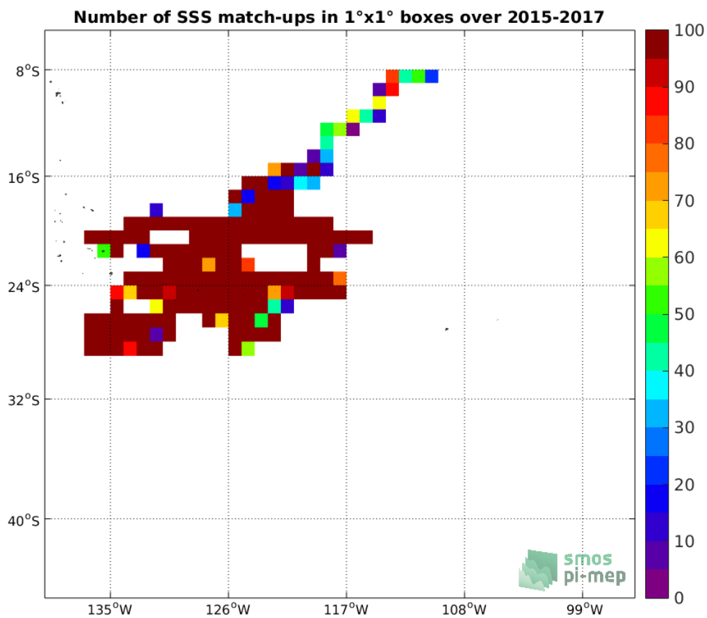
Figure 3: Number of SSS match-ups between Surface drifters SSS and the SMOS-L3-CATDS-IFREMER-CECOS-V2-MONTHLY-0.25DEG SSS product for the OTT zone Pi-MEP region over 1°x1° boxes and for the full satellite product period.
