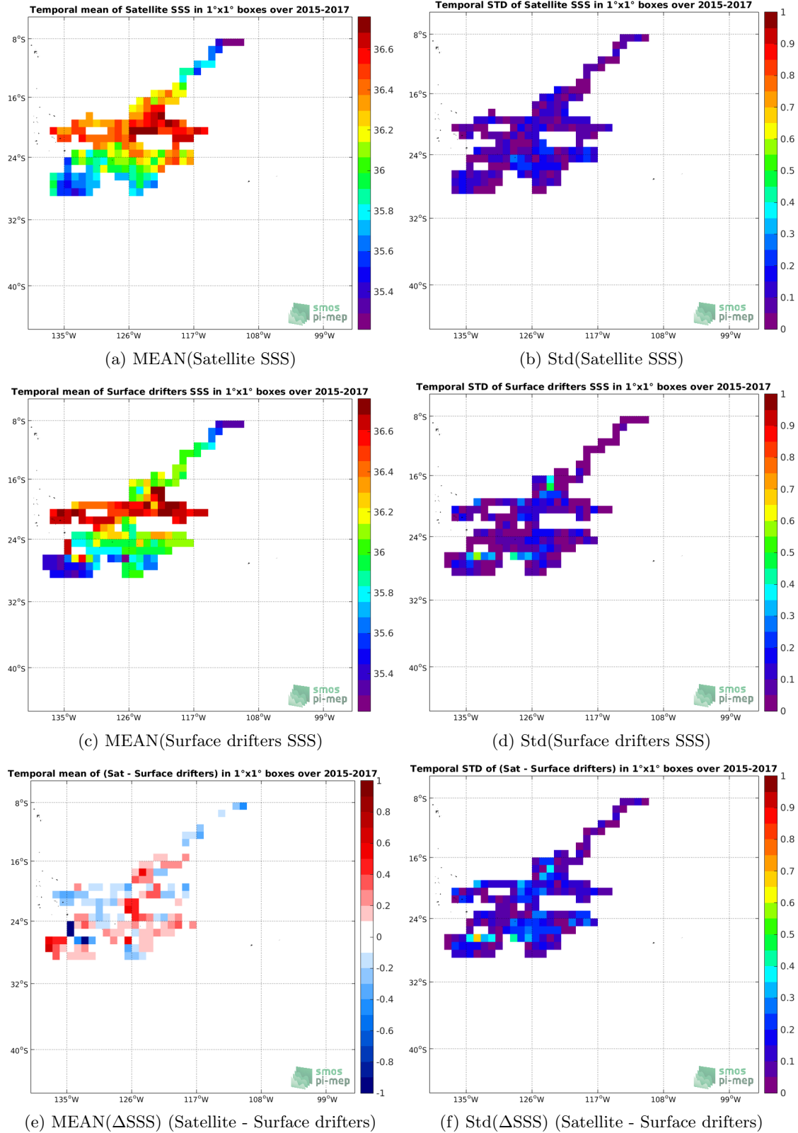
Figure 5: Temporal mean (left) and Std (right) of SSS from SMOS-L3-CATDS-IFREMER-CECOS-V2-MONTHLY-0.25DEG (top), Surface drifters (middle), and of \Delta SSS (Satellite - Surface drifters). Only match-up pairs are used to generate these maps.
