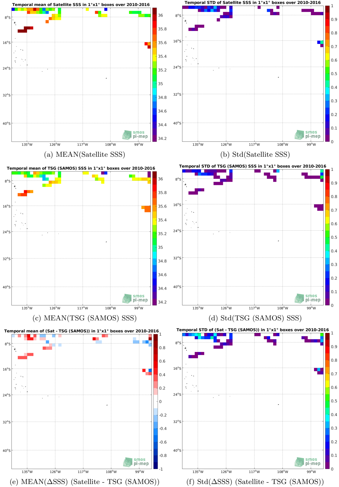
Figure 6: Temporal mean (left) and Std (right) of SSS from SMOS SSS L3 v2 - Daily - 0.5 Deg (CATDS-CECOS-IFREMER) (top), TSG (SAMOS) (middle), and of \Delta SSS (Satellite - TSG (SAMOS)). Only match-up pairs are used to generate these maps.
