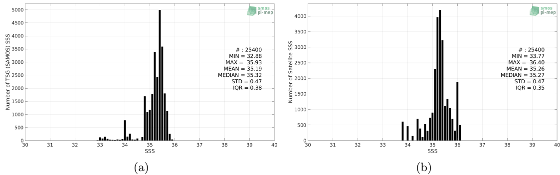
Figure 2: Histograms of SSS from TSG (SAMOS) (a) and SMOS SSS L3 v2 - Daily - 0.5 Deg (CATDS-CECOS-IFREMER) (b) considering all match-up pairs per bins of 0.1 over the OTT zone Pi-MEP region and for the full satellite product period.
