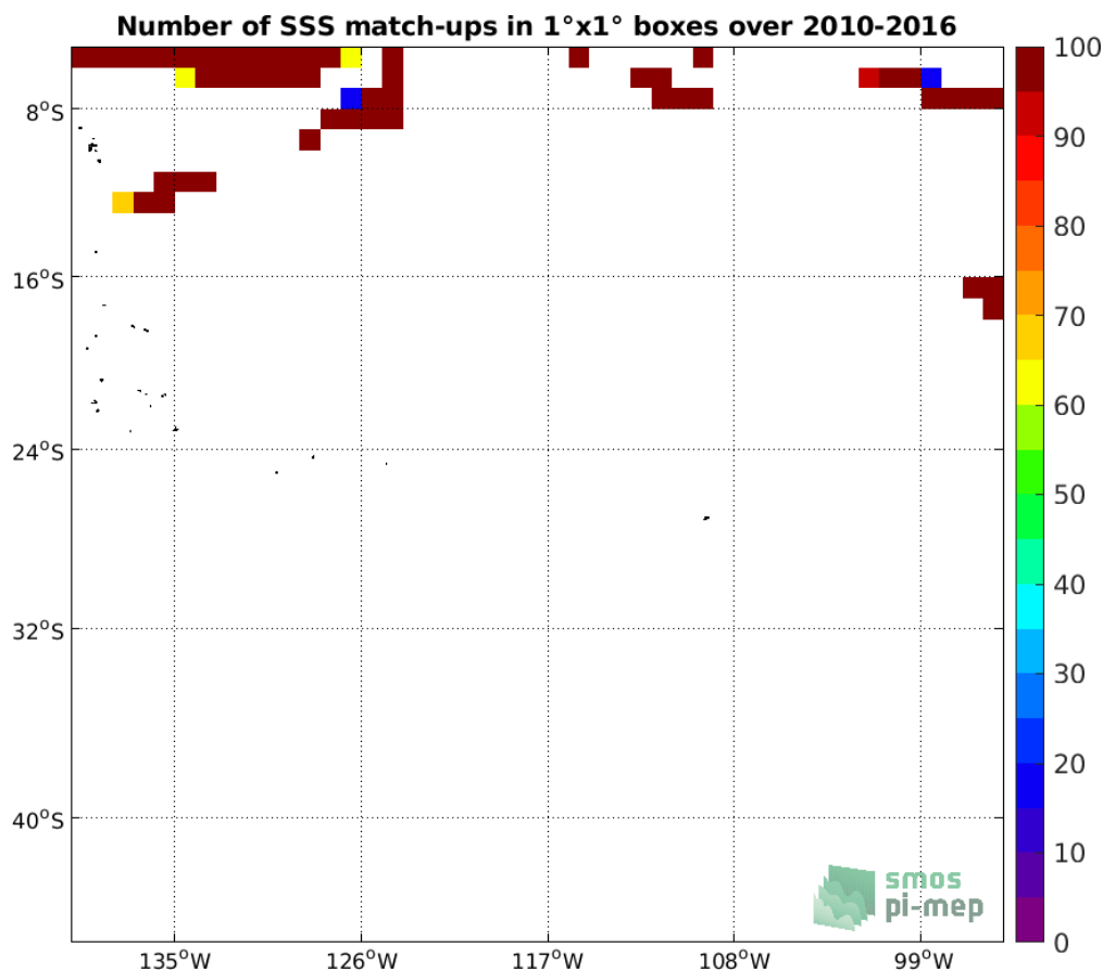
Figure 4: Number of SSS match-ups between TSG (SAMOS) SSS and the SMOS SSS L3 v2 - Daily - 0.5 Deg (CATDS-CECOS-IFREMER) SSS product for the OTT zone Pi-MEP region over 1°x1° boxes and for the full satellite product period.
