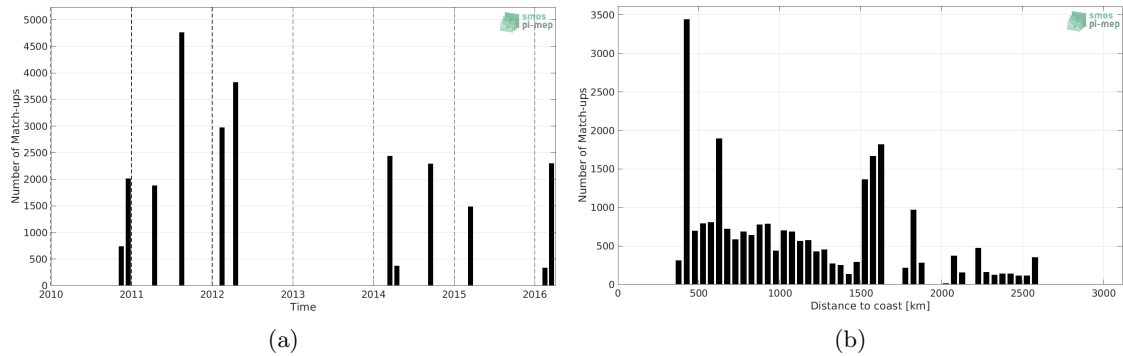
Figure 1: Number of match-ups between TSG (SAMOS) and SMOS SSS L3 v2 - Daily - 0.5 Deg (CATDS-CECOS-IFREMER) SSS as a function of time (a) and as function of the distance to coast (b) over the OTT zone Pi-MEP region and for the full satellite product period.
