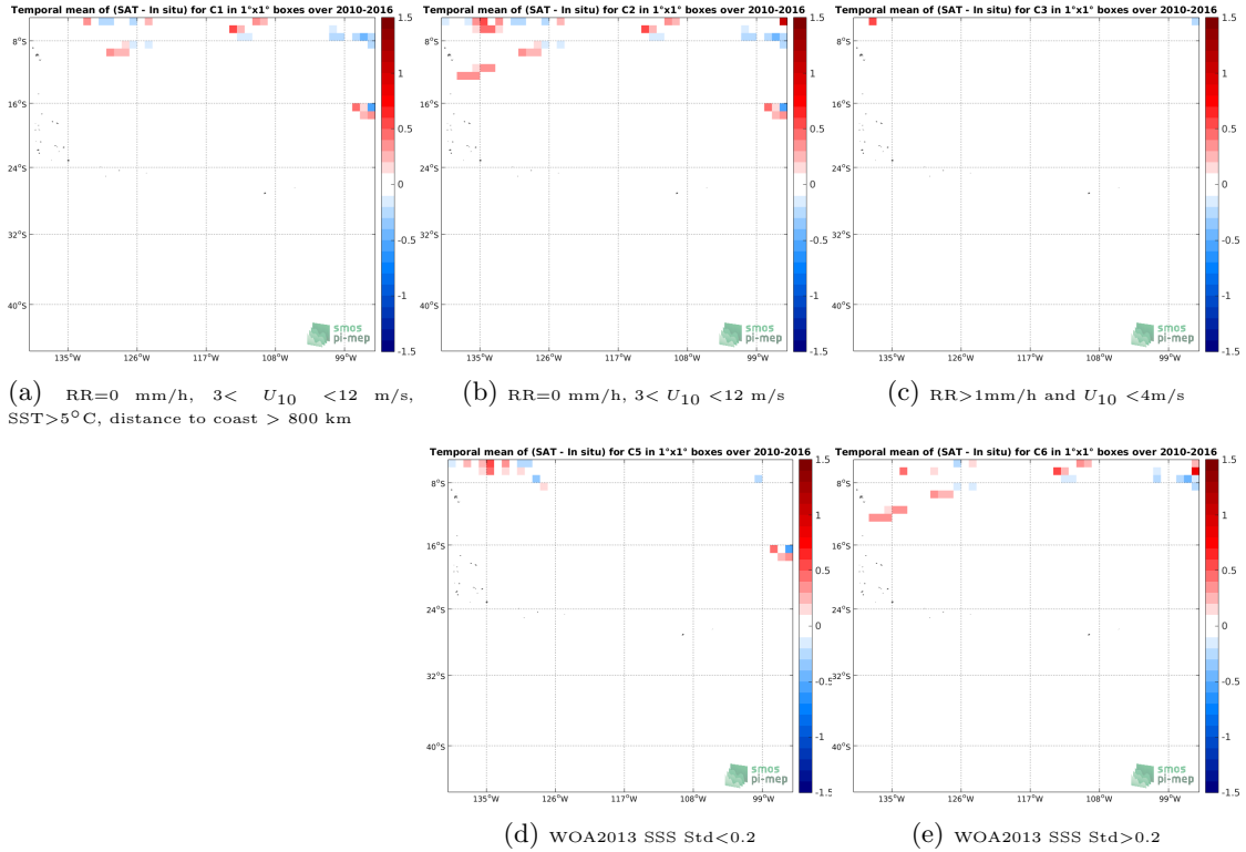
Figure 12: Temporal mean gridded over spatial boxes of size 1^{\circ}\times 1^{\circ} of \Delta\text{SSS} (SMOS SSS L3 v2 - Daily - 0.5 Deg (CATDS-CECOS-IFREMER) - TSG (SAMOS)) for 5 different subdatasets corresponding to: \text{RR}=0 mm/h, 3 < U_{10} < 12 m/s, \text{SST}>5^{\circ}\text{C} , distance to coast > 800 km (a), \text{RR}=0 mm/h, 3 < U_{10} < 12 m/s (b), \text{RR}>1 mm/h and U_{10} < 4 m/s (c), \text{WOA2013 SSS Std}<0.2 (d), \text{WOA2013 SSS Std}>0.2 (e).
