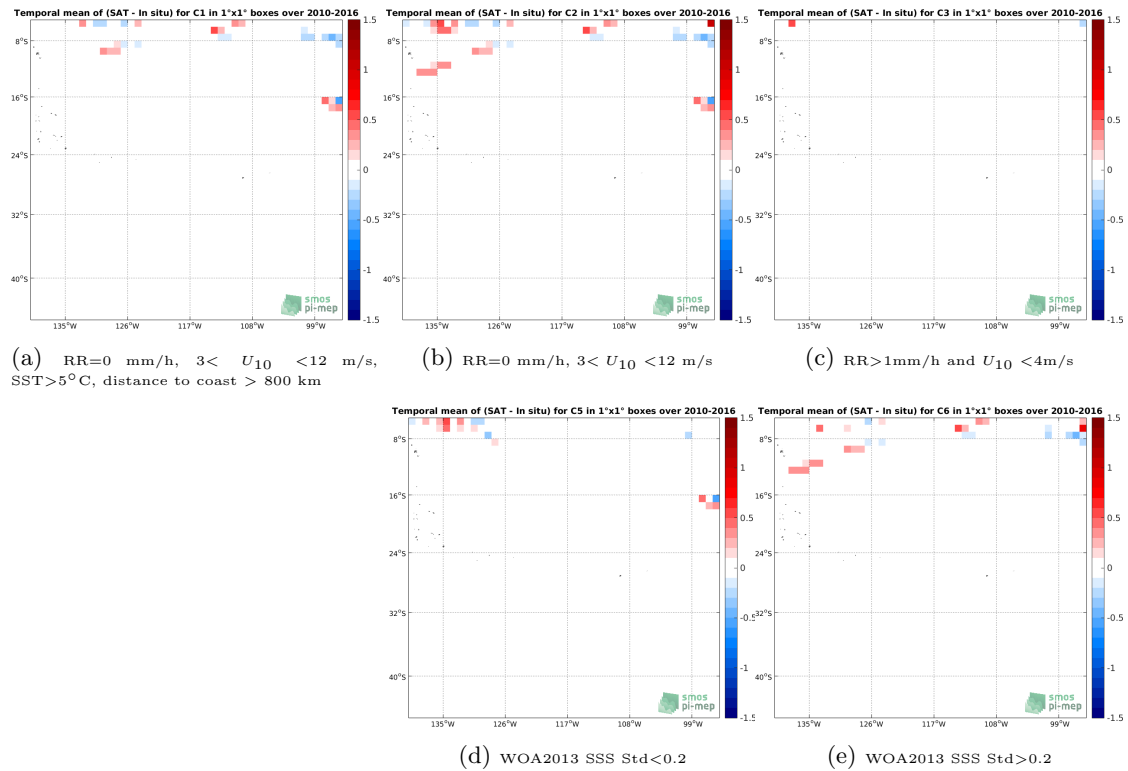
Figure 12: Temporal mean gridded over spatial boxes of size 1^\circ \times 1^\circ of \Delta SSS (SMOS L3 v2 - Daily - 0.5 Deg (CATDS-CECOS-IFREMER) - TSG-SAMOS) for 5 different subdatasets corresponding to:RR=0 mm/h, 3 < U_{10} < 12 m/s, SST >5^\circ C, distance to coast > 800 km (a), RR=0 mm/h, 3 < U_{10} < 12 m/s (b), RR >1 mm/h and U_{10} < 4 m/s (c), WOA2013 SSS Std <0.2 (d), WOA2013 SSS Std >0.2 (e).
