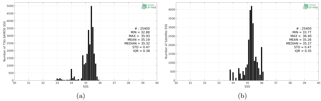
Figure 2: Histograms of SSS from TSG-SAMOS (a) and SMOS L3 v2 - Daily - 0.5 Deg (CATDS-CECOS-IFREMER) (b) considering all match-up pairs per bins of 0.1 over the OTT zone Pi-MEP region and for the full satellite product period.
