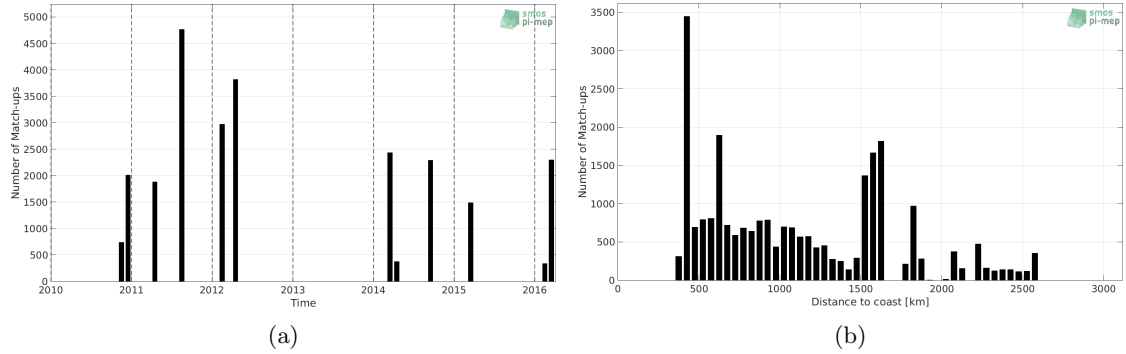
Figure 1: Number of match-ups between TSG-SAMOS and SMOS L3 v2 - Daily - 0.5 Deg (CATDS-CECOS-IFREMER) SSS as a function of time (a) and as function of the distance to coast (b) over the OTT zone Pi-MEP region and for the full satellite product period.
