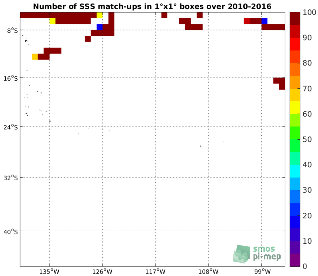
Figure 4: Number of SSS match-ups between TSG-SAMOS SSS and the SMOS L3 v2 - Daily - 0.5 Deg (CATDS-CECOS-IFREMER) SSS product for the OTT zone Pi-MEP region over 1°x1° boxes and for the full satellite product period.
