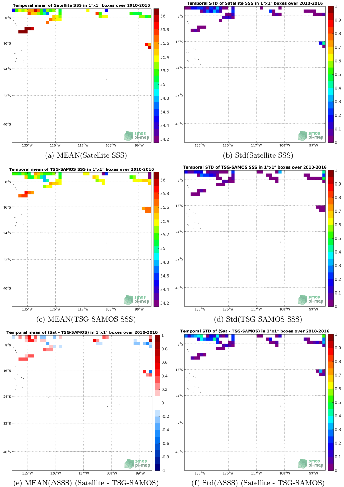
Figure 6: Temporal mean (left) and Std (right) of SSS from SMOS L3 v2 - Daily - 0.5 Deg (CATDS-CECOS-IFREMER) (top), TSG-SAMOS (middle), and of \Delta SSS (Satellite - TSG-SAMOS). Only match-up pairs are used to generate these maps.
