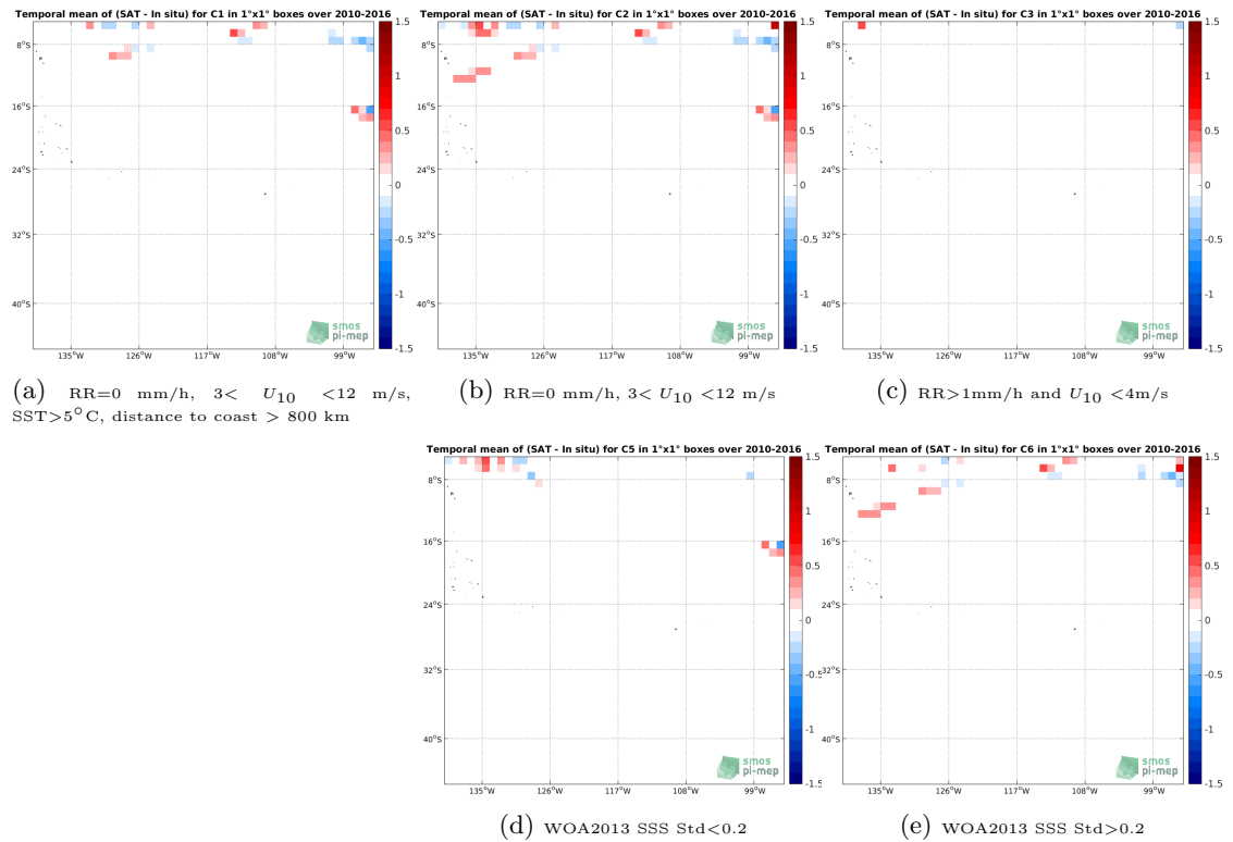
Figure 12: Temporal mean gridded over spatial boxes of size 1^\circ \times 1^\circ of \Delta SSS (SMOS-L3-CATDS-CECOS-IFREMER-V2-1DAY-0.5DEG - TSG-SAMOS) for 5 different subdatasets corresponding to: RR=0 mm/h, 3 < U_{10} < 12 m/s, SST > 5^\circ\text{C} , distance to coast > 800 km (a), RR=0 mm/h, 3 < U_{10} < 12 m/s (b), RR > 1 mm/h and U_{10} < 4 m/s (c), WOA2013 SSS Std < 0.2 (d), WOA2013 SSS Std > 0.2 (e).
