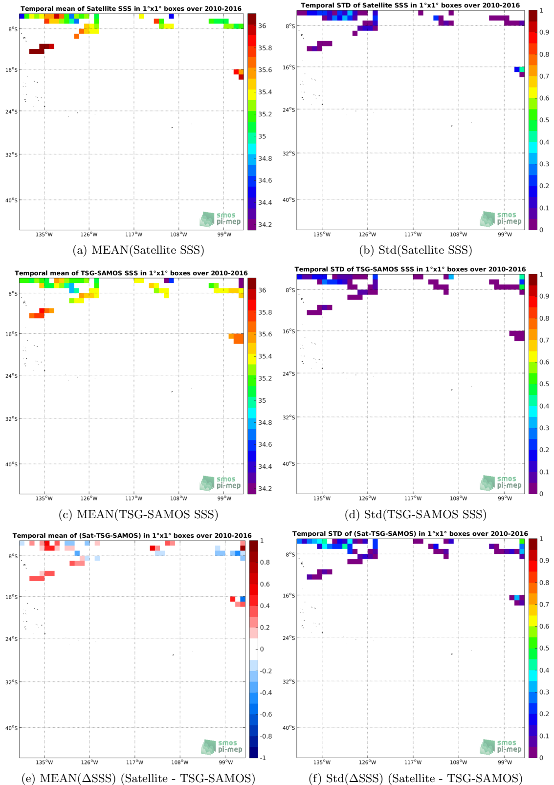
Figure 6: Temporal mean (left) and Std (right) of SSS from SMOS-L3-CATDS-CECOS-IFREMER-V2-1DAY-0.5DEG (top), TSG-SAMOS (middle), and of \Delta SSS (Satellite - TSG-SAMOS). Only match-up pairs are used to generate these maps.
