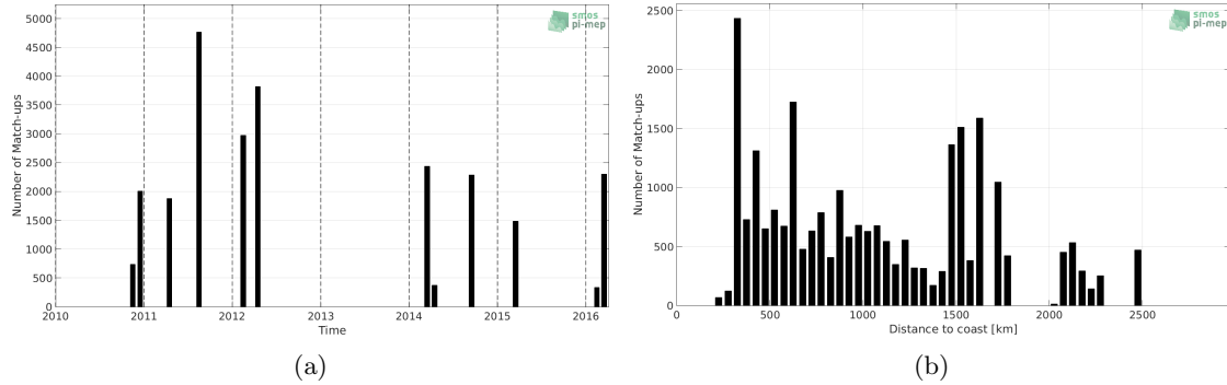
Figure 1: Number of match-ups between TSG-SAMOS and SMOS-L3-CATDS-CECOS-IFREMER-V2-1DAY-0.5DEG SSS as a function of time (a) and as function of the distance to coast (b) over the OTT zone Pi-MEP region and for the full satellite product period.
