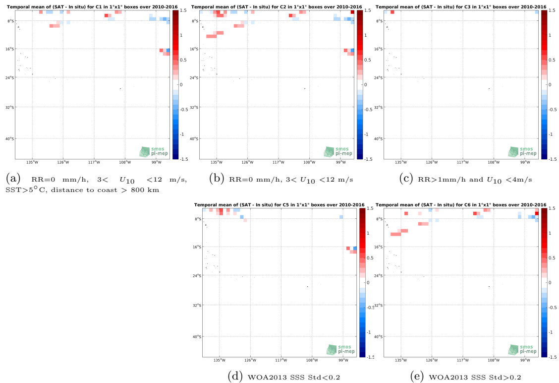
Figure 12: Temporal mean gridded over spatial boxes of size 1^\circ \times 1^\circ of \Delta SSS (SMOS-L3-CATDS-CECOS-IFREMER-V2-1DAY-0.5DEG - TSG-SAMOS) for 5 different subdatasets corresponding to:RR=0 mm/h, 3 < U_{10} < 12 m/s, SST >5^\circ C, distance to coast > 800 km (a), RR=0 mm/h, 3 < U_{10} < 12 m/s (b), RR >1 mm/h and U_{10} < 4 m/s (c), WOA2013 SSS Std <0.2 (d), WOA2013 SSS Std >0.2 (e).
