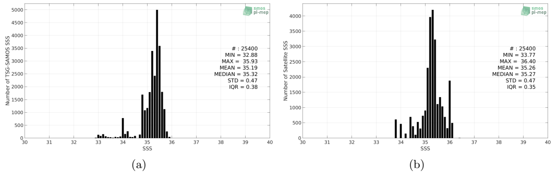
Figure 2: Histograms of SSS from TSG-SAMOS (a) and SMOS-L3-CATDS-CECOS-IFREMER-V2-1DAY-0.5DEG (b) considering all match-up pairs per bins of 0.1 over the OTT zone Pi-MEP region and for the full satellite product period.
