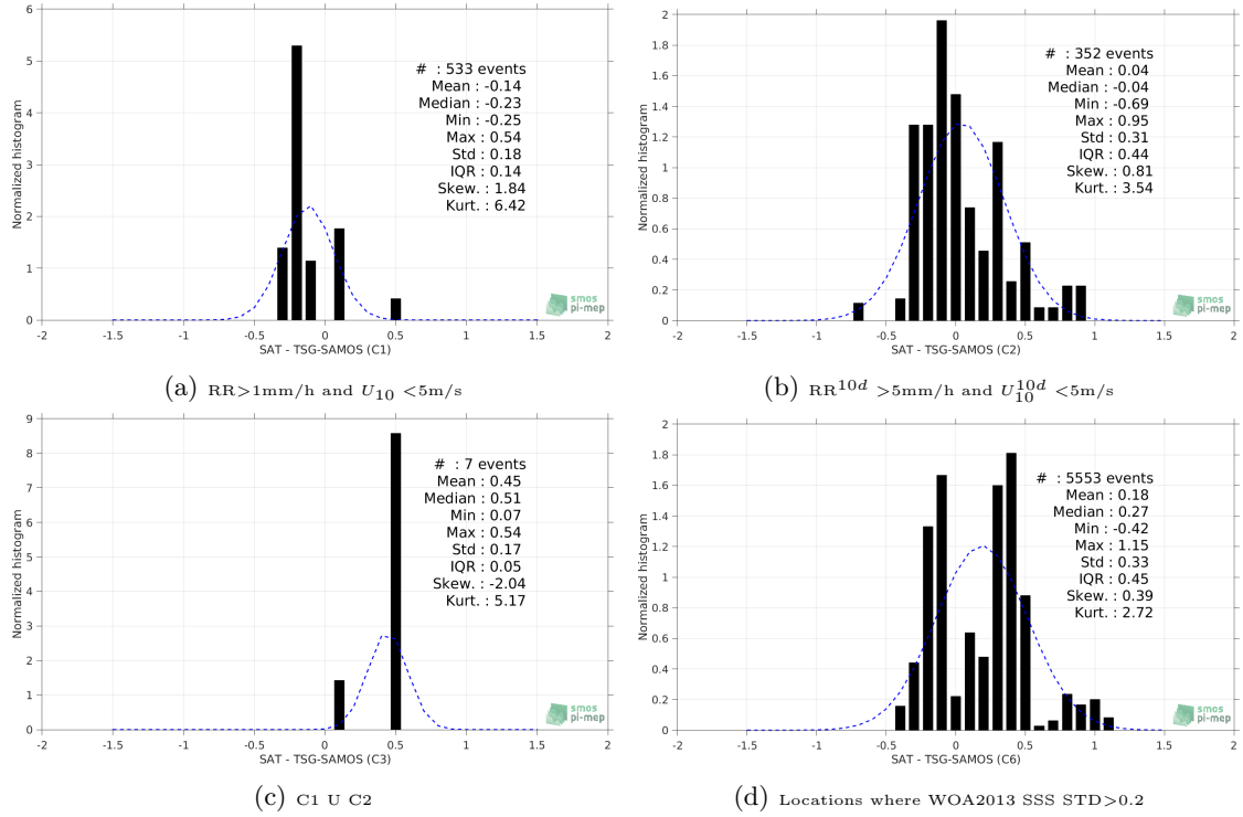
Figure 13: Normalized histogram of \Delta\text{SSS} (SMOS-L3-CATDS-CECOS-IFREMER-V2-1DAY-0.5DEG - TSG-SAMOS) for 6 different subdatasets corresponding to: RR > 1\text{mm/h} and U_{10} < 5\text{m/s} (a), RR^{10d} > 5\text{mm/h} and U_{10}^{10d} < 5\text{m/s} (b), C1 U C2 (c), Locations where WOA2013 SSS STD > 0.2 (d).
