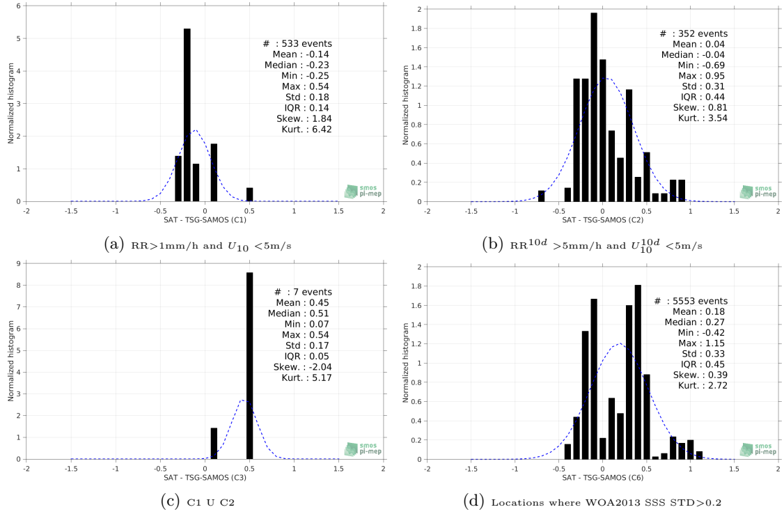
Figure 13: Normalized histogram of \Delta\text{SSS} (SMOS-L3-CATDS-CECOS-IFREMER-V2-1DAY-0.5DEG - TSG-SAMOS) for 6 different subdatasets corresponding to: RR > 1mm/h and U_{10} < 5\text{m/s} (a), RR^{10d} > 5\text{mm/h} and U_{10}^{10d} < 5\text{m/s} (b), C1 U C2 (c), Locations where WOA2013 SSS STD > 0.2 (d).
