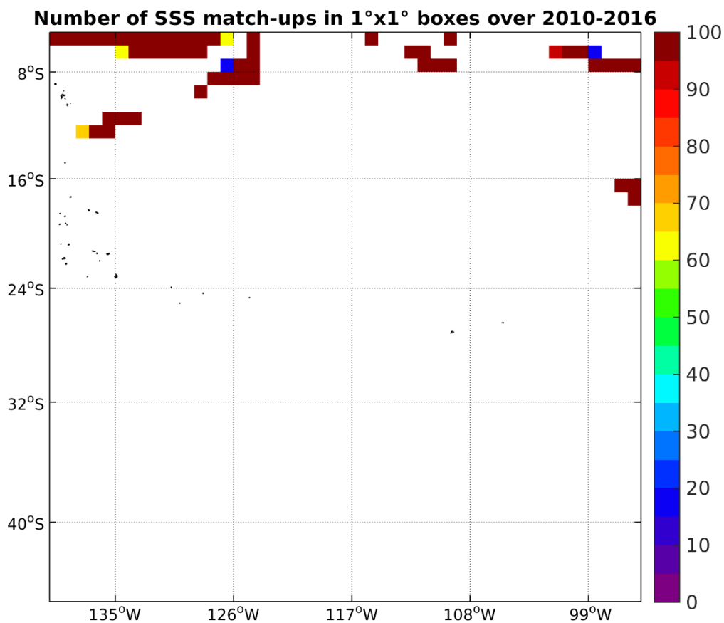
Figure 4: Number of SSS match-ups between TSG-SAMOS SSS and the SMOS-L3-CATDS-CECOS-IFREMER-V2-1DAY-0.5DEG SSS product for the OTT zone Pi-MEP region over 1°x1° boxes and for the full satellite product period.
