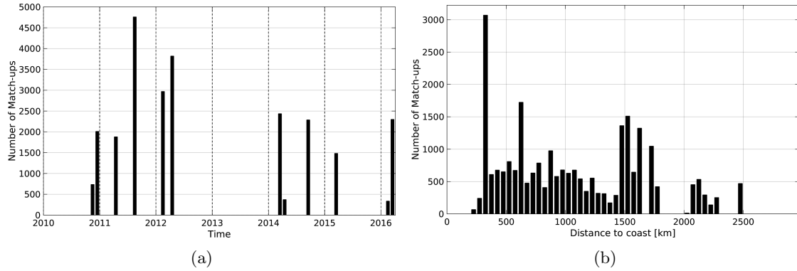
Figure 1: Number of match-ups between TSG-SAMOS and SMOS-L3-CATDS-CECOS-IFREMER-V2-1DAY-0.5DEG SSS as a function of time (a) and as function of the distance to coast (b) over the OTT zone Pi-MEP region and for the full satellite product period.
