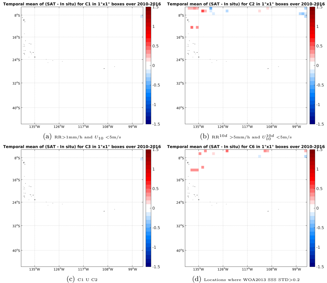
Figure 12: Temporal mean gridded over spatial boxes of size 1^\circ \times 1^\circ of \Delta SSS (SMOS-L3-CATDS-CECOS-IFREMER-V2-1DAY-0.5DEG - TSG-SAMOS) for 4 different subdatasets corresponding to: RR > 1 mm/h and U_{10} < 5 m/s (a), RR 10d > 5 mm/h and U_{10}^{10d} < 5 m/s (b), C1 U C2 (c), Locations where WOA2013 SSS STD > 0.2 (d).
