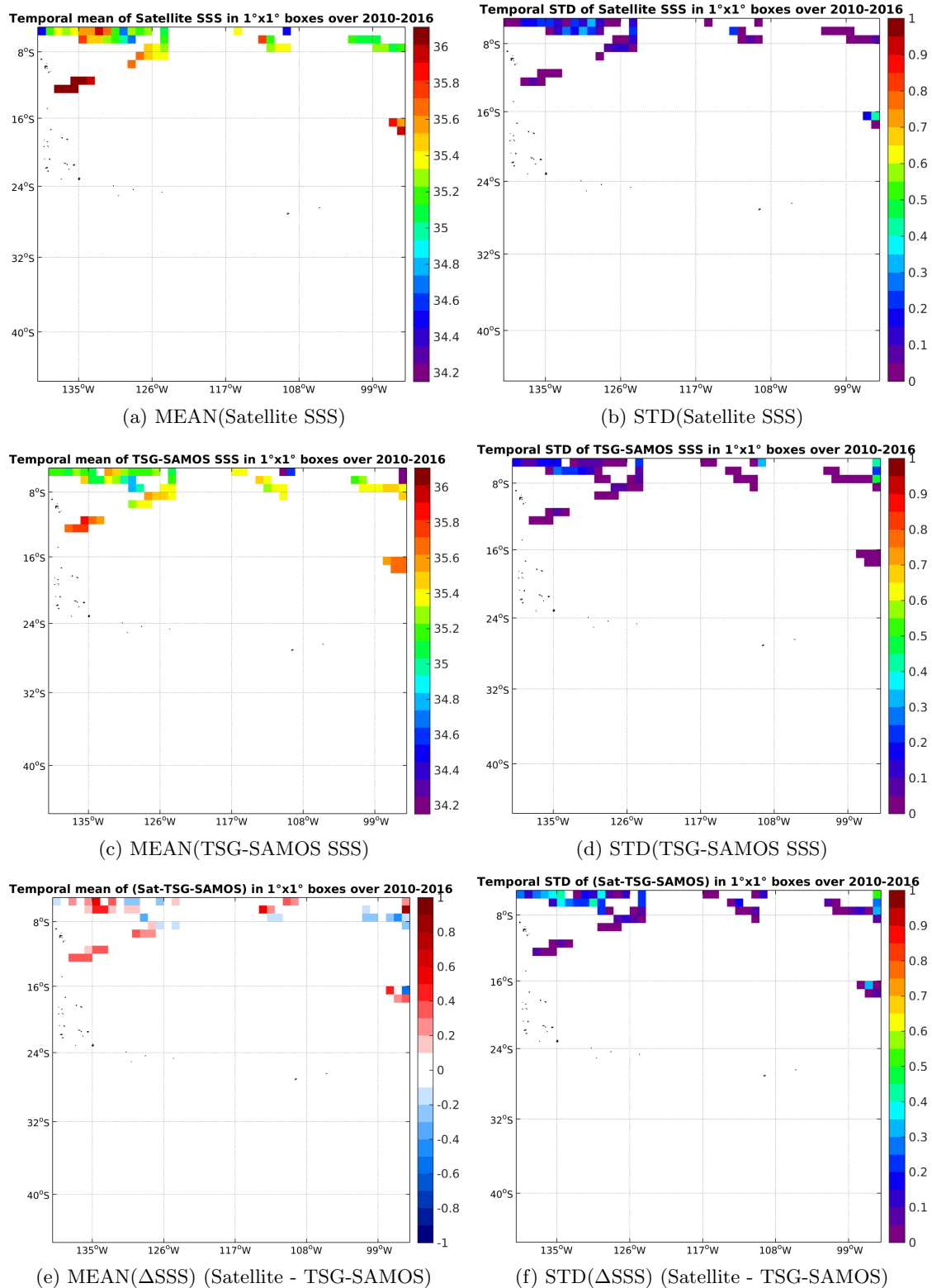
Figure 6: Temporal mean (left) and STD (right) of SSS from SMOS-L3-CATDS-CECOS-IFREMER-V2-1DAY-0.5DEG (top), TSG-SAMOS (middle), and of \Delta SSS (Satellite - TSG-SAMOS). Only match-up pairs are used to generate these maps.
