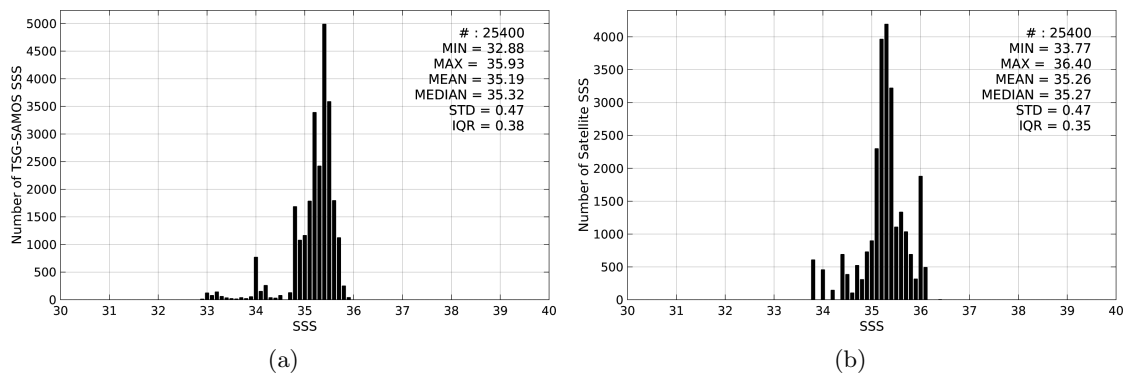
Figure 2: Histograms of SSS from TSG-SAMOS (a) and SMOS-L3-CATDS-CECOS-IFREMER-V2-1DAY-0.5DEG (b) considering all match-up pairs per bins of 0.1 over the OTT zone Pi-MEP region and for the full satellite product period.
