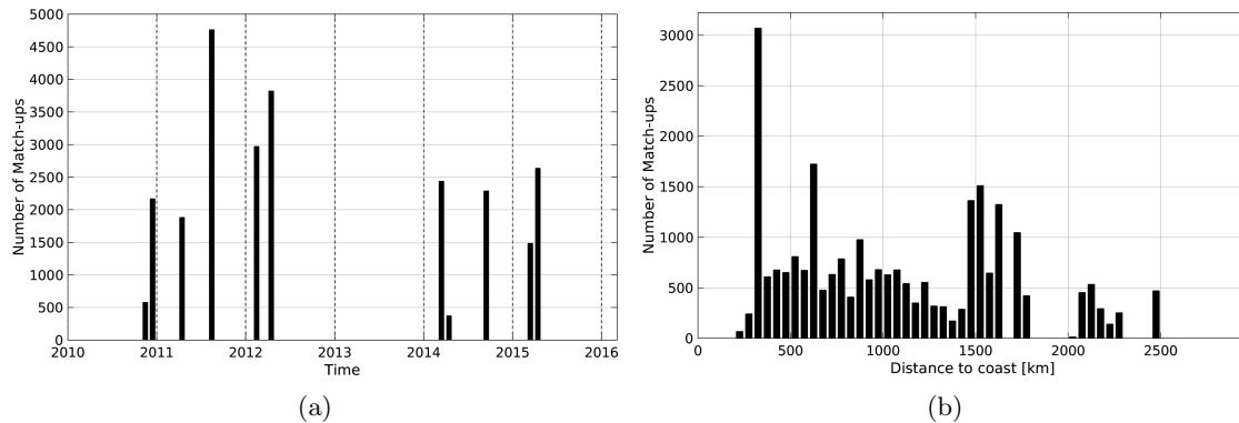
Figure 1: Number of match-ups between TSG-SAMOS and SMOS-L3-CATDS-CECOS-IFREMER-V2-1DAY-0.5deg SSS as a function of time (a) and as function of the distance to coast (b) over the OTT zone Pi-MEP region and for the full satellite product period.
