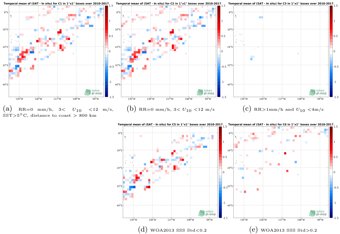
Figure 12: Temporal mean gridded over spatial boxes of size 1^{\circ}\times 1^{\circ} of \Delta\text{SSS} (SMOS SSS L3 v2 - Daily - 0.5 Deg (CATDS-CECOS-IFREMER) - TSG (LEGOS-DM)) for 5 different subdatasets corresponding to:RR=0 mm/h, 3 < U_{10} < 12 m/s, SST >5^{\circ}\text{C} , distance to coast > 800 km (a), RR=0 mm/h, 3 < U_{10} < 12 m/s (b), RR >1 mm/h and U_{10} < 4 m/s (c), WOA2013 SSS Std <0.2 (d), WOA2013 SSS Std >0.2 (e).
