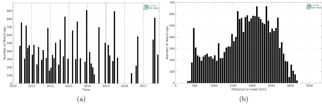
Figure 1: Number of match-ups between TSG (LEGOS-DM) and SMOS SSS L3 v2 - Daily - 0.5 Deg (CATDS-CECOS-IFREMER) SSS as a function of time (a) and as function of the distance to coast (b) over the OTT zone Pi-MEP region and for the full satellite product period.
