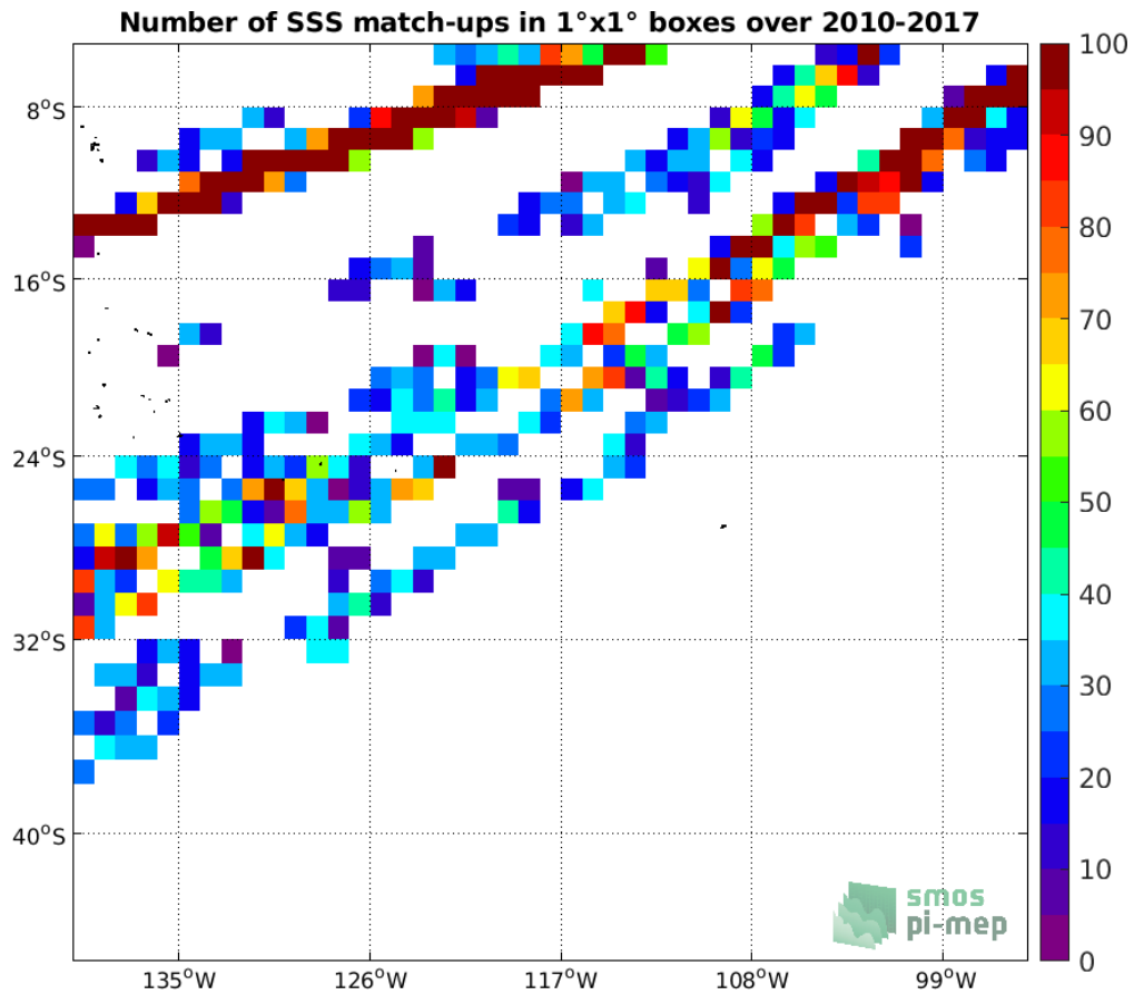
Figure 4: Number of SSS match-ups between TSG (LEGOS-DM) SSS and the SMOS SSS L3 v2 - Daily - 0.5 Deg (CATDS-CECOS-IFREMER) SSS product for the OTT zone Pi-MEP region over 1°x1° boxes and for the full satellite product period.
