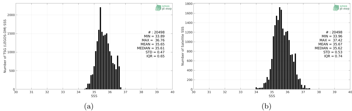
Figure 2: Histograms of SSS from TSG (LEGOS-DM) (a) and SMOS SSS L3 v2 - Daily - 0.5 Deg (CATDS-CECOS-IFREMER) (b) considering all match-up pairs per bins of 0.1 over the OTT zone Pi-MEP region and for the full satellite product period.
