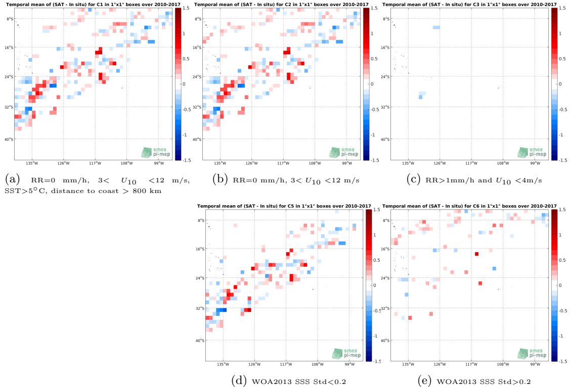
Figure 12: Temporal mean gridded over spatial boxes of size 1^{\circ}\times 1^{\circ} of \Delta\text{SSS} (SMOS SSS L3 v2 - Daily - 0.5 Deg (CATDS-CECOS-IFREMER) - TSG (LEGOS-DM)) for 5 different subdatasets corresponding to:RR=0 mm/h, 3 < U_{10} < 12 m/s, SST >5^{\circ}\text{C} , distance to coast > 800 km (a), RR=0 mm/h, 3 < U_{10} < 12 m/s (b), RR >1 mm/h and U_{10} < 4 m/s (c), WOA2013 SSS Std <0.2 (d), WOA2013 SSS Std >0.2 (e).
