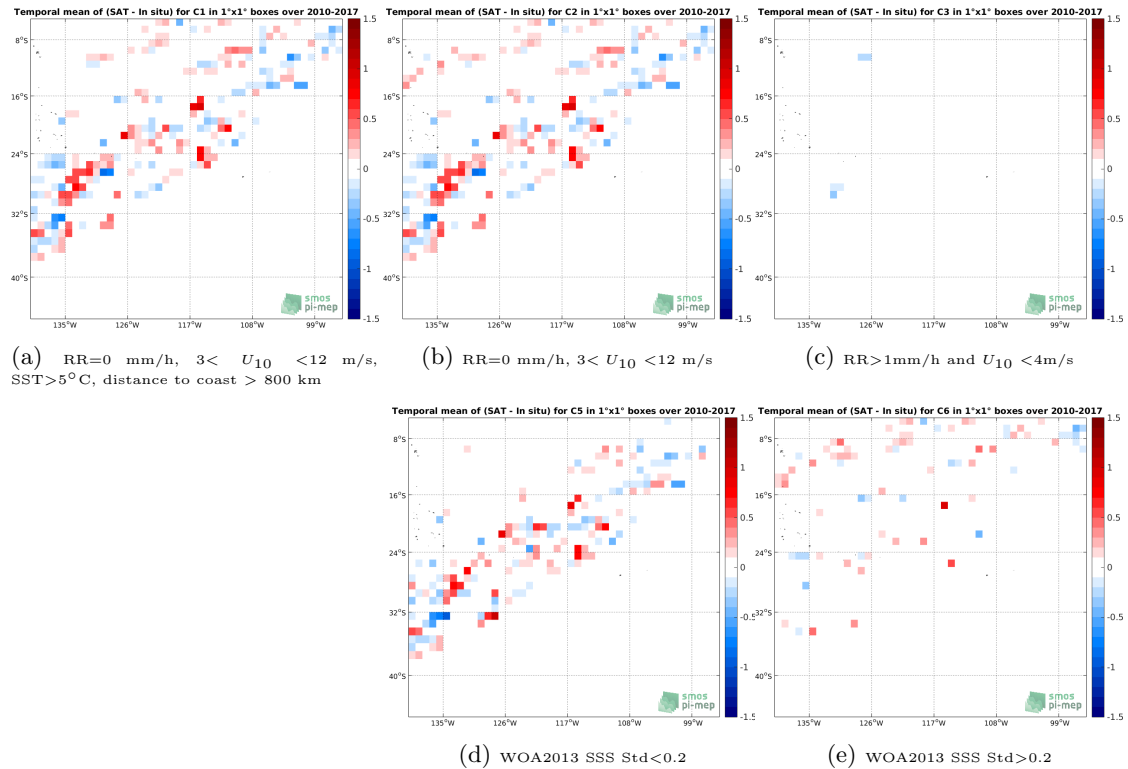
Figure 12: Temporal mean gridded over spatial boxes of size 1^{\circ}\times 1^{\circ} of \Delta\text{SSS} (SMOS L3 v2 - Daily - 0.5 Deg (CATDS-CECOS-IFREMER) - TSG-LEGOS-DM) for 5 different subdatasets corresponding to:RR=0 mm/h, 3 < U_{10} < 12 m/s, SST >5^{\circ}\text{C} , distance to coast > 800 km (a), RR=0 mm/h, 3 < U_{10} < 12 m/s (b), RR >1 mm/h and U_{10} < 4 m/s (c), WOA2013 SSS Std <0.2 (d), WOA2013 SSS Std >0.2 (e).
