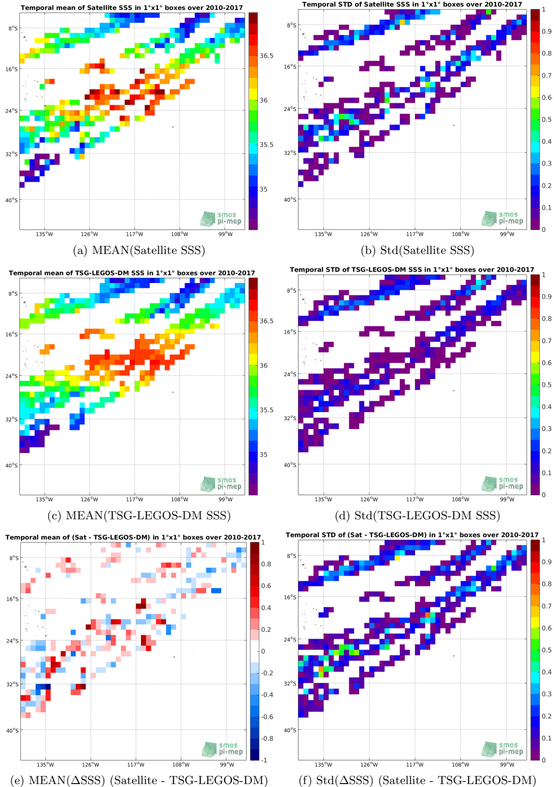
Figure 6: Temporal mean (left) and Std (right) of SSS from SMOS L3 v2 - Daily - 0.5 Deg (CATDS-CECOS-IFREMER) (top), TSG-LEGOS-DM (middle), and of \Delta SSS (Satellite - TSG-LEGOS-DM). Only match-up pairs are used to generate these maps.
