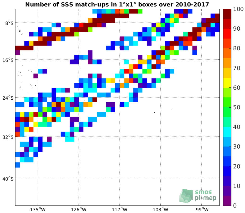
Figure 4: Number of SSS match-ups between TSG-LEGOS-DM SSS and the SMOS L3 v2 - Daily - 0.5 Deg (CATDS-CECOS-IFREMER) SSS product for the OTT zone Pi-MEP region over 1°x1° boxes and for the full satellite product period.
