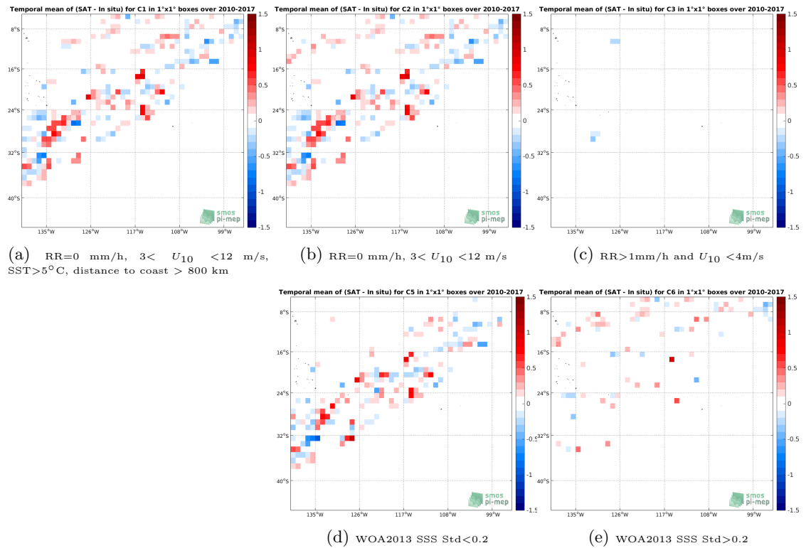
Figure 12: Temporal mean gridded over spatial boxes of size 1^\circ \times 1^\circ of \Delta SSS (SMOS-L3-CATDS-CECOS-IFREMER-V2-1DAY-0.5DEG - TSG-LEGOS-DM) for 5 different subdatasets corresponding to:RR=0 mm/h, 3 < U_{10} < 12 m/s, SST >5^\circ C, distance to coast > 800 km (a), RR=0 mm/h, 3 < U_{10} < 12 m/s (b), RR >1 mm/h and U_{10} < 4 m/s (c), WOA2013 SSS Std <0.2 (d), WOA2013 SSS Std >0.2 (e).
