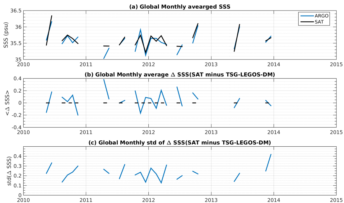
Figure 7: Time series of the monthly averaged mean SSS (top), mean \Delta SSS (Satellite - TSG-LEGOS-DM) and STD of \Delta SSS (Satellite - TSG-LEGOS-DM) over the OTT zone Pi-MEP region considering all match-ups collected by the Pi-MEP platform.
