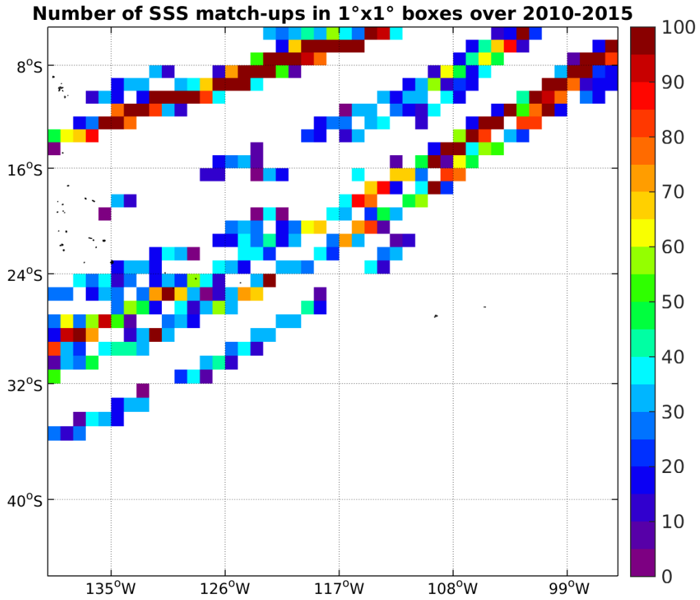
Figure 4: Number of SSS match-ups between TSG-LEGOS-DM SSS and the SMOS-L3-CATDS-CECOS-IFREMER-V2-1DAY-0.5DEG SSS product for the OTT zone Pi-MEP region over 1°x1° boxes and for the full satellite product period.
