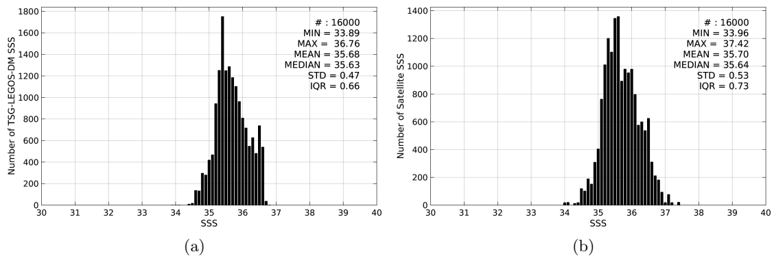
Figure 2: Histograms of SSS from TSG-LEGOS-DM (a) and SMOS-L3-CATDS-CECOS-IFREMER-V2-1DAY-0.5DEG (b) considering all match-up pairs per bins of 0.1 over the OTT zone Pi-MEP region and for the full satellite product period.
