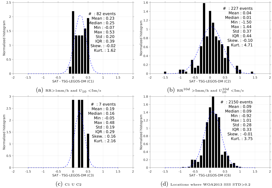
Figure 13: Normalized histogram of \Delta SSS (SMOS-L3-CATDS-CECOS-IFREMER-V2-1DAY-0.5DEG - TSG-LEGOS-DM) for 6 different subdatasets corresponding to: RR > 1mm/h and U_{10} < 5 m/s (a), RR^{10d} > 5 mm/h and U_{10}^{10d} < 5 m/s (b), C1 U C2 (c), Locations where WOA2013 SSS STD > 0.2 (d).
