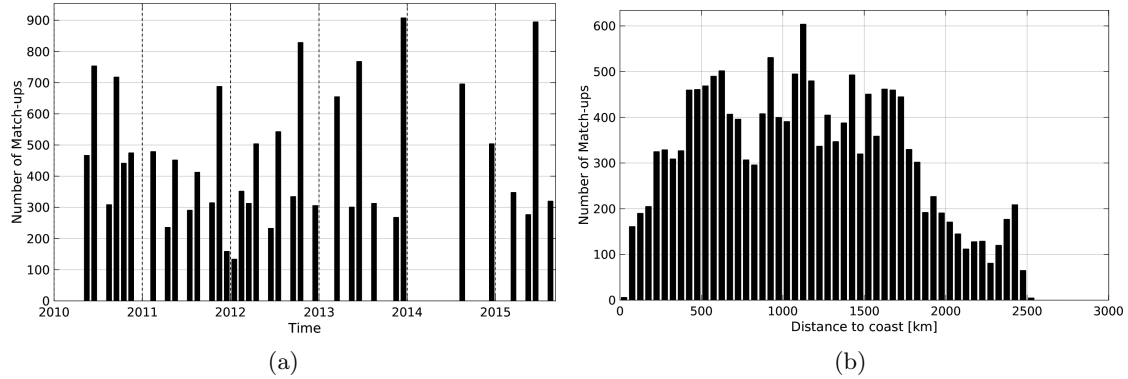
Figure 1: Number of match-ups between TSG-LEGOS-DM and SMOS-L3-CATDS-CECOS-IFREMER-V2-1DAY-0.5DEG SSS as a function of time (a) and as function of the distance to coast (b) over the OTT zone Pi-MEP region and for the full satellite product period.
