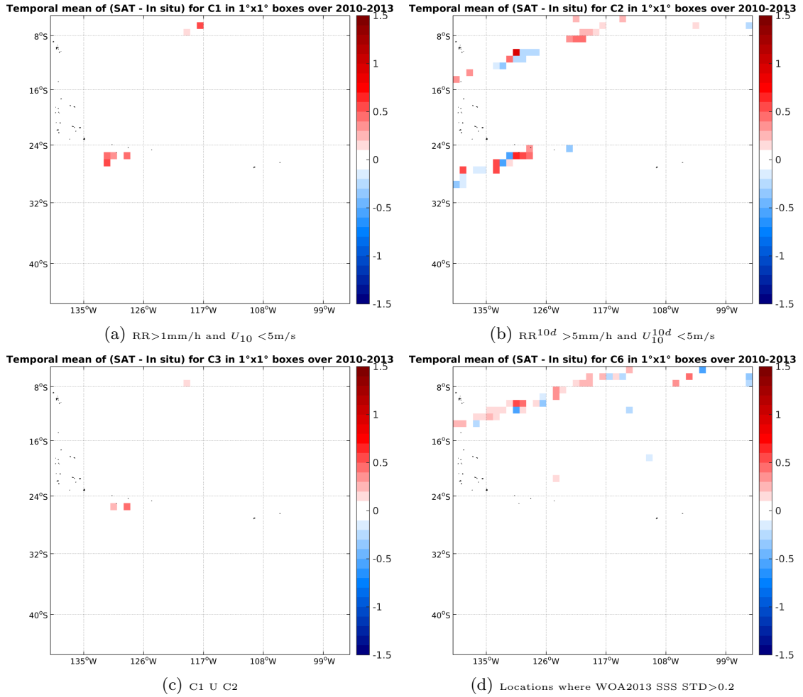
Figure 12: Temporal mean gridded over spatial boxes of size 1°x1° of \Delta SSS (SMOS-L3-CATDS-CECOS-IFREMER-V2-1DAY-0.5deg - TSG-LEGOS-DM) for 4 different subdatasets corresponding to:RR>1mm/h and U_{10} < 5 m/s (a), RR^{10d} > 5 mm/h and U_{10}^{10d} < 5 m/s (b), C1 U C2 (c),Locations where WOA2013 SSS STD>0.2 (d).
