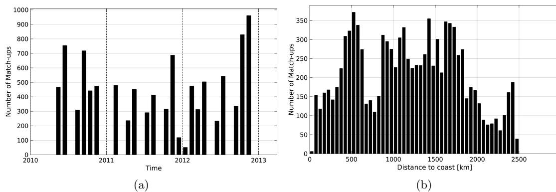
Figure 1: Number of match-ups between TSG-LEGOS-DM and SMOS-L3-CATDS-CECOS-IFREMER-V2-1DAY-0.5deg SSS as a function of time (a) and as function of the distance to coast (b) over the OTT zone Pi-MEP region and for the full satellite product period.
