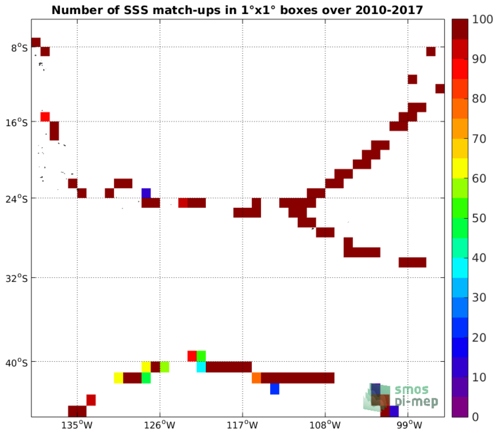
Figure 4: Number of SSS match-ups between TSG-GOSUD-Sailing-ship SSS and the SMOS L3 v2 - Daily - 0.5 Deg (CATDS-CECOS-IFREMER) SSS product for the OTT zone Pi-MEP region over 1°x1° boxes and for the full satellite product period.
