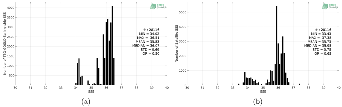
Figure 2: Histograms of SSS from TSG-GOSUD-Sailing-ship (a) and SMOS L3 v2 - Daily - 0.5 Deg (CATDS-CECOS-IFREMER) (b) considering all match-up pairs per bins of 0.1 over the OTT zone Pi-MEP region and for the full satellite product period.
