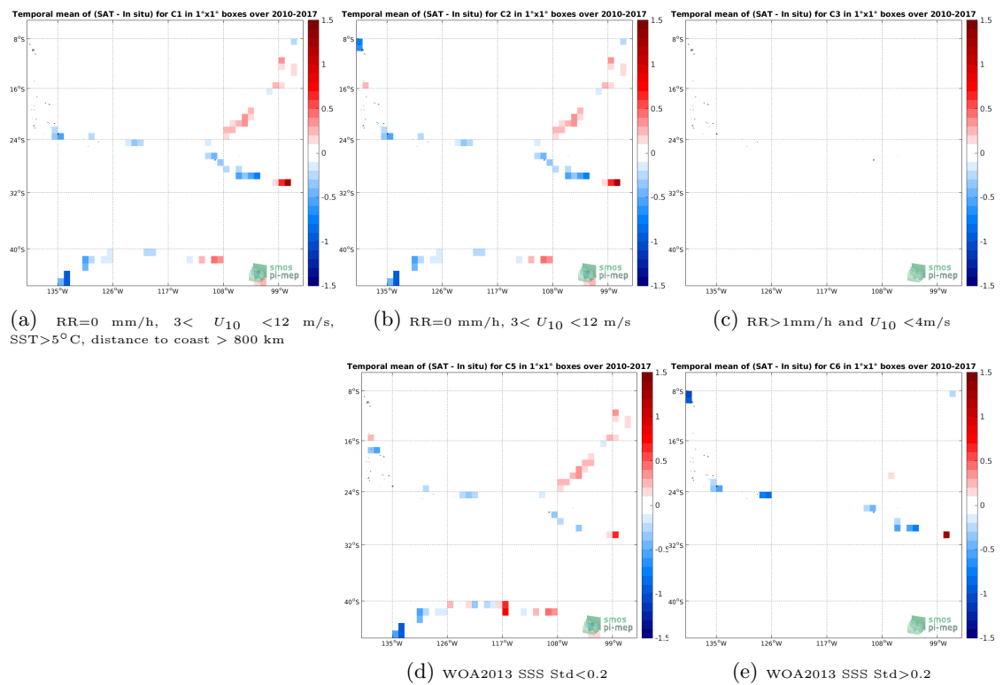
Figure 12: Temporal mean gridded over spatial boxes of size 1^\circ \times 1^\circ of \Delta SSS (SMOS L3 v2 - Daily - 0.5 Deg (CATDS-CECOS-IFREMER) - TSG-GOSUD-Sailing-ship) for 5 different subdatasets corresponding to:RR=0 mm/h, 3 < U_{10} < 12 m/s, SST >5^\circ\text{C} , distance to coast > 800 km (a), RR=0 mm/h, 3 < U_{10} < 12 m/s (b), RR >1 mm/h and U_{10} < 4 m/s (c), WOA2013 SSS Std <0.2 (d), WOA2013 SSS Std >0.2 (e).
