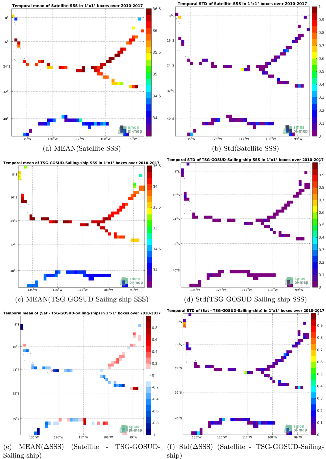
Figure 6: Temporal mean (left) and Std (right) of SSS from SMOS L3 v2 - Daily - 0.5 Deg (CATDS-CECOS-IFREMER) (top), TSG-GOSUD-Sailing-ship (middle), and of \Delta SSS (Satellite - TSG-GOSUD-Sailing-ship). Only match-up pairs are used to generate these maps.
