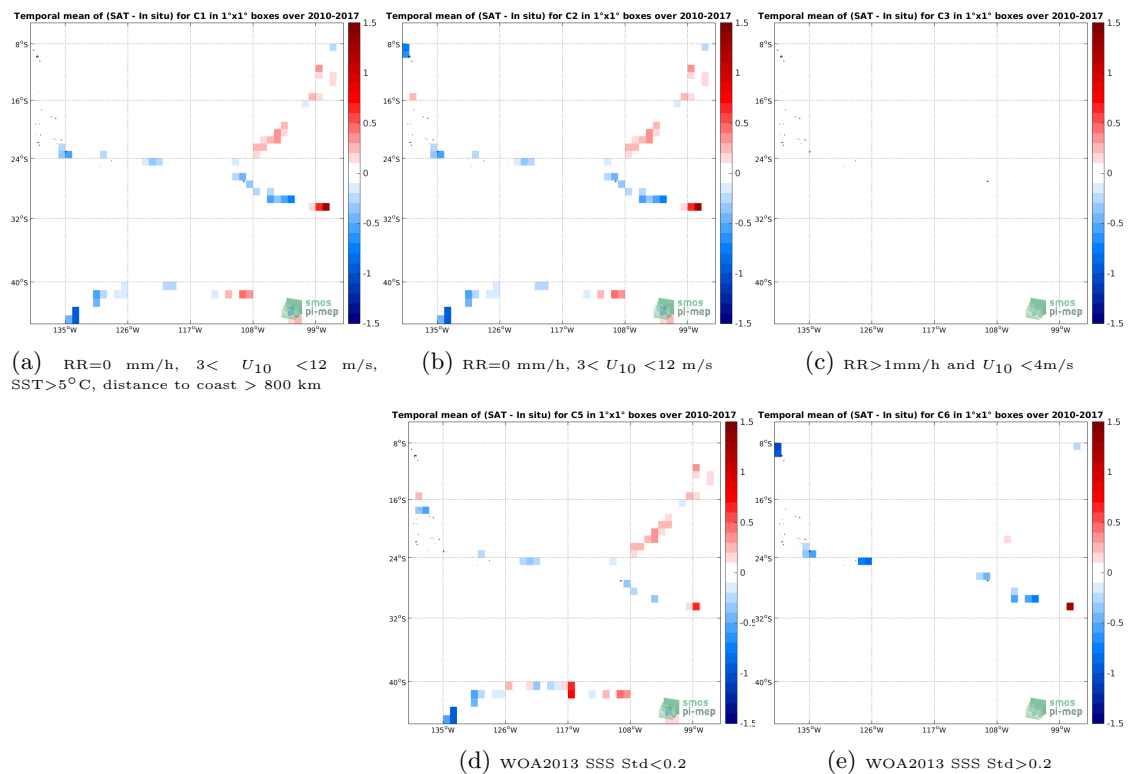
Figure 12: Temporal mean gridded over spatial boxes of size 1^\circ \times 1^\circ of \Delta SSS (SMOS-L3-CATDS-CECOS-IFREMER-V2-1DAY-0.5DEG - TSG-GOSUD-Sailing-ship) for 5 different subdatasets corresponding to:RR=0 mm/h, 3 < U_{10} < 12 m/s, SST >5^\circ\text{C} , distance to coast > 800 km (a), RR=0 mm/h, 3 < U_{10} < 12 m/s (b), RR >1 mm/h and U_{10} < 4 m/s (c), WOA2013 SSS Std <0.2 (d), WOA2013 SSS Std >0.2 (e).
