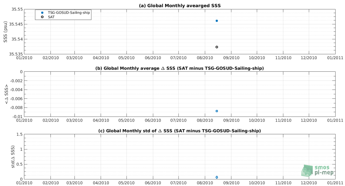
Figure 7: Time series of the monthly averaged mean SSS (top), mean \Delta SSS (Satellite - TSG-GOSUD-Sailing-ship) and STD of \Delta SSS (Satellite - TSG-GOSUD-Sailing-ship) over the OTT zone Pi-MEP region considering all match-ups collected by the Pi-MEP platform.
