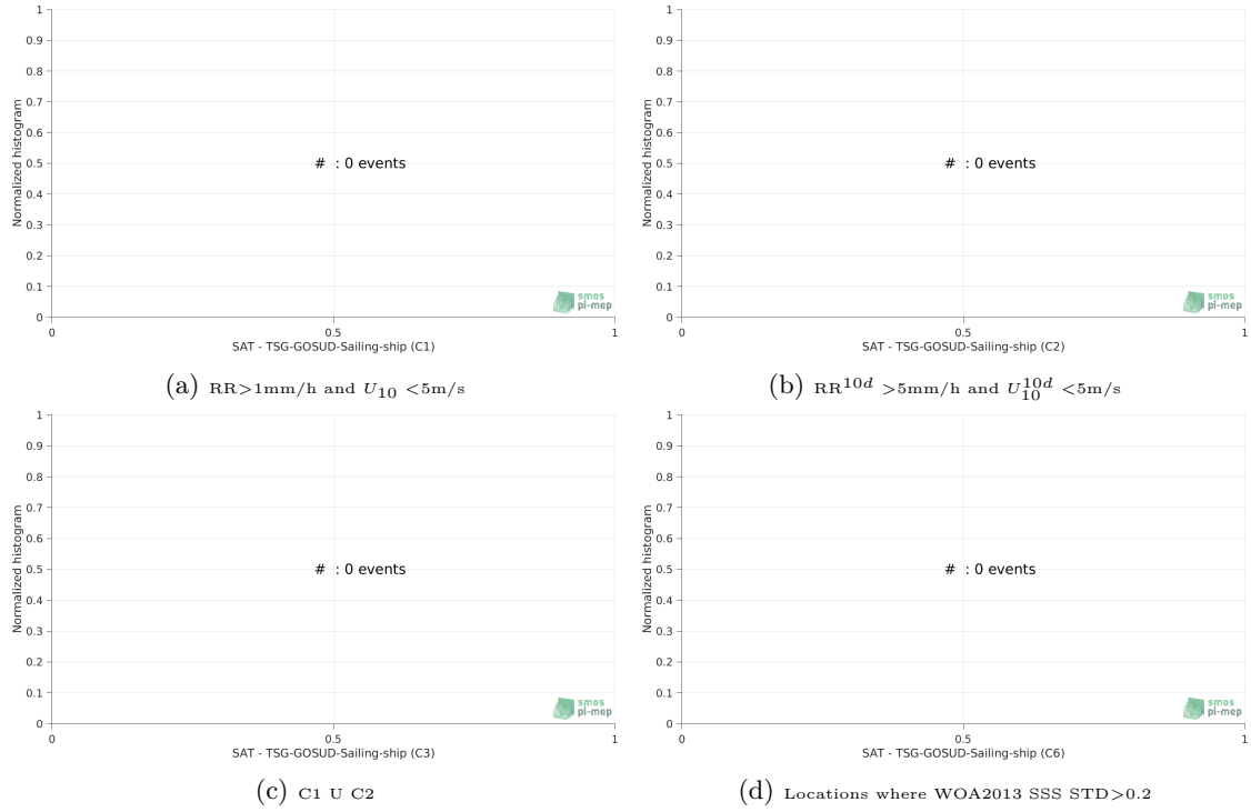
Figure 13: Normalized histogram of \Delta\text{SSS} (SMOS-L3-CATDS-CECOS-IFREMER-V2-1DAY-0.5DEG - TSG-GOSUD-Sailing-ship) for 6 different subdatasets corresponding to: RR > 1\text{mm/h} and U_{10} < 5\text{m/s} (a), RR^{10d} > 5\text{mm/h} and U_{10}^{10d} < 5\text{m/s} (b), C1 \cup C2 (c), Locations where WOA2013 SSS STD > 0.2 (d).
