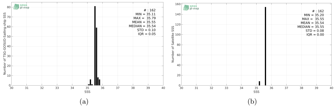
Figure 2: Histograms of SSS from TSG-GOSUD-Sailing-ship (a) and SMOS-L3-CATDS-CECOS-IFREMER-V2-1DAY-0.5DEG (b) considering all match-up pairs per bins of 0.1 over the OTT zone Pi-MEP region and for the full satellite product period.
