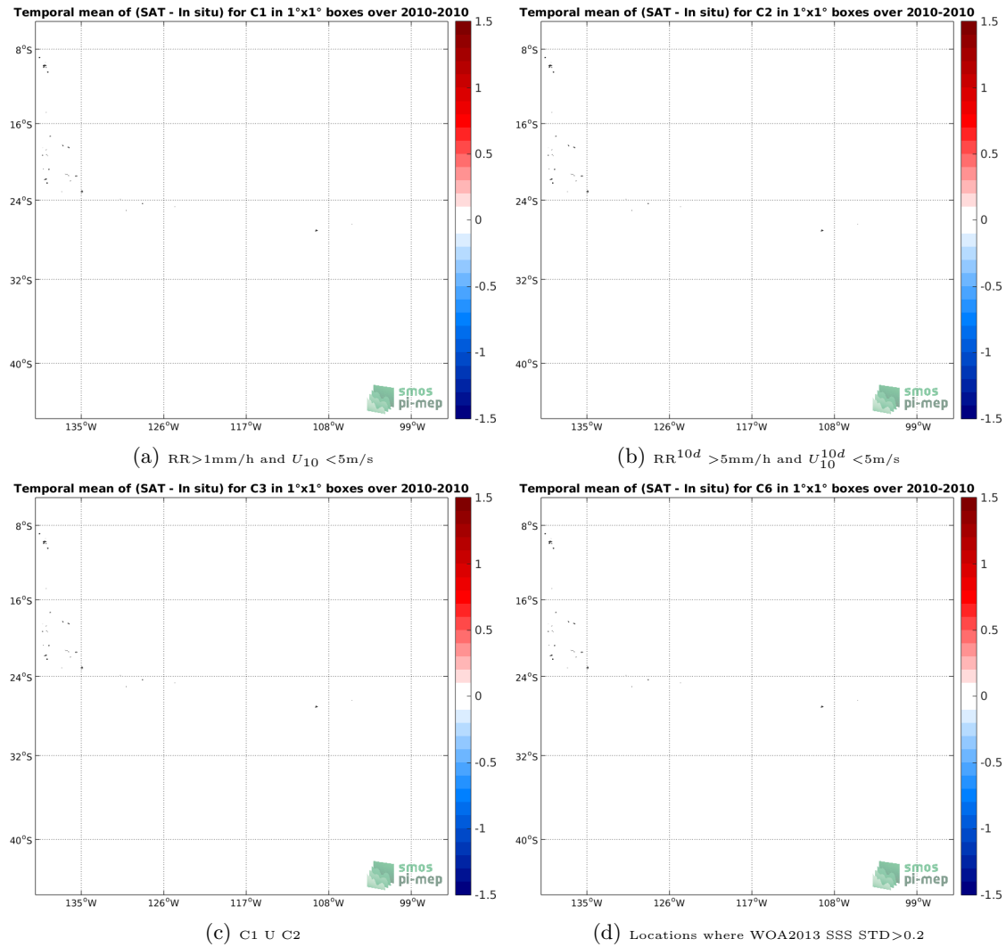
Figure 12: Temporal mean gridded over spatial boxes of size 1^\circ \times 1^\circ of \Delta SSS (SMOS-L3-CATDS-CECOS-IFREMER-V2-1DAY-0.5DEG - TSG-GOSUD-Sailing-ship) for 4 different subdatasets corresponding to: RR > 1\text{mm/h} and U_{10} < 5\text{m/s} (a), RR^{10d} > 5\text{mm/h} and U_{10}^{10d} < 5\text{m/s} (b), C1 U C2 (c), Locations where WOA2013 SSS STD > 0.2 (d).
