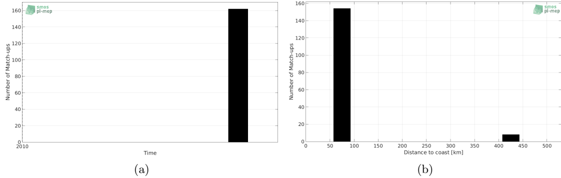
Figure 1: Number of match-ups between TSG-GOSUD-Sailing-ship and SMOS-L3-CATDS-CECOS-IFREMER-V2-1DAY-0.5DEG SSS as a function of time (a) and as function of the distance to coast (b) over the OTT zone Pi-MEP region and for the full satellite product period.
