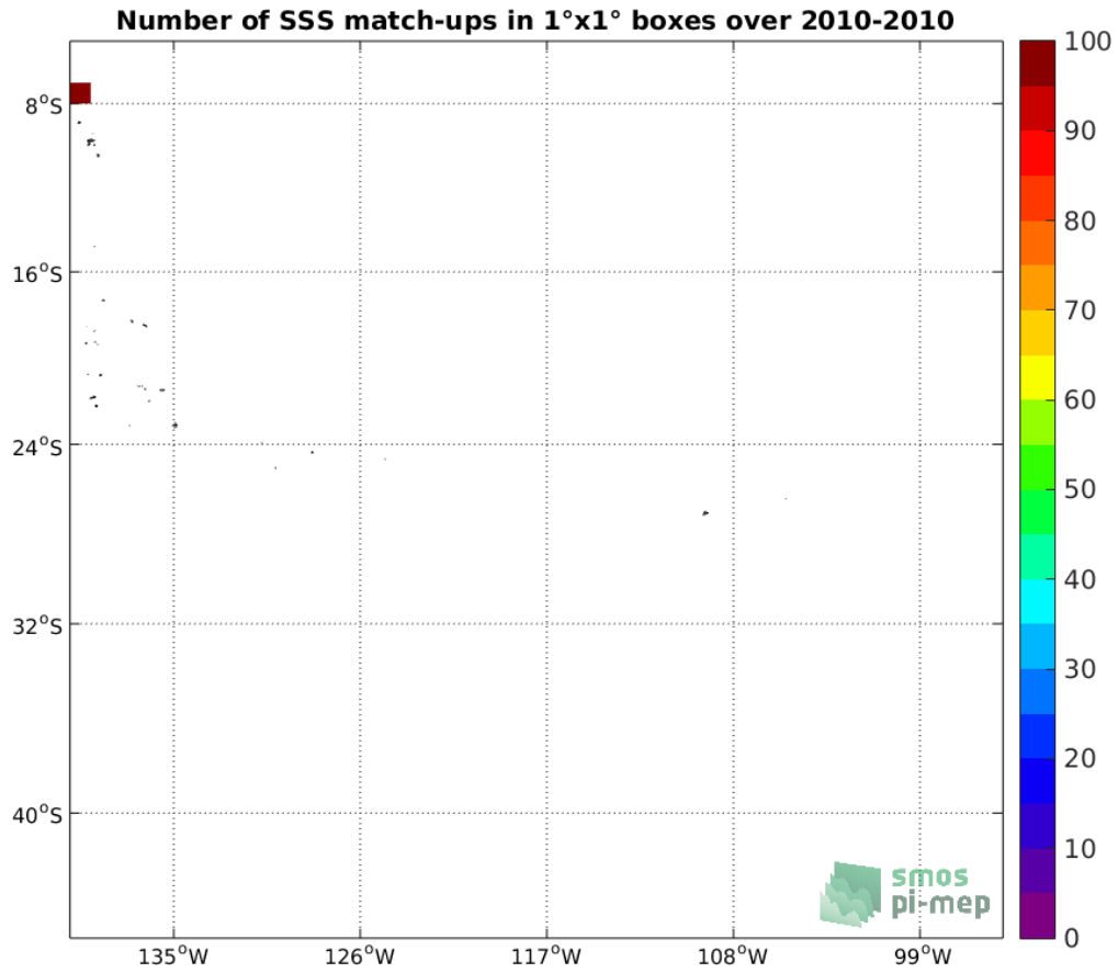
Figure 4: Number of SSS match-ups between TSG-GOSUD-Sailing-ship SSS and the SMOS-L3-CATDS-CECOS-IFREMER-V2-1DAY-0.5DEG SSS product for the OTT zone Pi-MEP region over 1°x1° boxes and for the full satellite product period.
