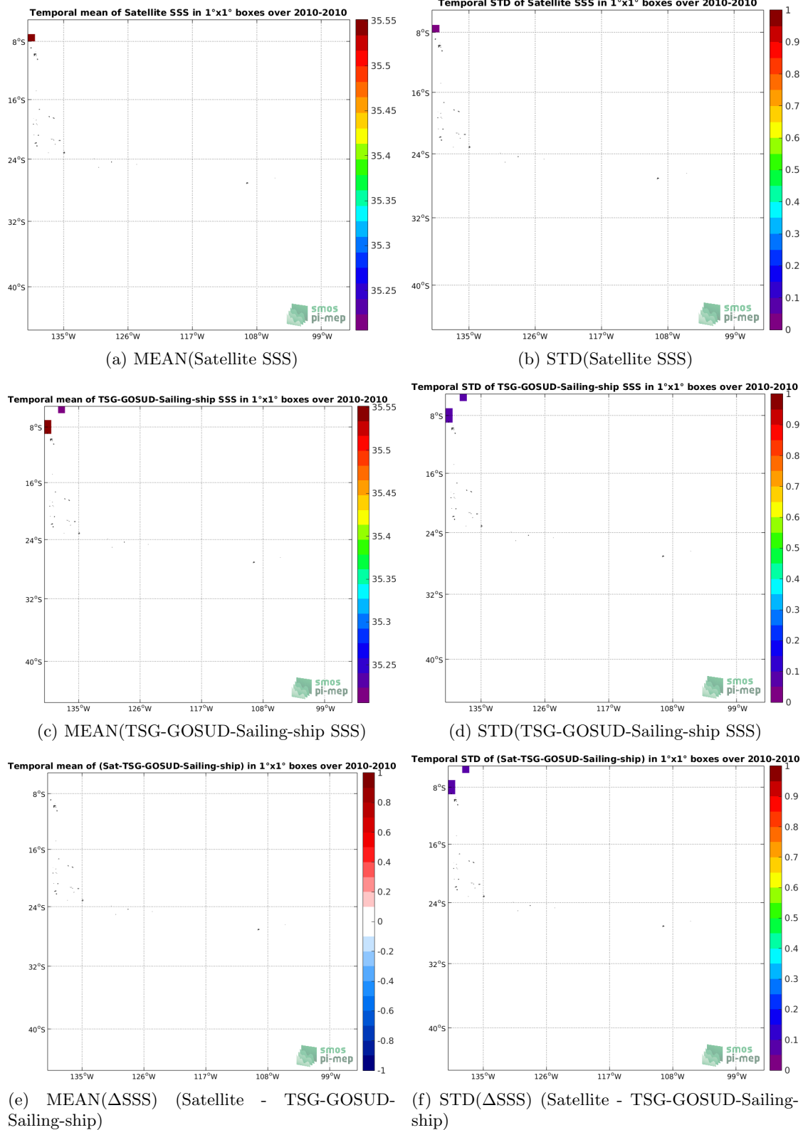
Figure 6: Temporal mean (left) and STD (right) of SSS from SMOS-L3-CATDS-CECOS-IFREMER-V2-1DAY-0.5DEG (top), TSG-GOSUD-Sailing-ship (middle), and of \Delta SSS (Satellite - TSG-GOSUD-Sailing-ship). Only match-up pairs are used to generate these maps.
