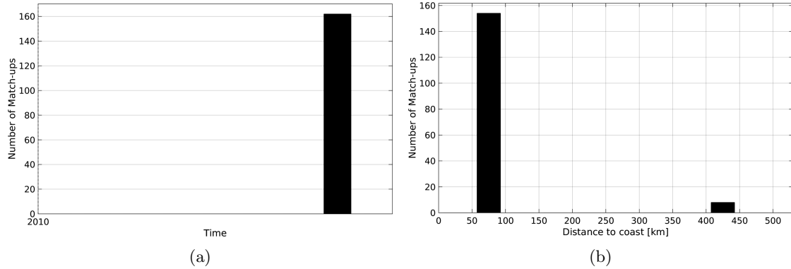
Figure 1: Number of match-ups between TSG-GOSUD-Sailing-ship and SMOS-L3-CATDS-CECOS-IFREMER-V2-1DAY-0.5DEG SSS as a function of time (a) and as function of the distance to coast (b) over the OTT zone Pi-MEP region and for the full satellite product period.
