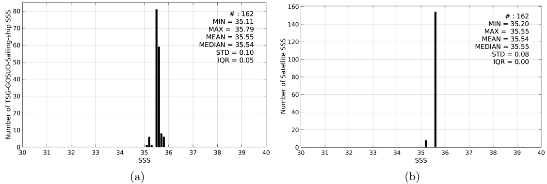
Figure 2: Histograms of SSS from TSG-GOSUD-Sailing-ship (a) and SMOS-L3-CATDS-CECOS-IFREMER-V2-1DAY-0.5deg (b) considering all match-up pairs per bins of 0.1 over the OTT zone Pi-MEP region and for the full satellite product period.
