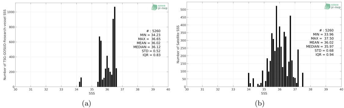
Figure 2: Histograms of SSS from TSG-GOSUD-Research-vessel (a) and SMOS L3 v2 - Daily - 0.5 Deg (CATDS-CECOS-IFREMER) (b) considering all match-up pairs per bins of 0.1 over the OTT zone Pi-MEP region and for the full satellite product period.
