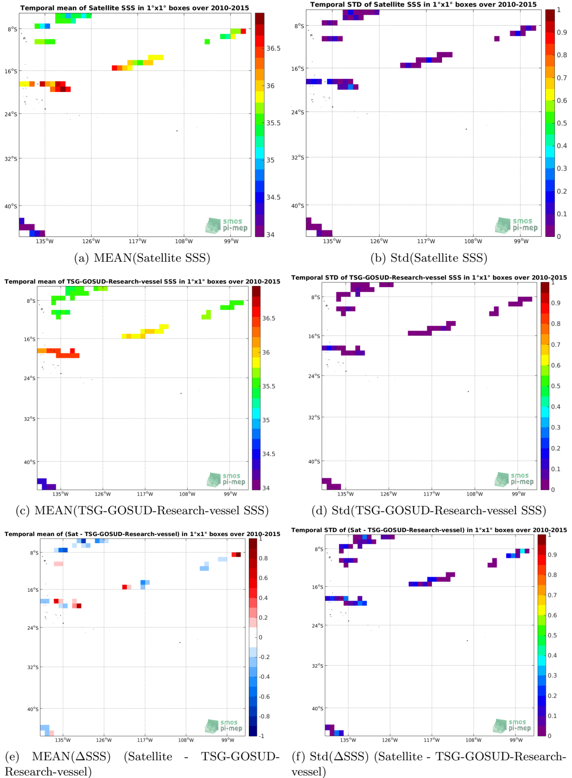
Figure 6: Temporal mean (left) and Std (right) of SSS from SMOS L3 v2 - Daily - 0.5 Deg (CATDS-CECOS-IFREMER) (top), TSG-GOSUD-Research-vessel (middle), and of \Delta SSS (Satellite - TSG-GOSUD-Research-vessel). Only match-up pairs are used to generate these maps.
