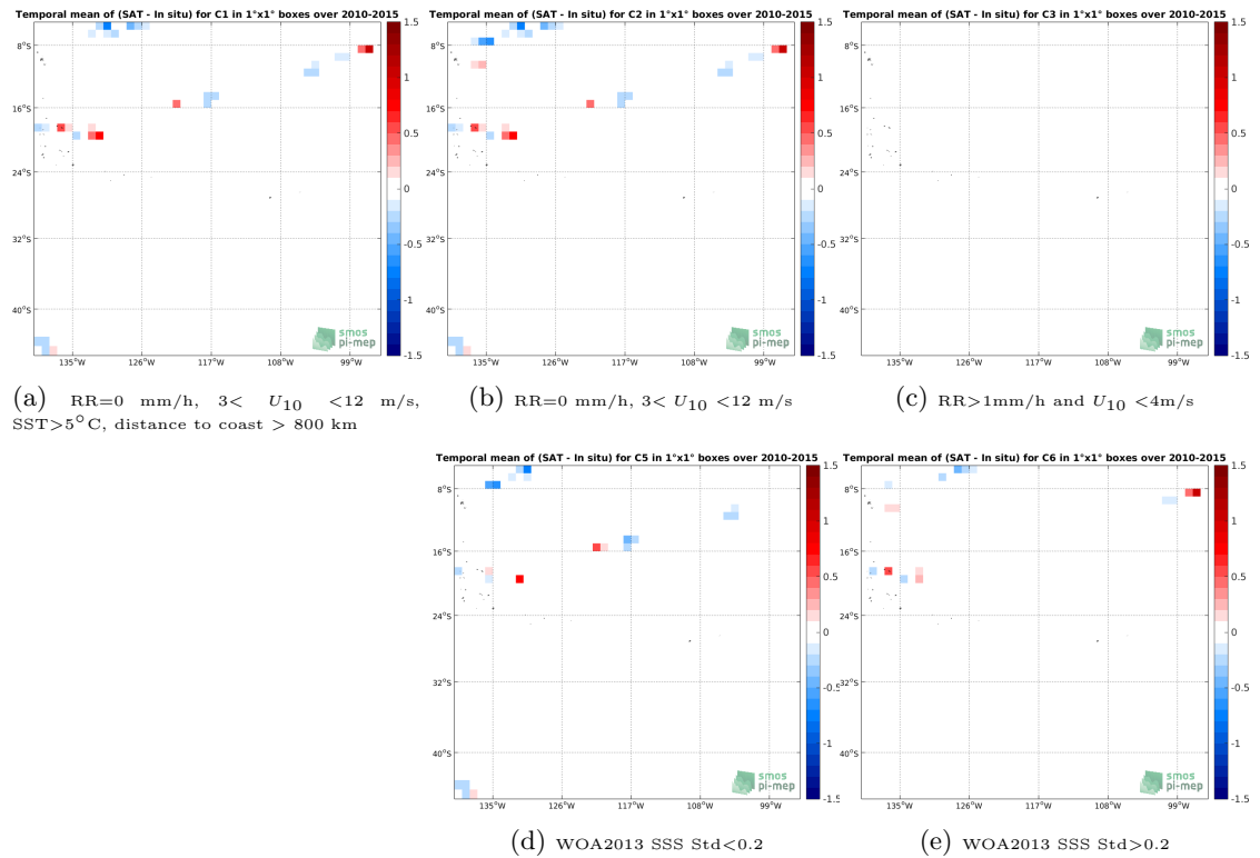
Figure 12: Temporal mean gridded over spatial boxes of size 1^\circ \times 1^\circ of \Delta SSS (SMOS L3 v2 - Daily - 0.5 Deg (CATDS-CECOS-IFREMER) - TSG-GOSUD-Research-vessel) for 5 different subdatasets corresponding to: RR=0 mm/h, 3 < U_{10} < 12 m/s, SST > 5^\circ\text{C} , distance to coast > 800 km (a), RR=0 mm/h, 3 < U_{10} < 12 m/s (b), RR > 1 mm/h and U_{10} < 4 m/s (c), WOA2013 SSS Std < 0.2 (d), WOA2013 SSS Std > 0.2 (e).
