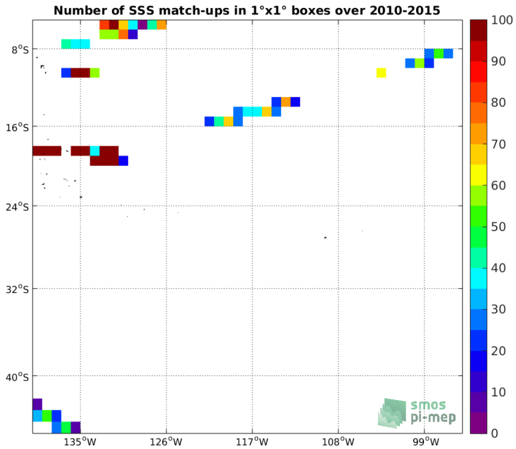
Figure 4: Number of SSS match-ups between TSG-GOSUD-Research-vessel SSS and the SMOS L3 v2 - Daily - 0.5 Deg (CATDS-CECOS-IFREMER) SSS product for the OTT zone Pi-MEP region over 1°x1° boxes and for the full satellite product period.
