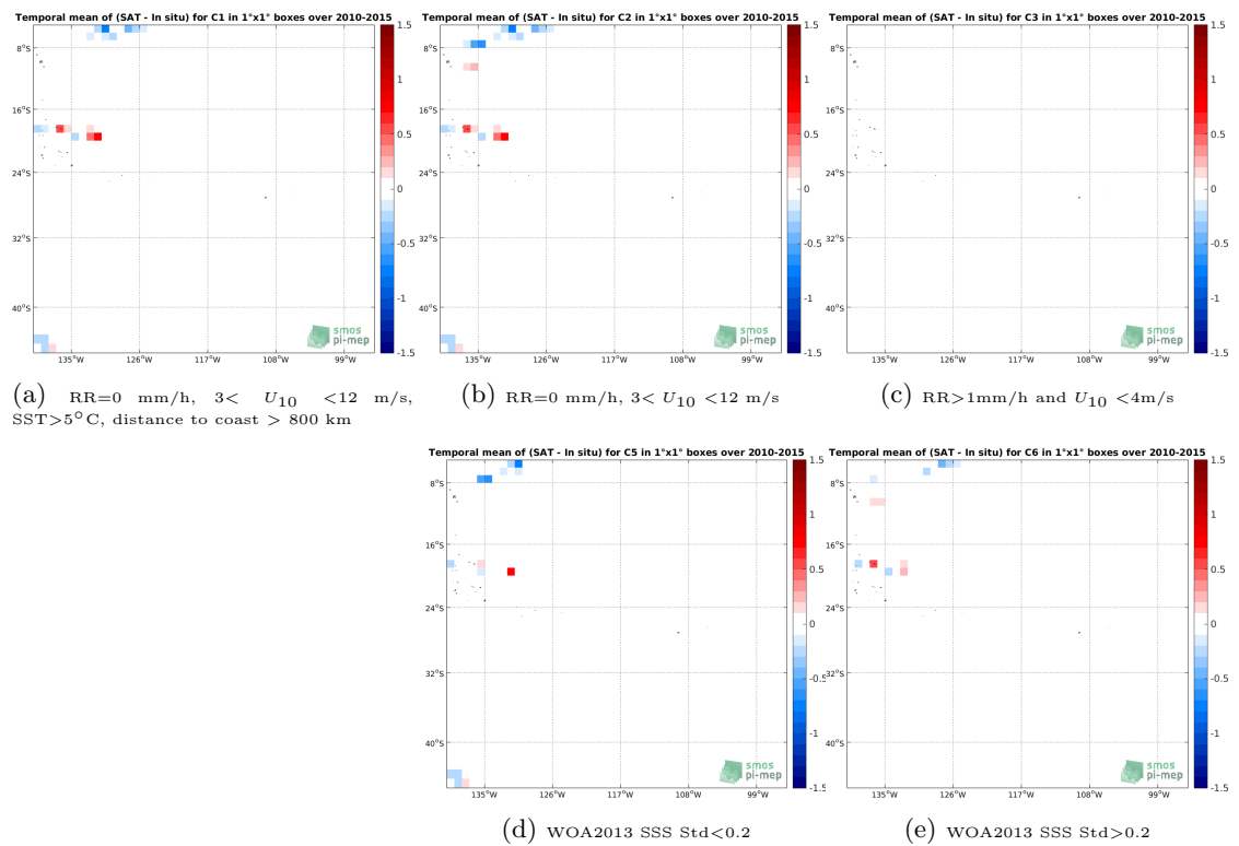
Figure 12: Temporal mean gridded over spatial boxes of size 1^\circ \times 1^\circ of \Delta SSS (SMOS-L3-CATDS-CECOS-IFREMER-V2-1DAY-0.5DEG - TSG-GOSUD-Research-vessel) for 5 different subdatasets corresponding to:RR=0 mm/h, 3 < U_{10} < 12 m/s, SST >5^\circ\text{C} , distance to coast > 800 km (a), RR=0 mm/h, 3 < U_{10} < 12 m/s (b), RR >1 mm/h and U_{10} < 4 m/s (c), WOA2013 SSS Std <0.2 (d), WOA2013 SSS Std >0.2 (e).
