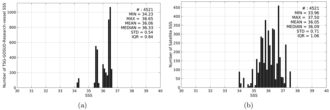
Figure 2: Histograms of SSS from TSG-GOSUD-Research-vessel (a) and SMOS-L3-CATDS-CECOS-IFREMER-V2-1DAY-0.5DEG (b) considering all match-up pairs per bins of 0.1 over the OTT zone Pi-MEP region and for the full satellite product period.
