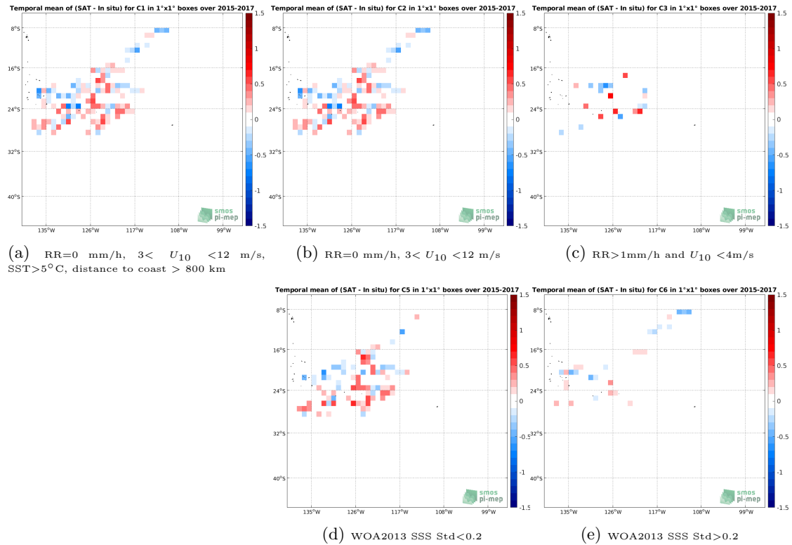
Figure 11: Temporal mean gridded over spatial boxes of size 1^{\circ}\times 1^{\circ} of \Delta\text{SSS} (SMOS SSS L3 v2 - Daily - 0.5 Deg (CATDS-CECOS-IFREMER) - Surface drifters) for 5 different subdatasets corresponding to:RR=0 mm/h, 3 < U_{10} < 12 m/s, SST >5^{\circ}\text{C} , distance to coast > 800 km (a), RR=0 mm/h, 3 < U_{10} < 12 m/s (b), RR >1 mm/h and U_{10} < 4 m/s (c), WOA2013 SSS Std <0.2 (d), WOA2013 SSS Std >0.2 (e).
