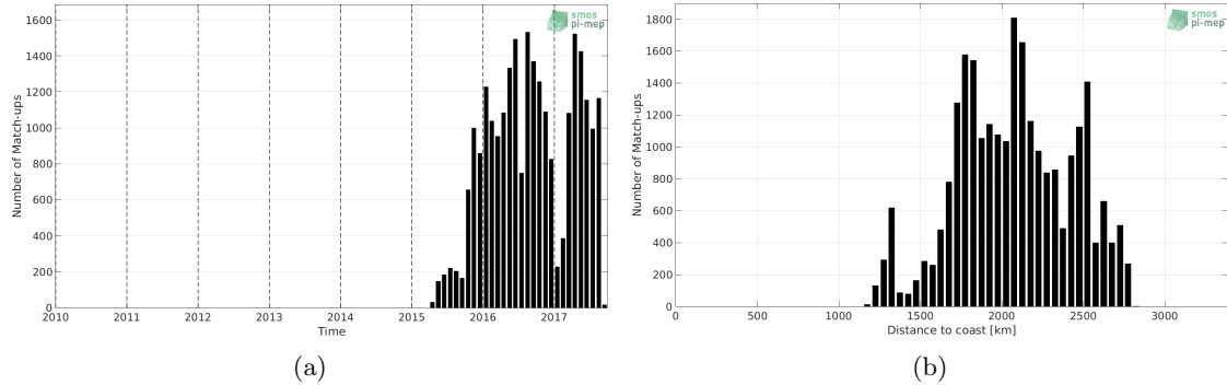
Figure 1: Number of match-ups between Surface drifters and SMOS L3 v2 - Daily - 0.5 Deg (CATDS-CECOS-IFREMER) SSS as a function of time (a) and as function of the distance to coast (b) over the OTT zone Pi-MEP region and for the full satellite product period.
