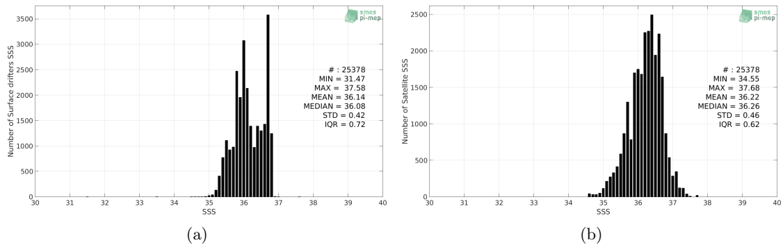
Figure 2: Histograms of SSS from Surface drifters (a) and SMOS L3 v2 - Daily - 0.5 Deg (CATDS-CECOS-IFREMER) (b) considering all match-up pairs per bins of 0.1 over the OTT zone Pi-MEP region and for the full satellite product period.
