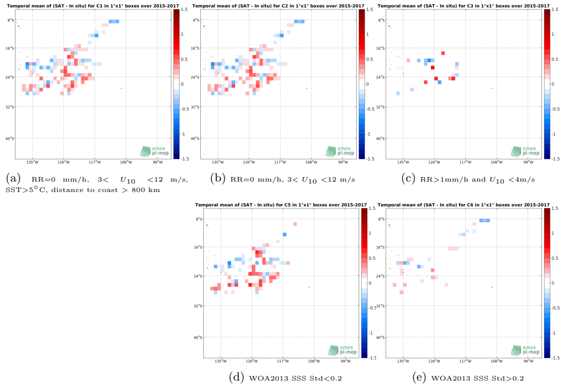
Figure 11: Temporal mean gridded over spatial boxes of size 1^{\circ}\times 1^{\circ} of \Delta\text{SSS} (SMOS L3 v2 - Daily - 0.5 Deg (CATDS-CECOS-IFREMER) - Surface drifters) for 5 different subdatasets corresponding to:RR=0 mm/h, 3 < U_{10} < 12 m/s, SST >5^{\circ}\text{C} , distance to coast > 800 km (a), RR=0 mm/h, 3 < U_{10} < 12 m/s (b), RR >1 mm/h and U_{10} < 4 m/s (c), WOA2013 SSS Std <0.2 (d), WOA2013 SSS Std >0.2 (e).
