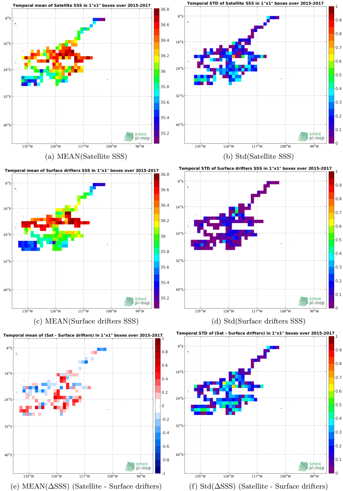
Figure 5: Temporal mean (left) and Std (right) of SSS from SMOS L3 v2 - Daily - 0.5 Deg (CATDS-CECOS-IFREMER) (top), Surface drifters (middle), and of \Delta SSS (Satellite - Surface drifters). Only match-up pairs are used to generate these maps.
