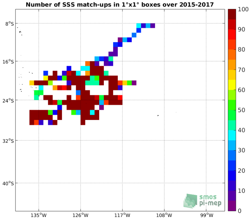
Figure 3: Number of SSS match-ups between Surface drifters SSS and the SMOS L3 v2 - Daily - 0.5 Deg (CATDS-CECOS-IFREMER) SSS product for the OTT zone Pi-MEP region over 1°x1° boxes and for the full satellite product period.
