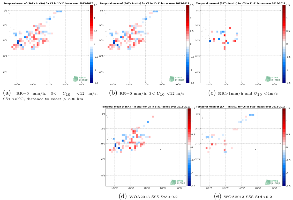
Figure 11: Temporal mean gridded over spatial boxes of size 1^\circ \times 1^\circ of \Delta SSS (SMOS-L3-CATDS-CECOS-IFREMER-V2-1DAY-0.5DEG - Surface drifters) for 5 different subdatasets corresponding to: RR=0 mm/h, 3 < U_{10} < 12 m/s, SST > 5^\circ\text{C} , distance to coast > 800 km (a), RR=0 mm/h, 3 < U_{10} < 12 m/s (b), RR > 1 mm/h and U_{10} < 4 m/s (c), WOA2013 SSS Std < 0.2 (d), WOA2013 SSS Std > 0.2 (e).
