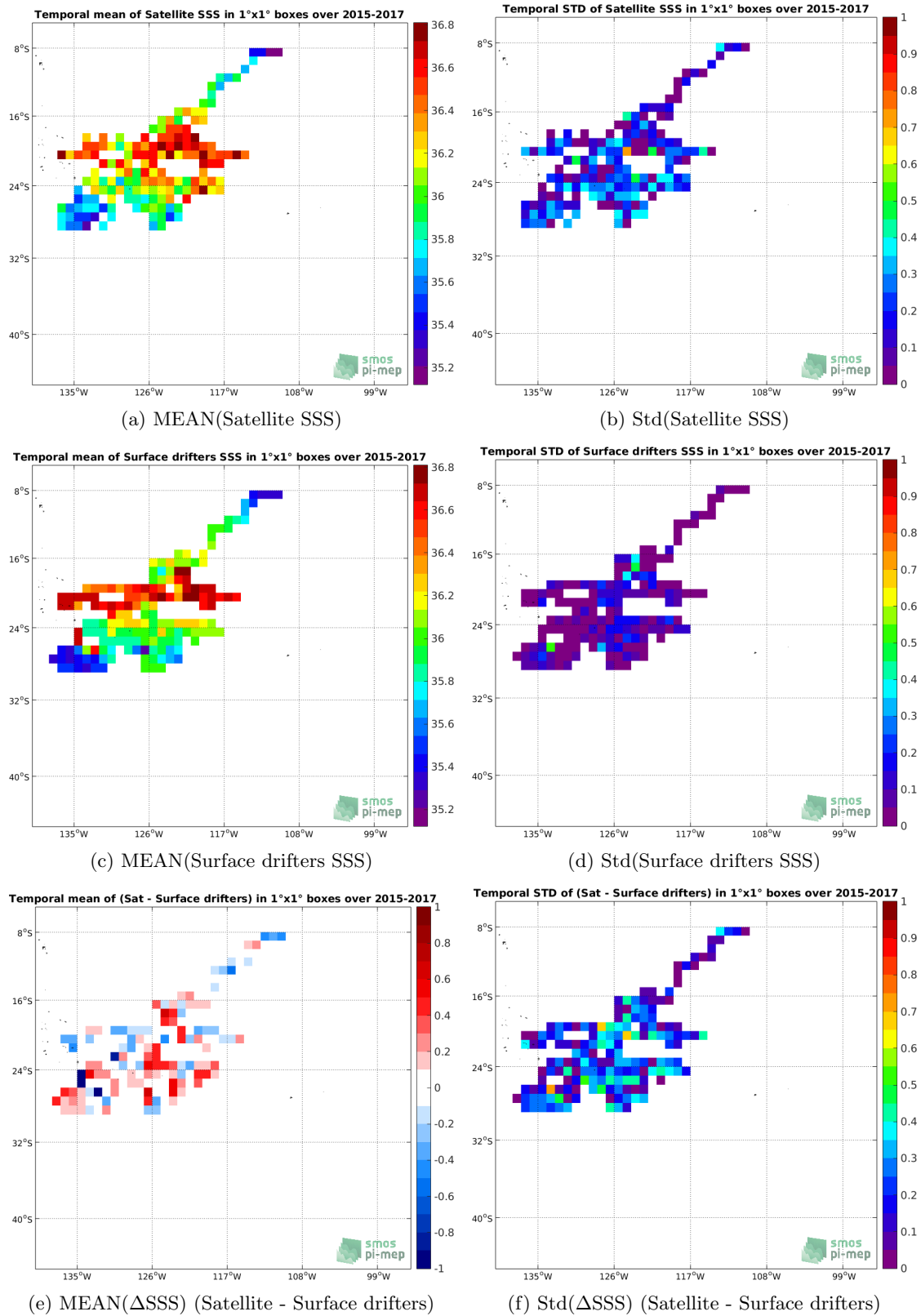
Figure 5: Temporal mean (left) and Std (right) of SSS from SMOS-L3-CATDS-CECOS-IFREMER-V2-1DAY-0.5DEG (top), Surface drifters (middle), and of \Delta SSS (Satellite - Surface drifters). Only match-up pairs are used to generate these maps.
