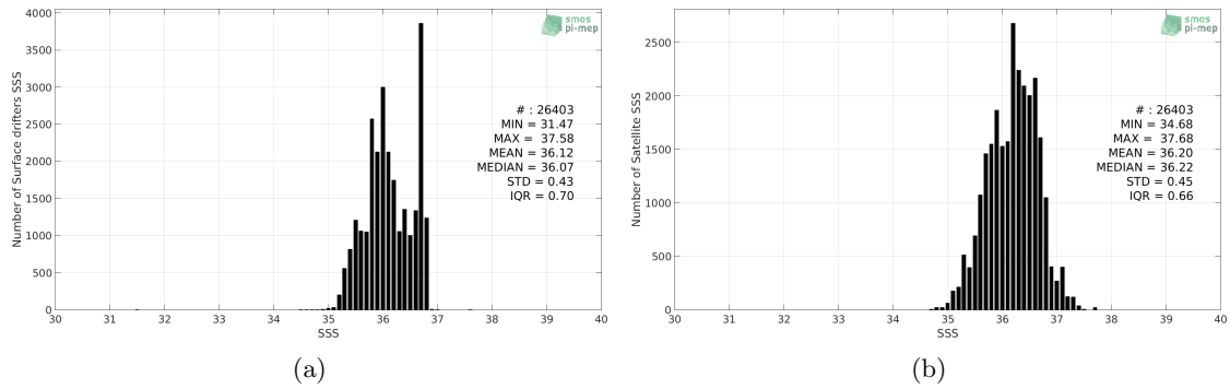
Figure 2: Histograms of SSS from Surface drifters (a) and SMOS-L3-CATDS-CECOS-IFREMER-V2-1DAY-0.5DEG (b) considering all match-up pairs per bins of 0.1 over the OTT zone Pi-MEP region and for the full satellite product period.
