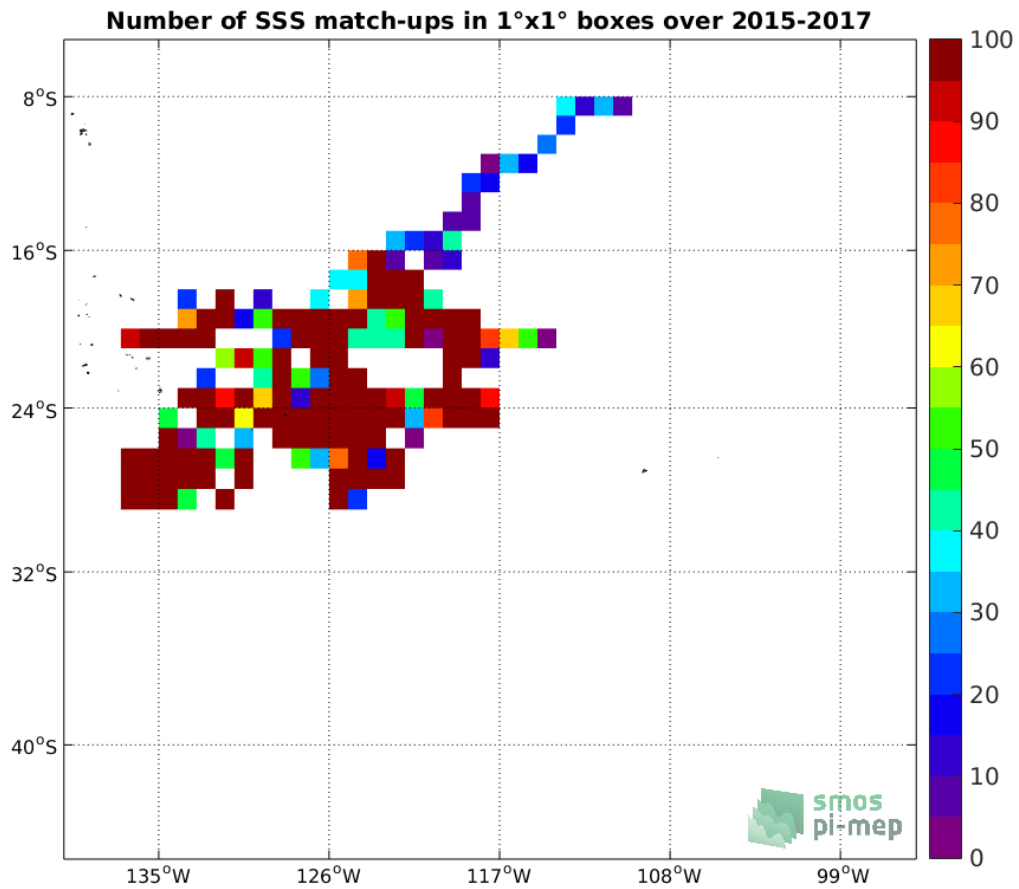
Figure 3: Number of SSS match-ups between Surface drifters SSS and the SMOS-L3-CATDS-CECOS-IFREMER-V2-1DAY-0.5DEG SSS product for the OTT zone Pi-MEP region over 1°x1° boxes and for the full satellite product period.
