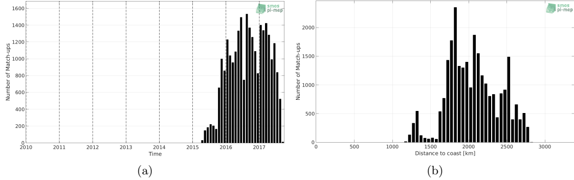
Figure 1: Number of match-ups between Surface drifters and SMOS-L3-CATDS-CECOS-IFREMER-V2-1DAY-0.5DEG SSS as a function of time (a) and as function of the distance to coast (b) over the OTT zone Pi-MEP region and for the full satellite product period.
