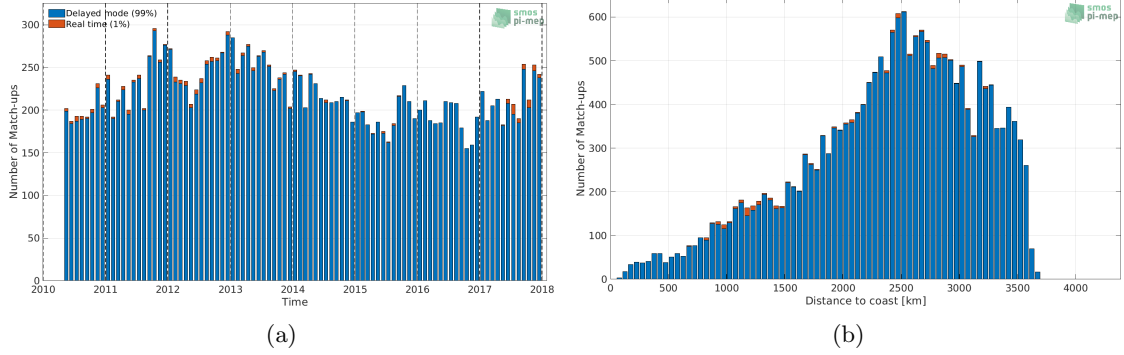
Figure 1: Number of match-ups between Argo and SMOS SSS L3 v2 - Daily - 0.5 Deg (CATDS-CECOS-IFREMER) SSS as a function of time (a) and as function of the distance to coast (b) over the OTT zone Pi-MEP region and for the full satellite product period.
