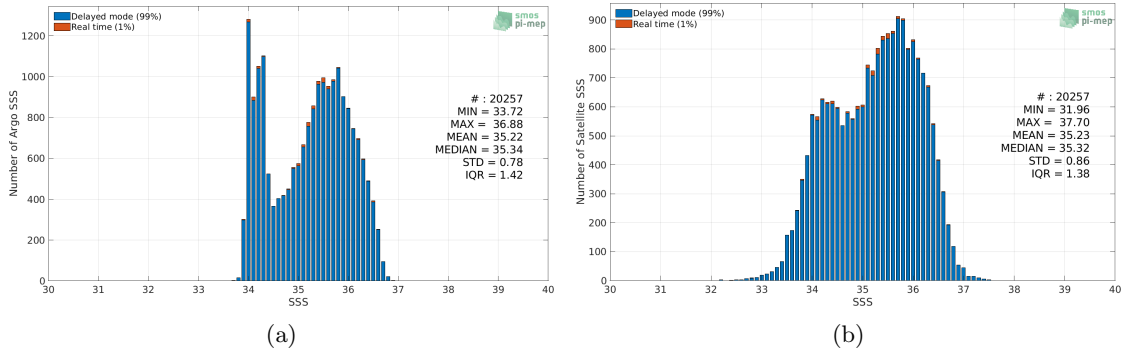
Figure 2: Histograms of SSS from Argo (a) and SMOS SSS L3 v2 - Daily - 0.5 Deg (CATDS-CECOS-IFREMER) (b) considering all match-up pairs per bins of 0.1 over the OTT zone Pi-MEP region and for the full satellite product period.
