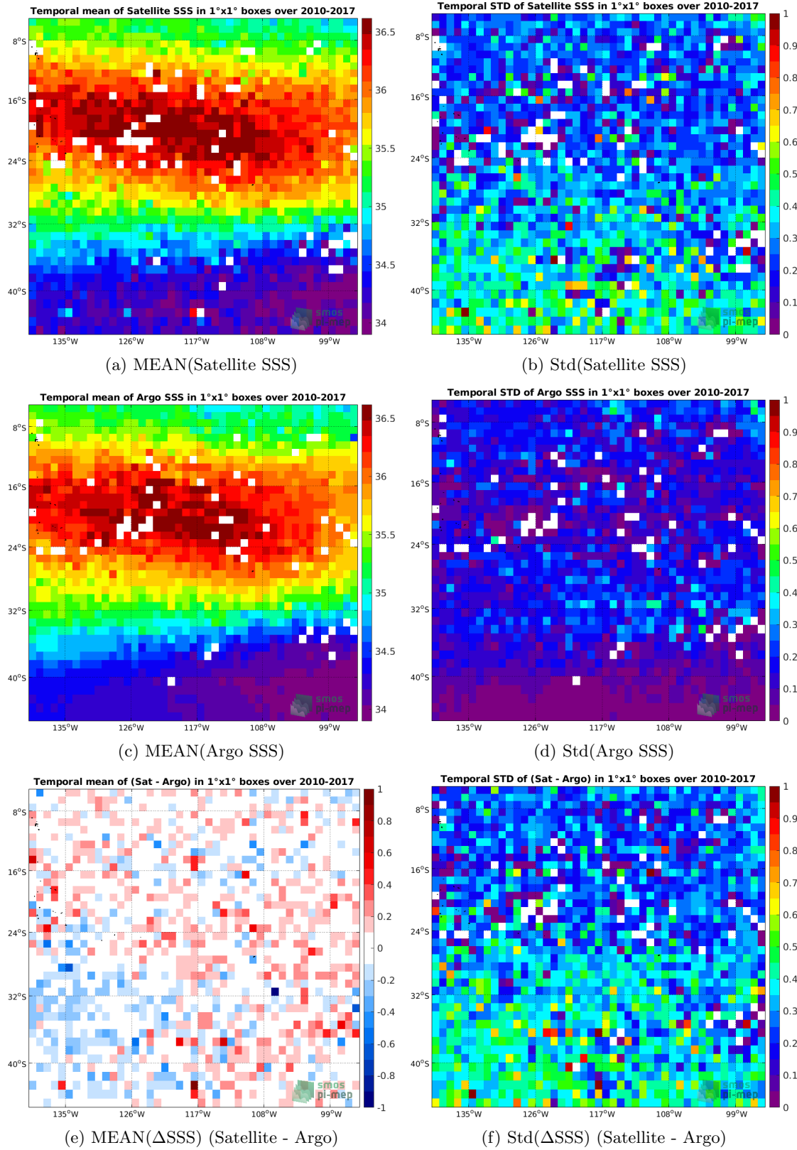
Figure 6: Temporal mean (left) and Std (right) of SSS from SMOS SSS L3 v2 - Daily - 0.5 Deg (CATDS-CECOS-IFREMER) (top), Argo (middle), and of \Delta SSS (Satellite - Argo). Only match-up pairs are used to generate these maps.
