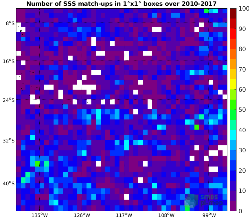
Figure 4: Number of SSS match-ups between Argo SSS and the SMOS SSS L3 v2 - Daily - 0.5 Deg (CATDS-CECOS-IFREMER) SSS product for the OTT zone Pi-MEP region over 1°x1° boxes and for the full satellite product period.
