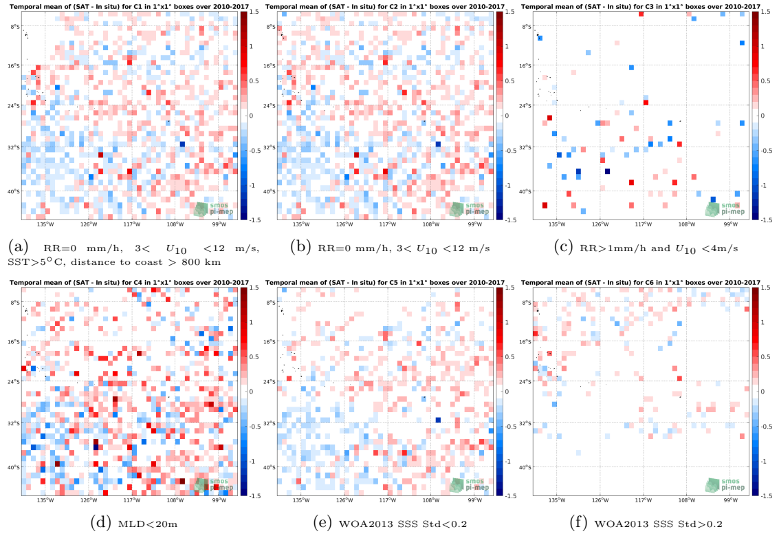
Figure 12: Temporal mean gridded over spatial boxes of size 1^\circ \times 1^\circ of \Delta SSS (SMOS SSS L3 v2 - Daily - 0.5 Deg (CATDS-CECOS-IFREMER) - Argo) for 6 different subdatasets corresponding to:RR=0 mm/h, 3 < U_{10} < 12 m/s, SST >5^\circ\text{C} , distance to coast > 800 km (a), RR=0 mm/h, 3 < U_{10} < 12 m/s (b), RR >1 mm/h and U_{10} < 4 m/s (c),MLD <20 m (d),WOA2013 SSS Std <0.2 (e),WOA2013 SSS Std >0.2 (f).
