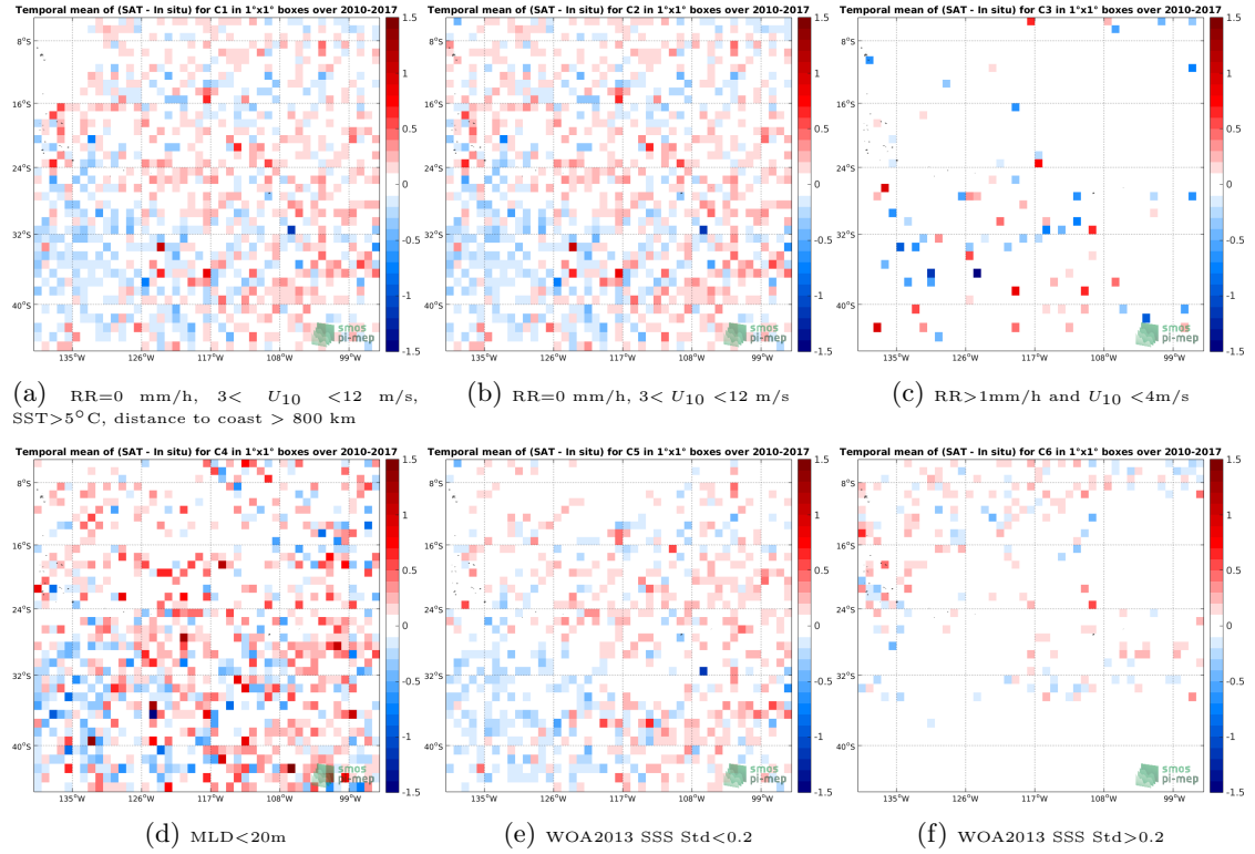
Figure 12: Temporal mean gridded over spatial boxes of size 1^\circ \times 1^\circ of \Delta SSS (SMOS SSS L3 v2 - Daily - 0.5 Deg (CATDS-CECOS-IFREMER) - Argo) for 6 different subdatasets corresponding to: RR=0 mm/h, 3 < U_{10} < 12 m/s, SST > 5^\circ C , distance to coast > 800 km (a), RR=0 mm/h, 3 < U_{10} < 12 m/s (b), RR > 1 mm/h and U_{10} < 4 m/s (c), MLD < 20 m (d), WOA2013 SSS Std < 0.2 (e), WOA2013 SSS Std > 0.2 (f).
