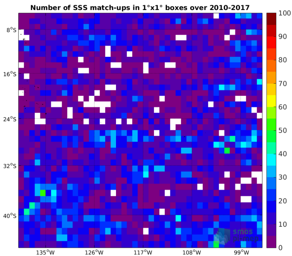
Figure 4: Number of SSS match-ups between Argo SSS and the SMOS L3 v2 - Daily - 0.5 Deg (CATDS-CECOS-IFREMER) SSS product for the OTT zone Pi-MEP region over 1°x1° boxes and for the full satellite product period.
