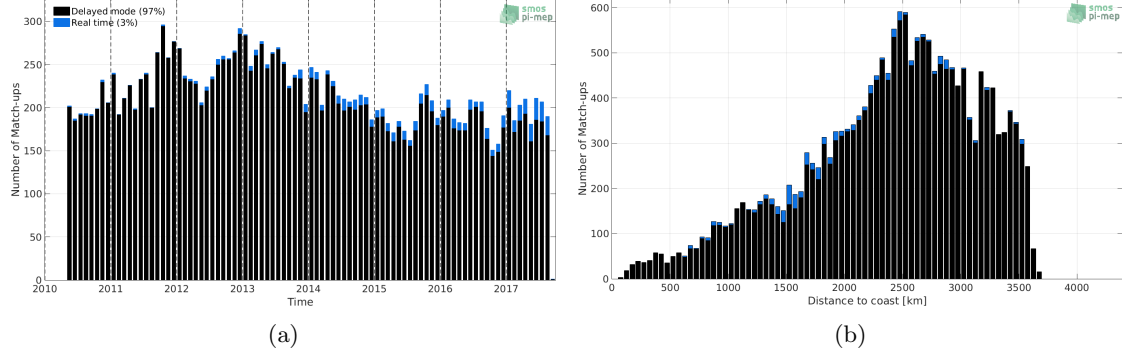
Figure 1: Number of match-ups between Argo and SMOS L3 v2 - Daily - 0.5 Deg (CATDS-CECOS-IFREMER) SSS as a function of time (a) and as function of the distance to coast (b) over the OTT zone Pi-MEP region and for the full satellite product period.
