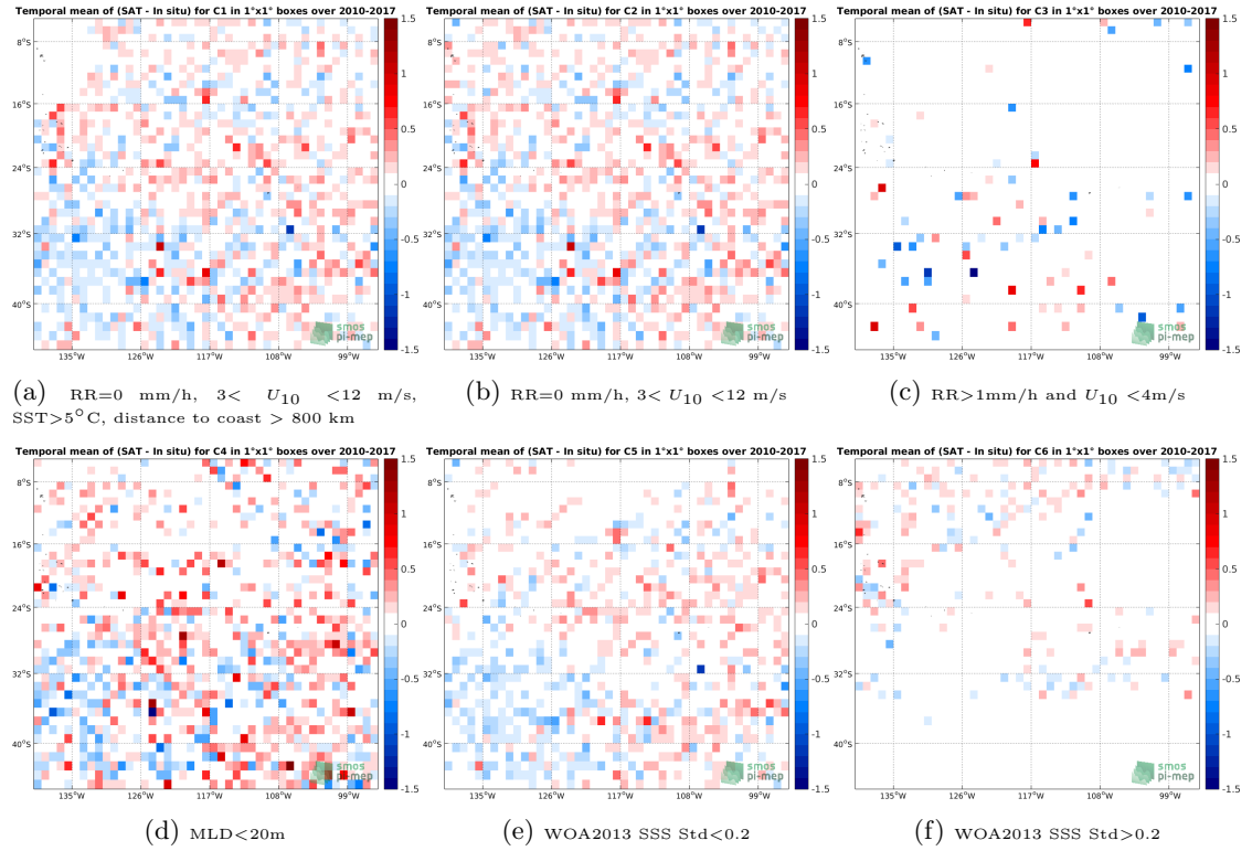
Figure 12: Temporal mean gridded over spatial boxes of size 1^\circ \times 1^\circ of \Delta SSS (SMOS L3 v2 - Daily - 0.5 Deg (CATDS-CECOS-IFREMER) - Argo) for 6 different subdatasets corresponding to: RR=0 mm/h, 3 < U_{10} < 12 m/s, SST >5^\circ C, distance to coast > 800 km (a), RR=0 mm/h, 3 < U_{10} < 12 m/s (b), RR >1 mm/h and U_{10} < 4 m/s (c), MLD <20 m (d), WOA2013 SSS Std <0.2 (e), WOA2013 SSS Std >0.2 (f).
