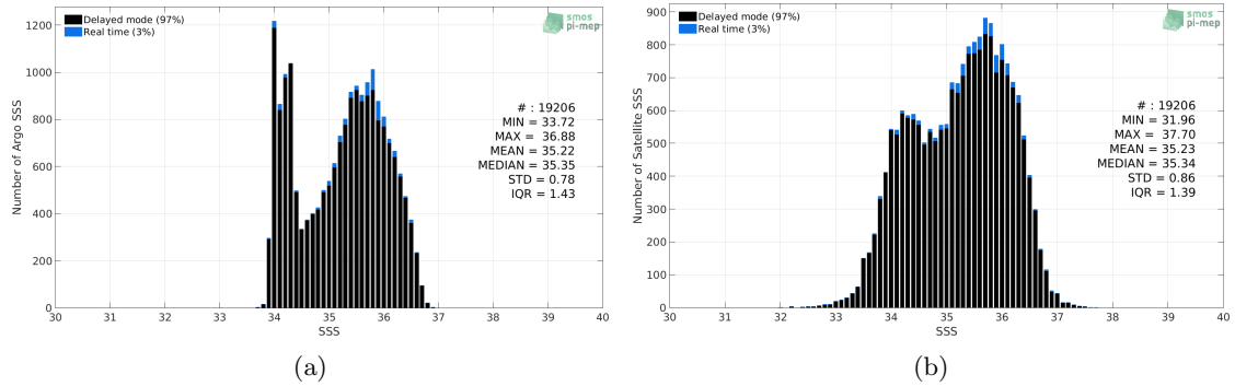
Figure 2: Histograms of SSS from Argo (a) and SMOS L3 v2 - Daily - 0.5 Deg (CATDS-CECOS-IFREMER) (b) considering all match-up pairs per bins of 0.1 over the OTT zone Pi-MEP region and for the full satellite product period.
