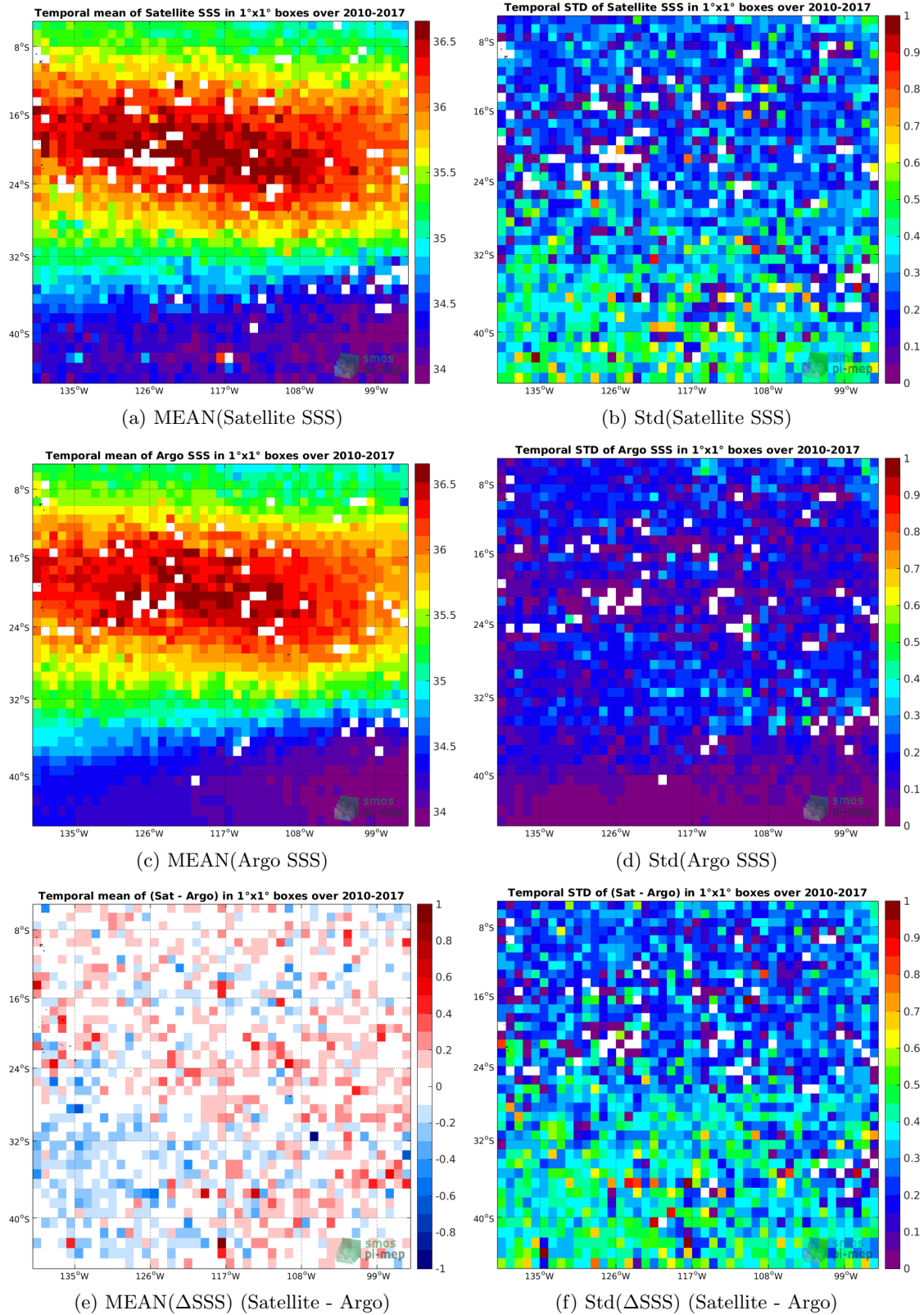
Figure 6: Temporal mean (left) and Std (right) of SSS from SMOS L3 v2 - Daily - 0.5 Deg (CATDS-CECOS-IFREMER) (top), Argo (middle), and of \Delta SSS (Satellite - Argo). Only match-up pairs are used to generate these maps.
