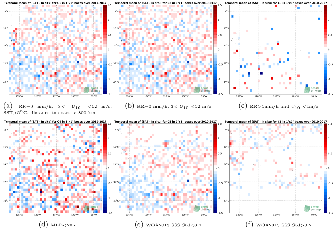
Figure 12: Temporal mean gridded over spatial boxes of size 1^\circ \times 1^\circ of \Delta SSS (SMOS-L3-CATDS-CECOS-IFREMER-V2-1DAY-0.5DEG - Argo) for 6 different subdatasets corresponding to: RR=0 mm/h, 3 < U_{10} < 12 m/s, SST >5^\circ C, distance to coast > 800 km (a), RR=0 mm/h, 3 < U_{10} < 12 m/s (b), RR >1 mm/h and U_{10} < 4 m/s (c), MLD <20 m (d), WOA2013 SSS Std <0.2 (e), WOA2013 SSS Std >0.2 (f).
