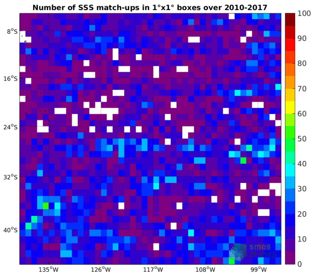
Figure 4: Number of SSS match-ups between Argo SSS and the SMOS-L3-CATDS-CECOS-IFREMER-V2-1DAY-0.5DEG SSS product for the OTT zone Pi-MEP region over 1°x1° boxes and for the full satellite product period.
