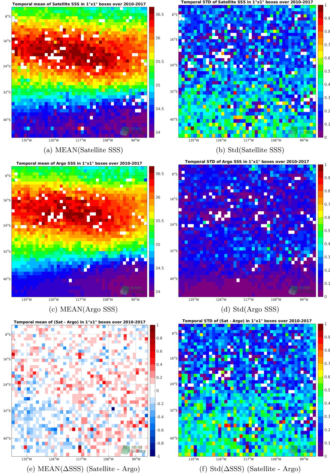
Figure 6: Temporal mean (left) and Std (right) of SSS from SMOS-L3-CATDS-CECOS-IFREMER-V2-1DAY-0.5DEG (top), Argo (middle), and of \Delta SSS (Satellite - Argo). Only match-up pairs are used to generate these maps.
