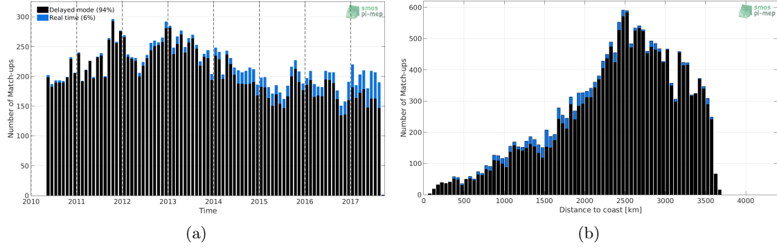
Figure 1: Number of match-ups between Argo and SMOS-L3-CATDS-CECOS-IFREMER-V2-1DAY-0.5DEG SSS as a function of time (a) and as function of the distance to coast (b) over the OTT zone Pi-MEP region and for the full satellite product period.
