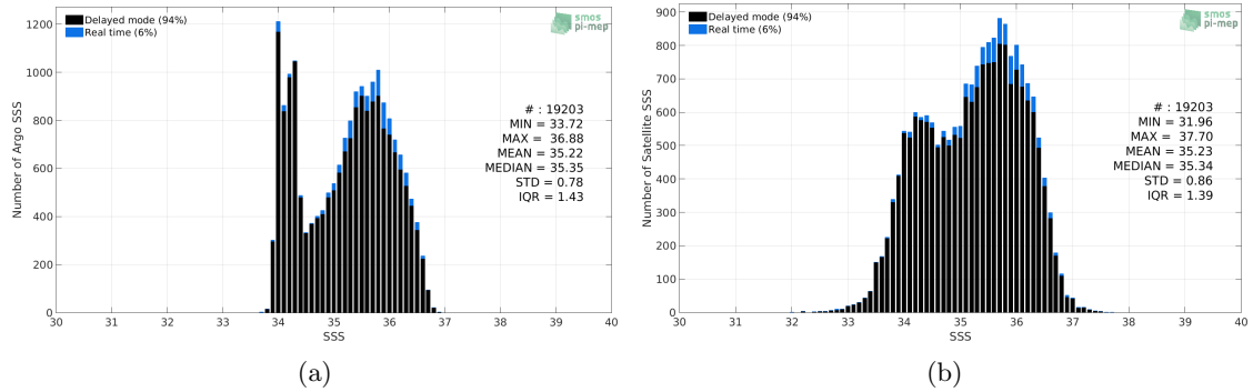
Figure 2: Histograms of SSS from Argo (a) and SMOS-L3-CATDS-CECOS-IFREMER-V2-1DAY-0.5DEG (b) considering all match-up pairs per bins of 0.1 over the OTT zone Pi-MEP region and for the full satellite product period.
