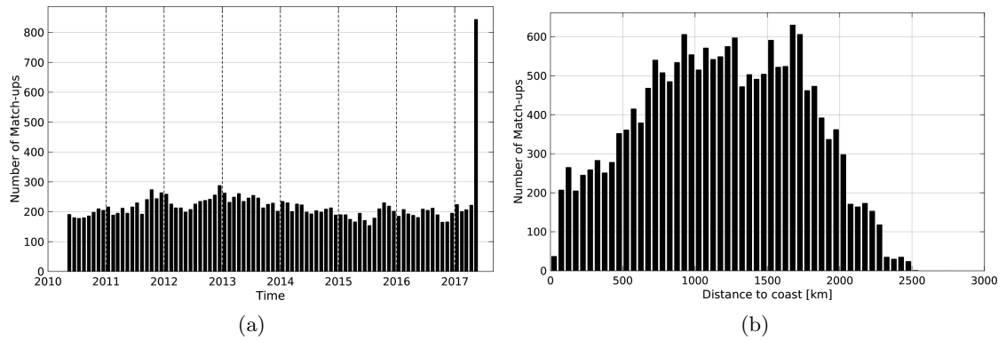
Figure 1: Number of match-ups between Argo and SMOS-L3-CATDS-CECOS-IFREMER-V2-1DAY-0.5deg SSS as a function of time (a) and as function of the distance to coast (b) over the OTT zone Pi-MEP region and for the full satellite product period.
