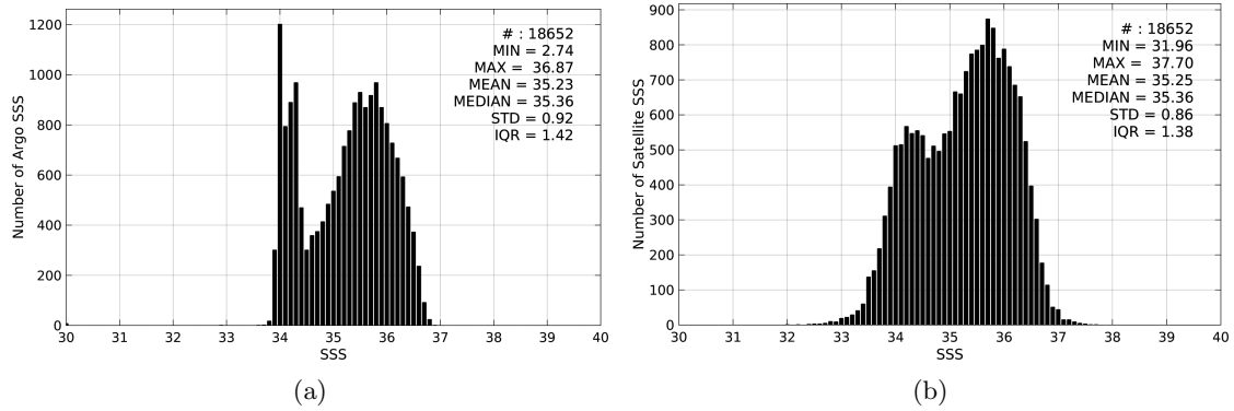
Figure 2: Histograms of SSS from Argo (a) and SMOS-L3-CATDS-CECOS-IFREMER-V2-1DAY-0.5deg (b) considering all match-up pairs per bins of 0.1 over the OTT zone Pi-MEP region and for the full satellite product period.
