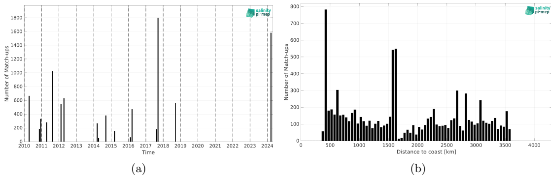
Figure 2: Number of match-ups between TSG (SAMOS) and SMOS SSS L3 v335 - Monthly - 25 km (CATDS-CPDC) SSS as a function of time (a) and as function of the distance to coast (b) over the OTT zone Pi-MEP region and for the full satellite product period.
