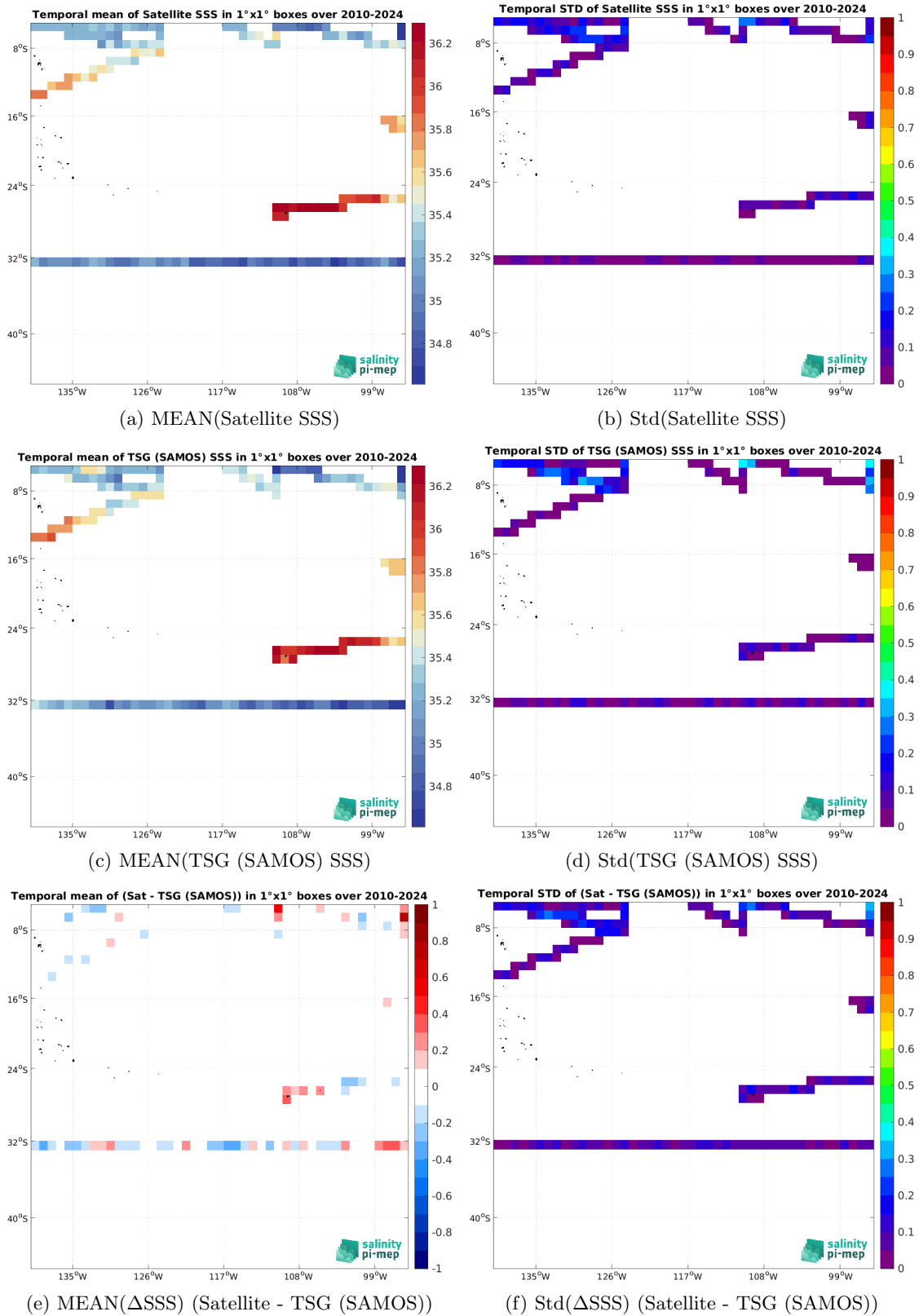
Figure 7: Temporal mean (left) and Std (right) of SSS from SMOS SSS L3 v335 - Monthly - 25 km (CATDS-CPDC) (top), TSG (SAMOS) (middle), and of \Delta SSS (Satellite - TSG (SAMOS)). Only match-up pairs are used to generate these maps.
