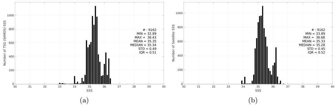
Figure 3: Histograms of SSS from TSG (SAMOS) (a) and SMOS SSS L3 v335 - Monthly - 25 km (CATDS-CPDC) (b) considering all match-up pairs per bins of 0.1 over the OTT zone Pi-MEP region and for the full satellite product period.
