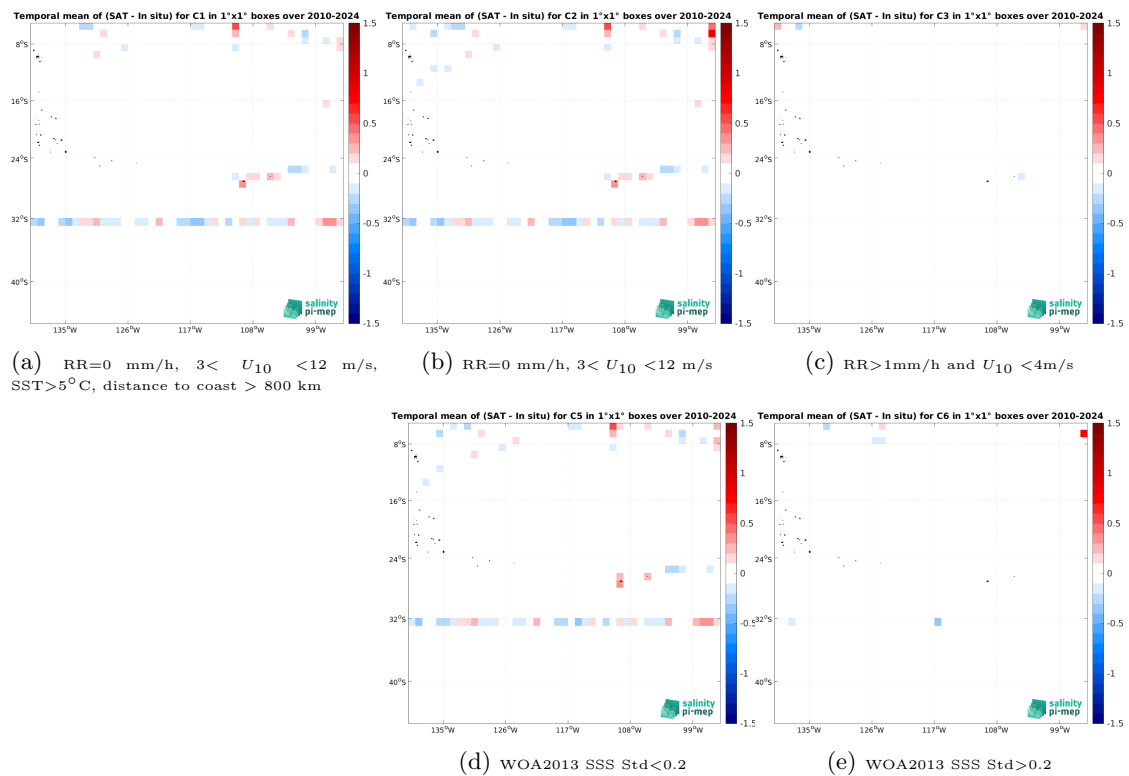
Figure 14: Temporal mean gridded over spatial boxes of size 1^\circ \times 1^\circ of \Delta SSS (SMOS SSS L3 v335 - Monthly - 25 km (CATDS-CPDC) - TSG (SAMOS)) for 5 different subdatasets corresponding to: RR=0 mm/h, 3 < U_{10} < 12 m/s, SST > 5^\circ C , distance to coast > 800 km (a), RR=0 mm/h, 3 < U_{10} < 12 m/s (b), RR > 1 mm/h and U_{10} < 4 m/s (c), WOA2013 SSS Std < 0.2 (d), WOA2013 SSS Std > 0.2 (e).
