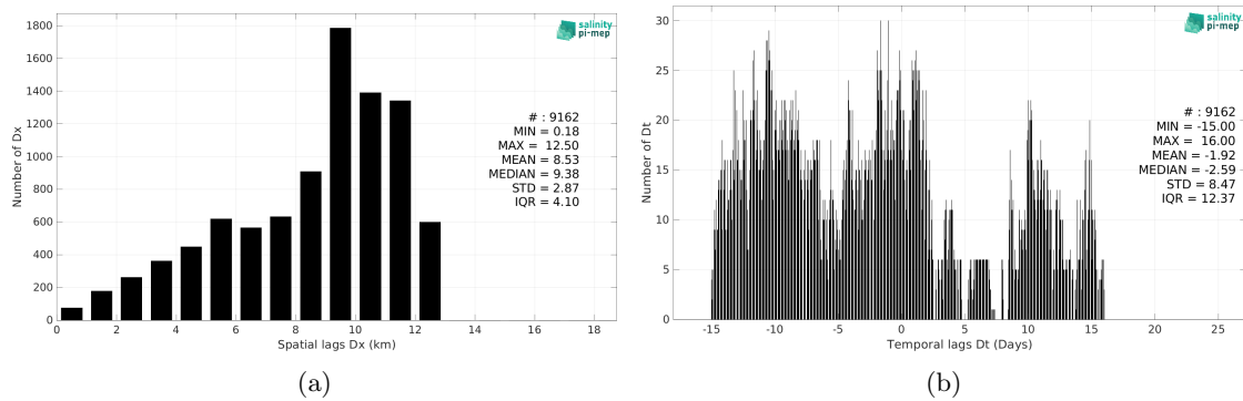
Figure 6: Histograms of the spatial (a) and temporal (b) lags between the location/time of the TSG (SAMOS) measurement and the date of the corresponding SMOS SSS L3 v335 - Monthly - 25 km (CATDS-CPDC) SSS pixel.
