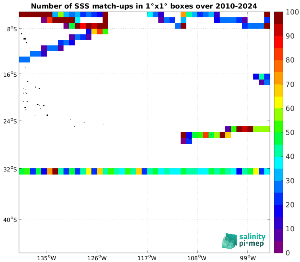
Figure 5: Number of SSS match-ups between TSG (SAMOS) SSS and the SMOS SSS L3 v335 - Monthly - 25 km (CATDS-CPDC) SSS product for the OTT zone Pi-MEP region over 1^\circ \times 1^\circ boxes and for the full satellite product period.
