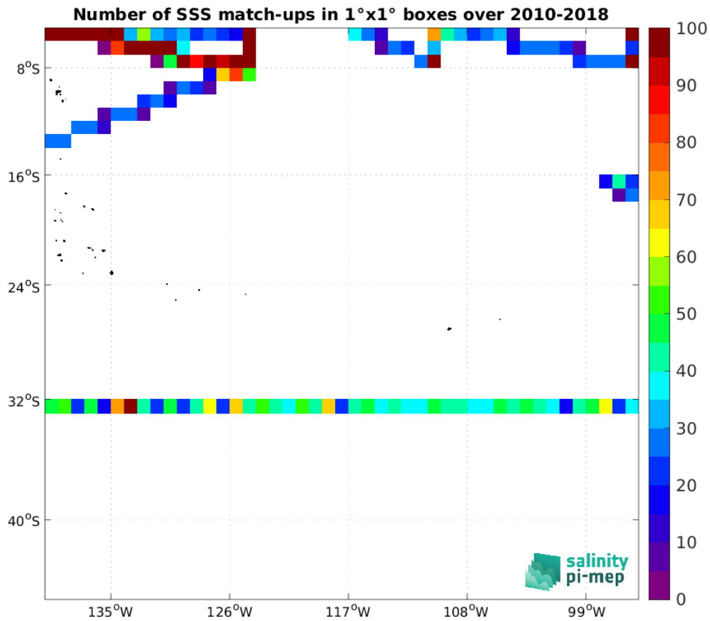
Figure 4: Number of SSS match-ups between TSG (SAMOS) SSS and the SMOS SSS L3 v335 - Monthly - 25 km (CATDS-CPDC) SSS product for the OTT zone Pi-MEP region over 1^{\circ} \times 1^{\circ} boxes and for the full satellite product period.
