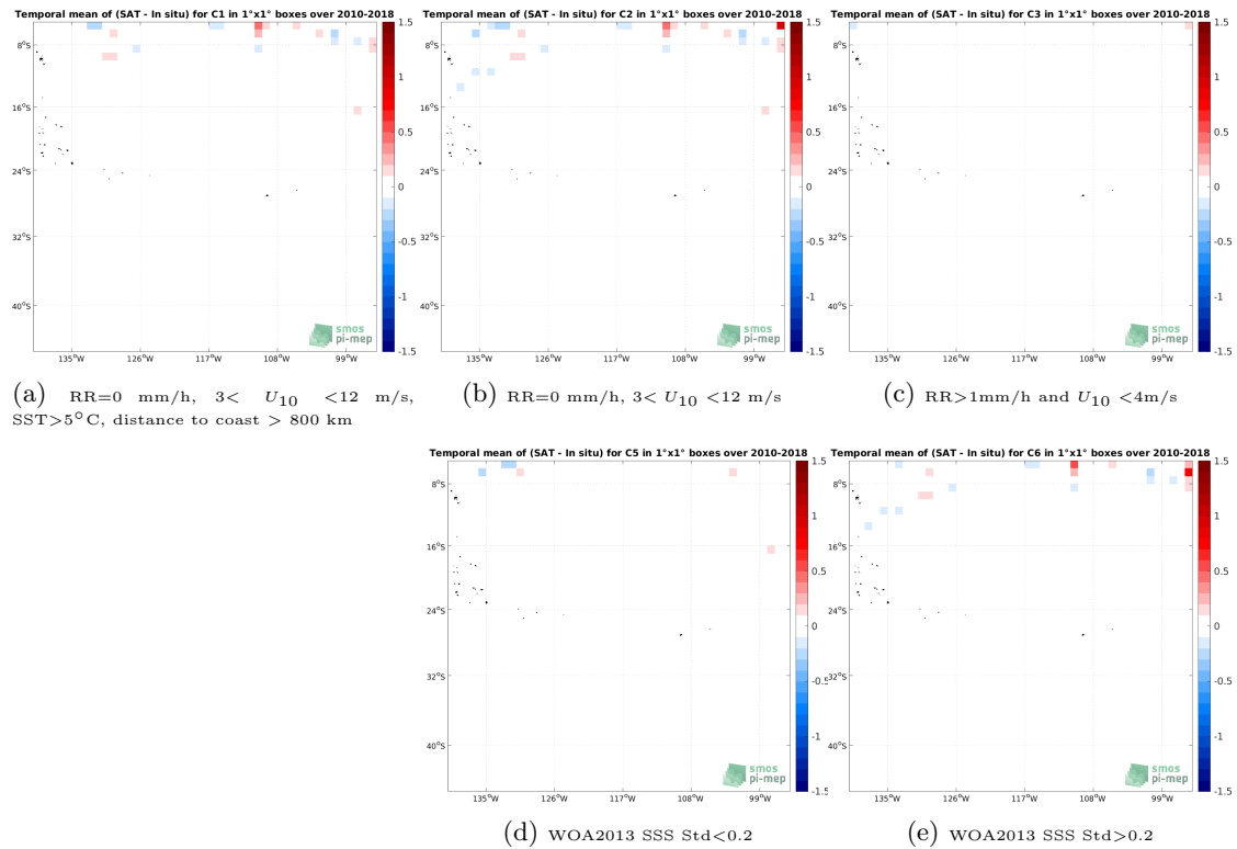
Figure 12: Temporal mean gridded over spatial boxes of size 1^\circ \times 1^\circ of \Delta SSS (SMOS SSS L3 v335 - Monthly - 25 km (CATDS-CPDC) - TSG (SAMOS)) for 5 different subdatasets corresponding to:RR=0 mm/h, 3 < U_{10} < 12 m/s, SST >5^\circ C, distance to coast > 800 km (a), RR=0 mm/h, 3 < U_{10} < 12 m/s (b), RR >1 mm/h and U_{10} < 4 m/s (c), WOA2013 SSS Std <0.2 (d), WOA2013 SSS Std >0.2 (e).
