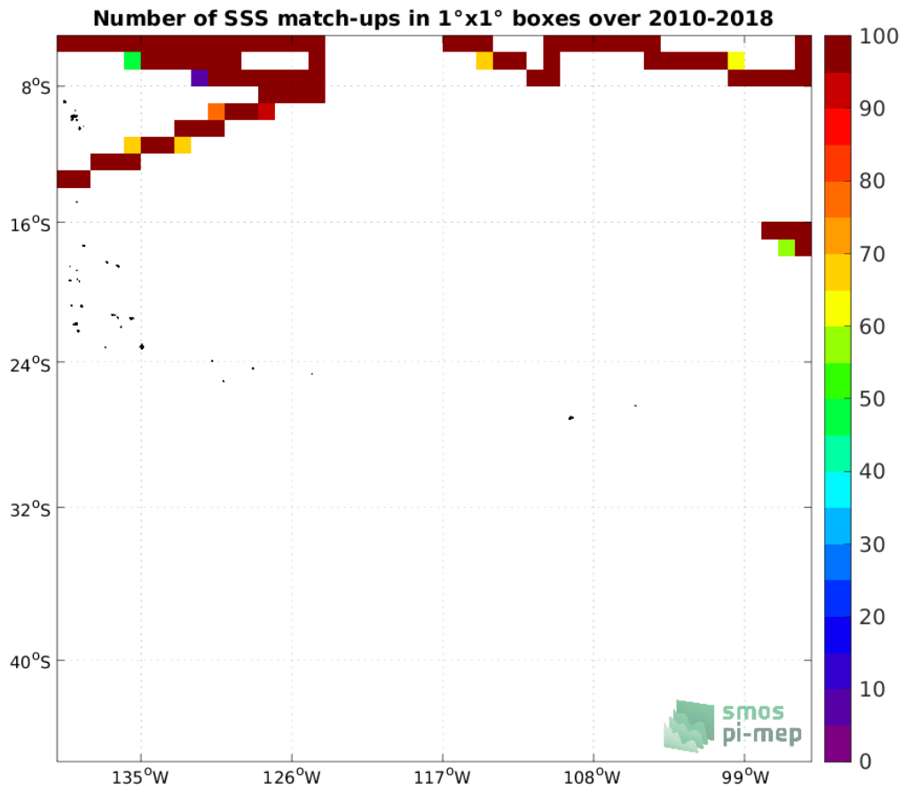
Figure 4: Number of SSS match-ups between TSG (SAMOS) SSS and the SMOS SSS L3 v335 - Monthly - 25 km (CATDS-CPDC) SSS product for the OTT zone Pi-MEP region over 1^\circ \times 1^\circ boxes and for the full satellite product period.
