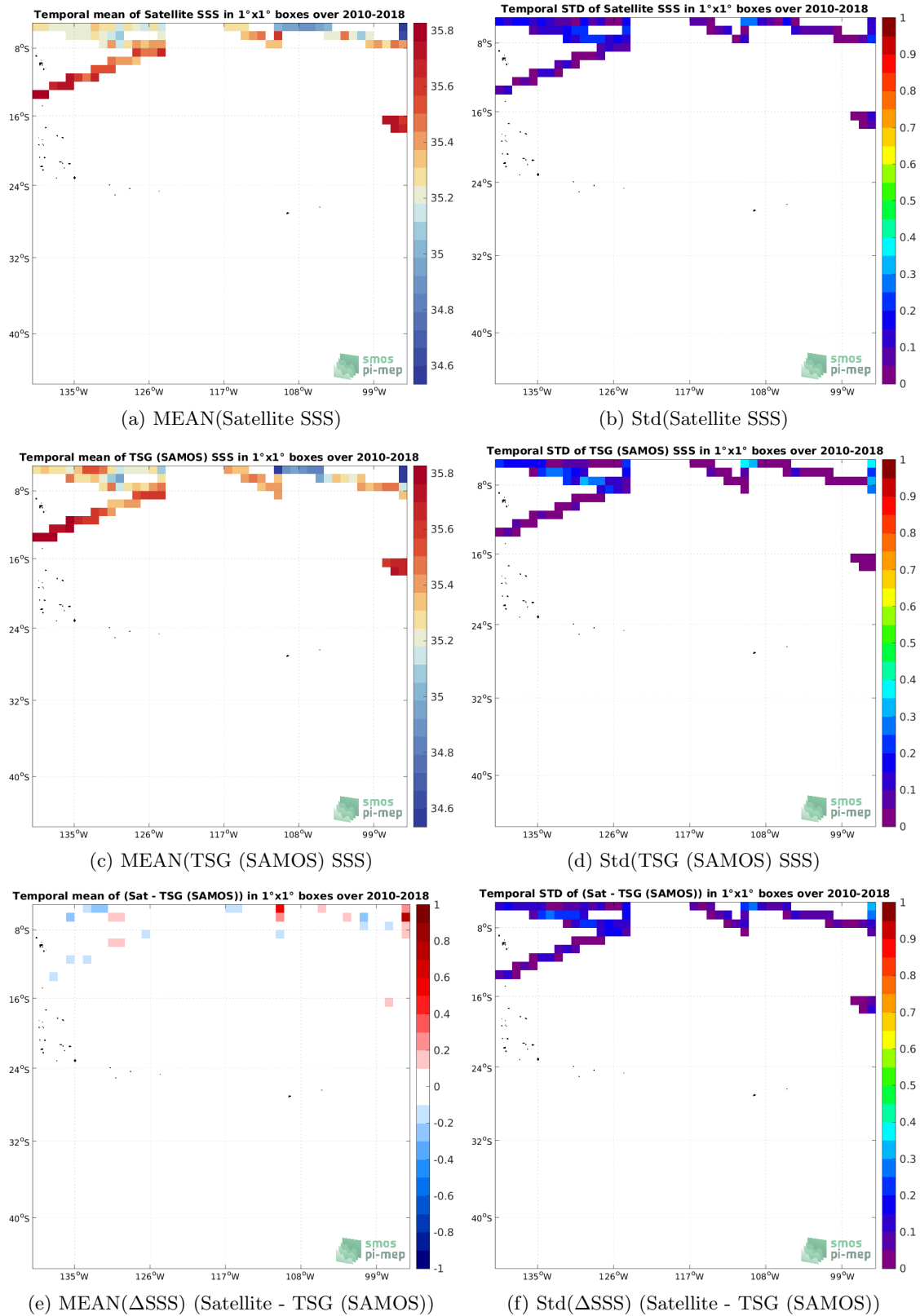
Figure 6: Temporal mean (left) and Std (right) of SSS from SMOS SSS L3 v335 - Monthly - 25 km (CATDS-CPDC) (top), TSG (SAMOS) (middle), and of \Delta SSS (Satellite - TSG (SAMOS)). Only match-up pairs are used to generate these maps.
