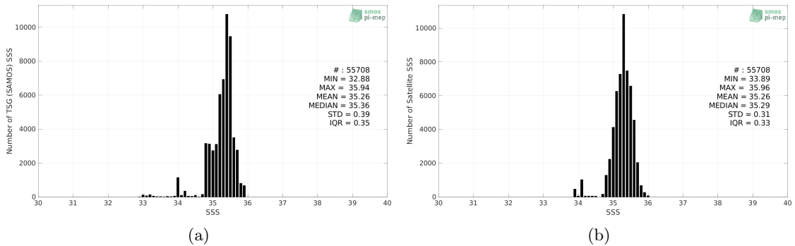
Figure 2: Histograms of SSS from TSG (SAMOS) (a) and SMOS SSS L3 v335 - Monthly - 25 km (CATDS-CPDC) (b) considering all match-up pairs per bins of 0.1 over the OTT zone Pi-MEP region and for the full satellite product period.
