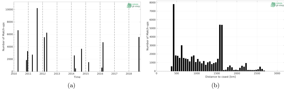
Figure 1: Number of match-ups between TSG (SAMOS) and SMOS SSS L3 v335 - Monthly - 25 km (CATDS-CPDC) SSS as a function of time (a) and as function of the distance to coast (b) over the OTT zone Pi-MEP region and for the full satellite product period.
