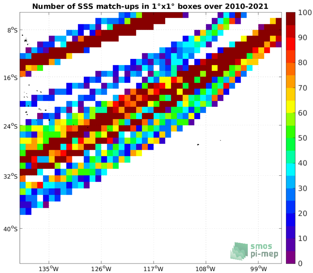
Figure 4: Number of SSS match-ups between TSG (LEGOS-DM) SSS and the SMOS SSS L3 v335 - Monthly - 25 km (CATDS-CPDC) SSS product for the OTT zone Pi-MEP region over 1°x1° boxes and for the full satellite product period.
