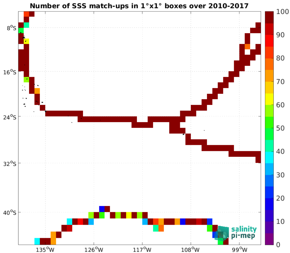
Figure 4: Number of SSS match-ups between TSG (GOSUD-Sailing-ship) SSS and the SMOS SSS L3 v335 - Monthly - 25 km (CATDS-CPDC) SSS product for the OTT zone Pi-MEP region over 1^{\circ} \times 1^{\circ} boxes and for the full satellite product period.
