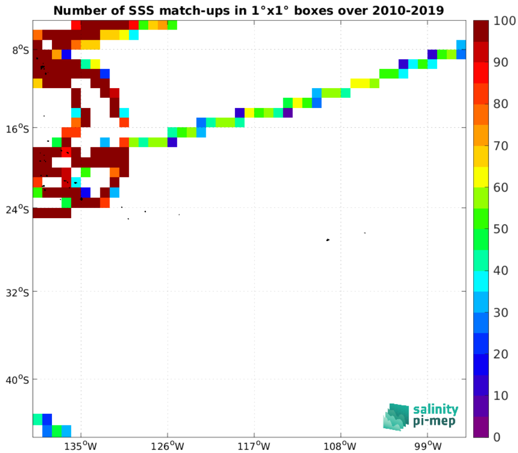
Figure 5: Number of SSS match-ups between TSG (GOSUD-Research-vessel) SSS and the SMOS SSS L3 v335 - Monthly - 25 km (CATDS-CPDC) SSS product for the OTT zone Pi-MEP region over 1^\circ \times 1^\circ boxes and for the full satellite product period.
