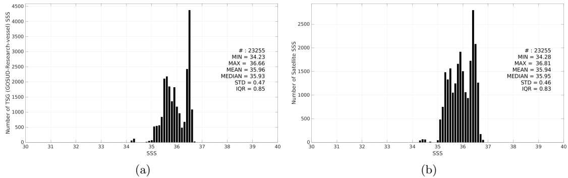
Figure 3: Histograms of SSS from TSG (GOSUD-Research-vessel) (a) and SMOS SSS L3 v335 - Monthly - 25 km (CATDS-CPDC) (b) considering all match-up pairs per bins of 0.1 over the OTT zone Pi-MEP region and for the full satellite product period.
