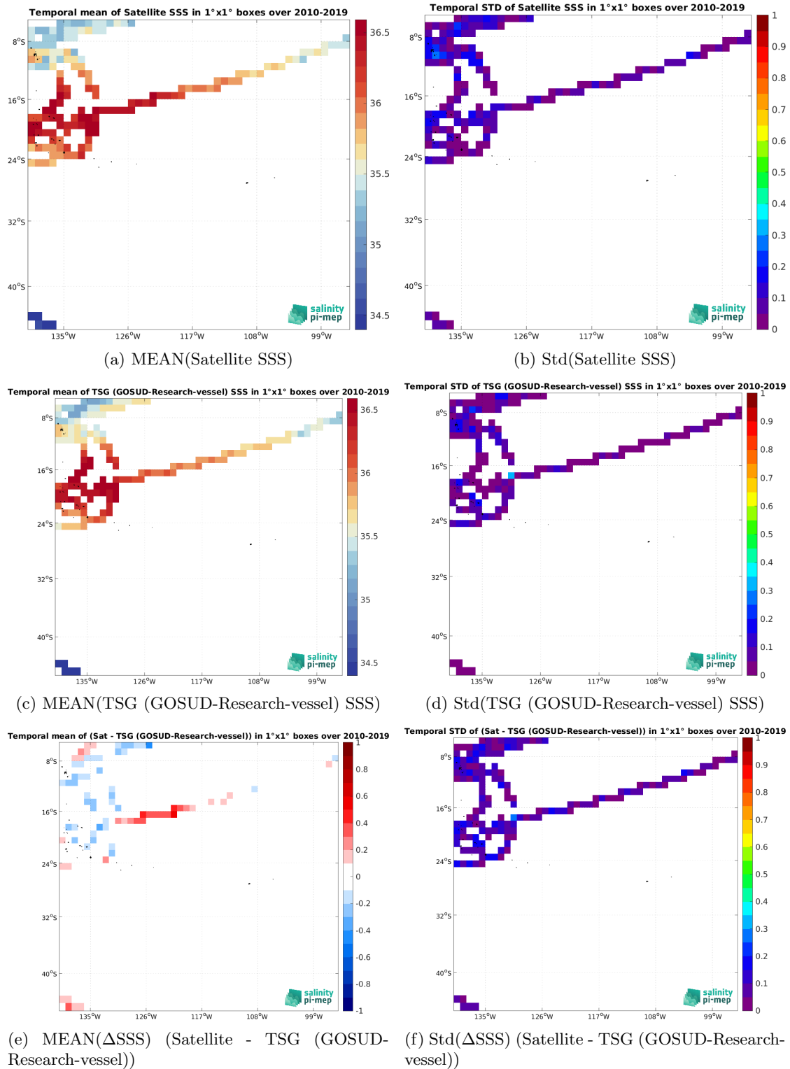
Figure 7: Temporal mean (left) and Std (right) of SSS from SMOS SSS L3 v335 - Monthly - 25 km (CATDS-CPDC) (top), TSG (GOSUD-Research-vessel) (middle), and of \Delta SSS (Satellite - TSG (GOSUD-Research-vessel)). Only match-up pairs are used to generate these maps.
