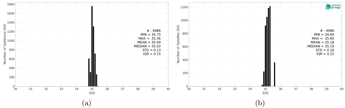
Figure 2: Histograms of SSS from Saildrone (a) and SMOS SSS L3 v335 - Monthly - 25 km (CATDS-CPDC) (b) considering all match-up pairs per bins of 0.1 over the OTT zone Pi-MEP region and for the full satellite product period.
