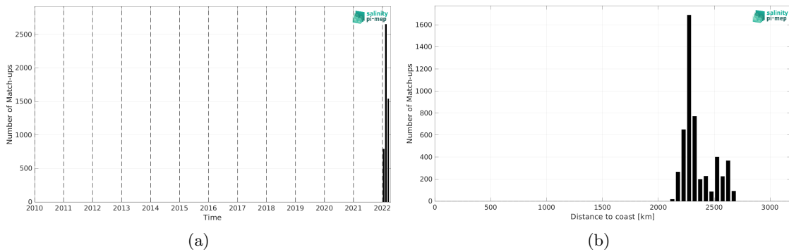
Figure 1: Number of match-ups between Saildrone and SMOS SSS L3 v335 - Monthly - 25 km (CATDS-CPDC) SSS as a function of time (a) and as function of the distance to coast (b) over the OTT zone Pi-MEP region and for the full satellite product period.
