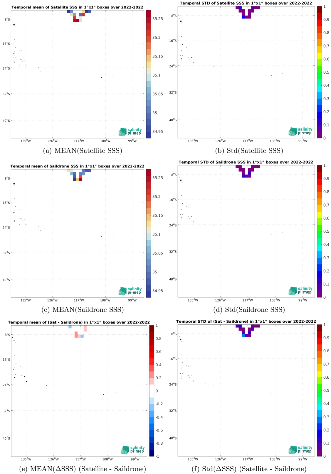
Figure 6: Temporal mean (left) and Std (right) of SSS from SMOS SSS L3 v335 - Monthly - 25 km (CATDS-CPDC) (top), Saildrone (middle), and of \Delta SSS (Satellite - Saildrone). Only match-up pairs are used to generate these maps.
