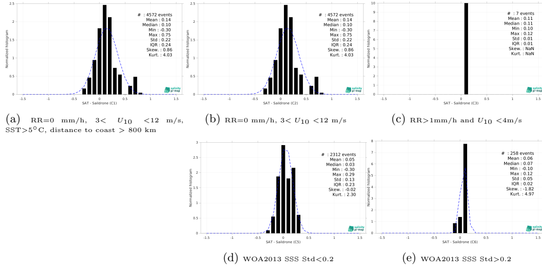
Figure 13: Normalized histogram of \Delta SSS (SMOS SSS L3 v335 - Monthly - 25 km (CATDS-CPDC) - Sairdrone) for 5 different subdatasets corresponding to: RR=0 mm/h, 3 < U_{10} < 12 m/s, SST > 5°C, distance to coast > 800 km (a), RR=0 mm/h, 3 < U_{10} < 12 m/s (b), RR > 1mm/h and U_{10} < 4 m/s (c), WOA2013 SSS Std < 0.2 (d), WOA2013 SSS Std > 0.2 (e).
