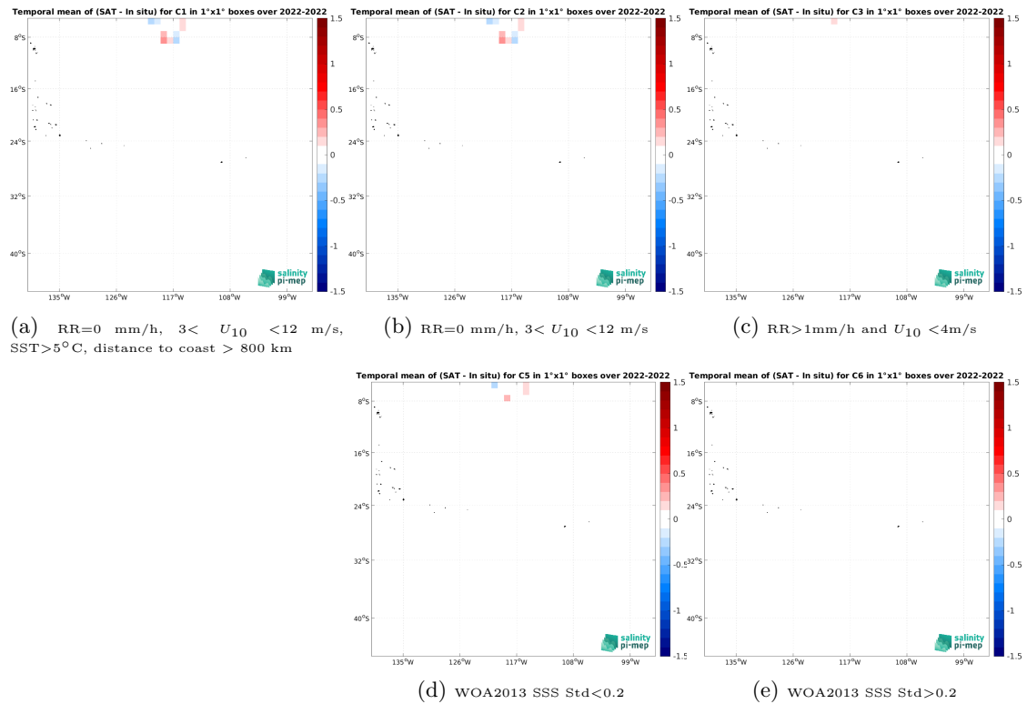
Figure 12: Temporal mean gridded over spatial boxes of size 1^\circ \times 1^\circ of \Delta SSS (SMOS SSS L3 v335 - Monthly - 25 km (CATDS-CPDC) - Saildrone) for 5 different subdatasets corresponding to:RR=0 mm/h, 3 < U_{10} < 12 m/s, SST >5^\circ C, distance to coast > 800 km (a), RR=0 mm/h, 3 < U_{10} < 12 m/s (b), RR >1 mm/h and U_{10} < 4 m/s (c), WOA2013 SSS Std <0.2 (d), WOA2013 SSS Std >0.2 (e).
