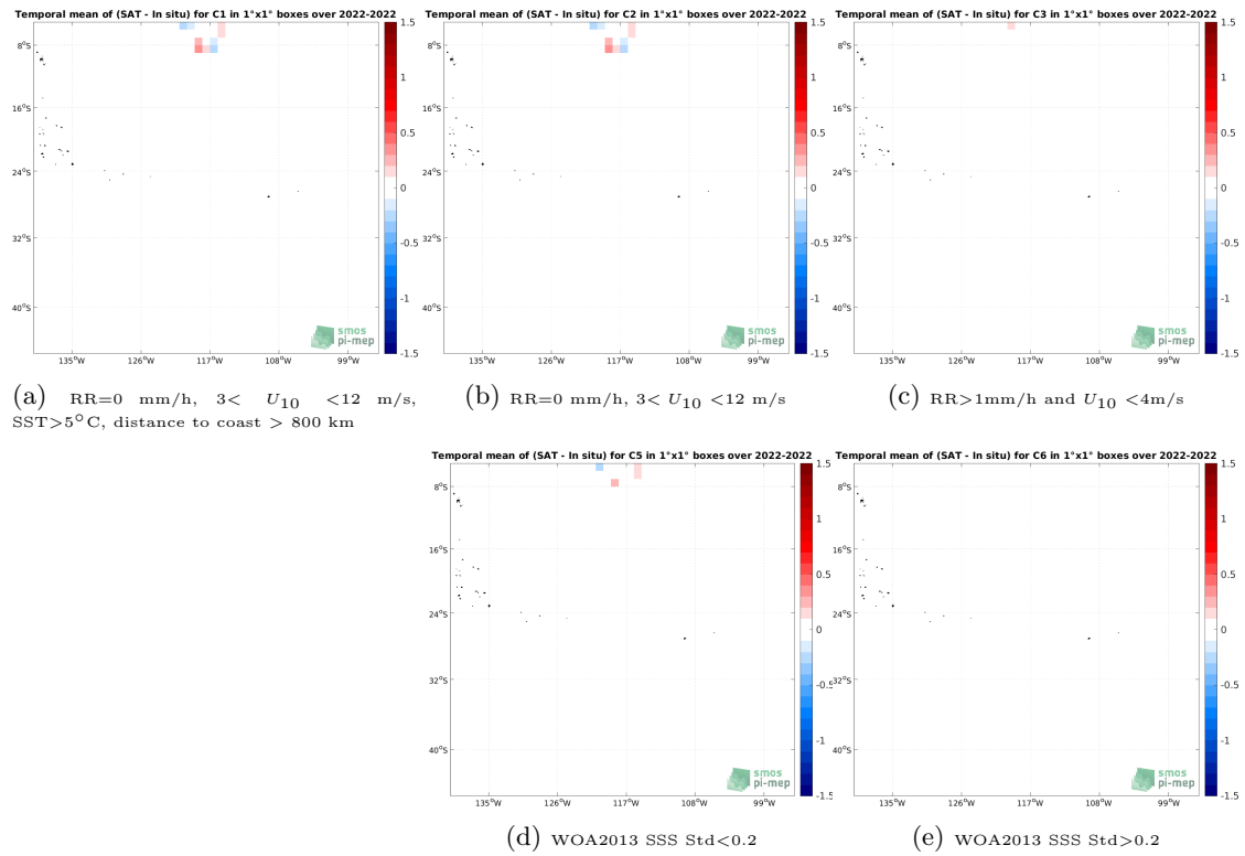
Figure 12: Temporal mean gridded over spatial boxes of size 1^\circ \times 1^\circ of \Delta SSS (SMOS SSS L3 v335 - Monthly - 25 km (CATDS-CPDC) - Saildrone) for 5 different subdatasets corresponding to:RR=0 mm/h, 3 < U_{10} < 12 m/s, SST >5^\circ C, distance to coast > 800 km (a), RR=0 mm/h, 3 < U_{10} < 12 m/s (b), RR >1 mm/h and U_{10} < 4 m/s (c), WOA2013 SSS Std <0.2 (d), WOA2013 SSS Std >0.2 (e).
